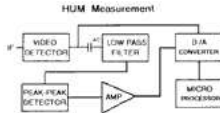
Figure 10: HUM Measurement Block Diagram
