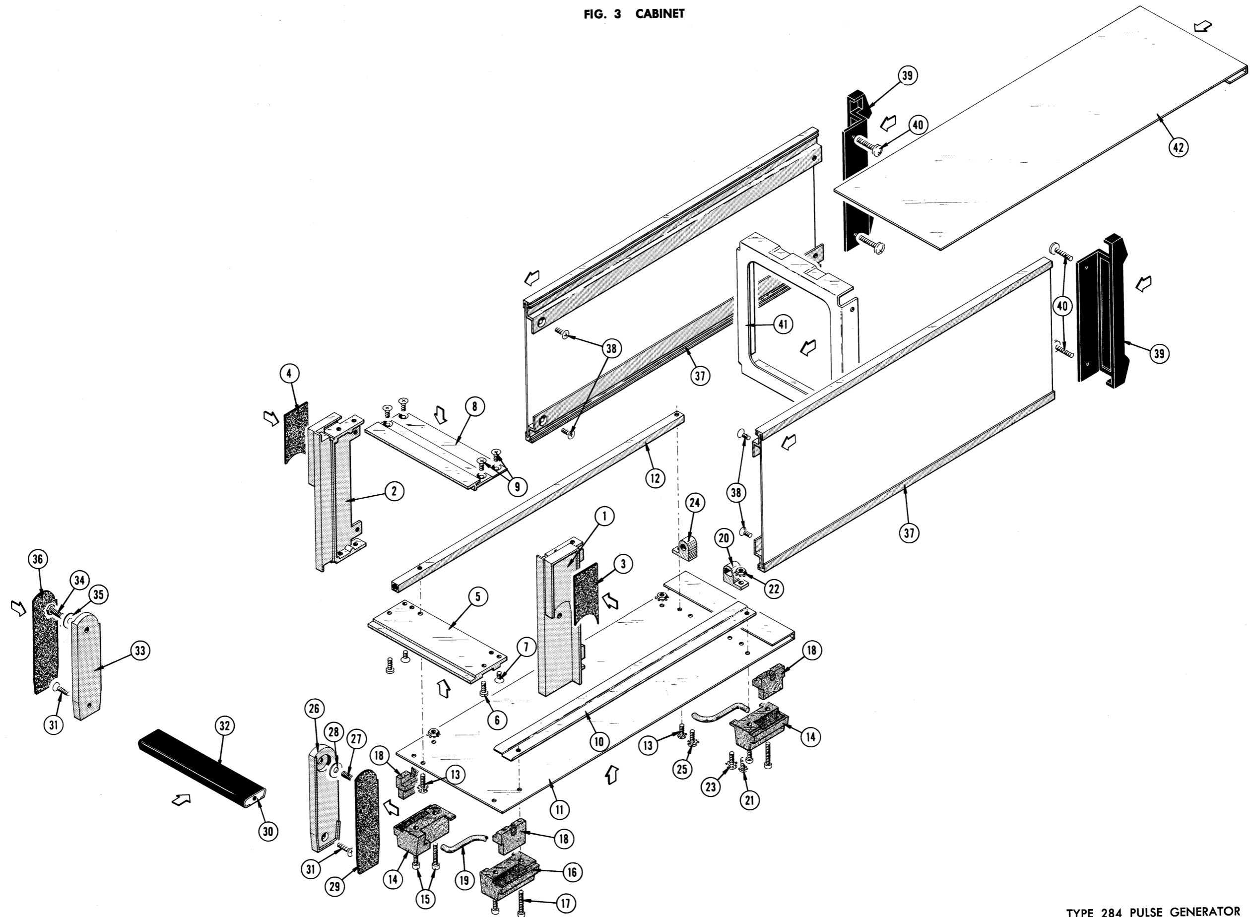
TYPE 284 PULSE GENERATOR
