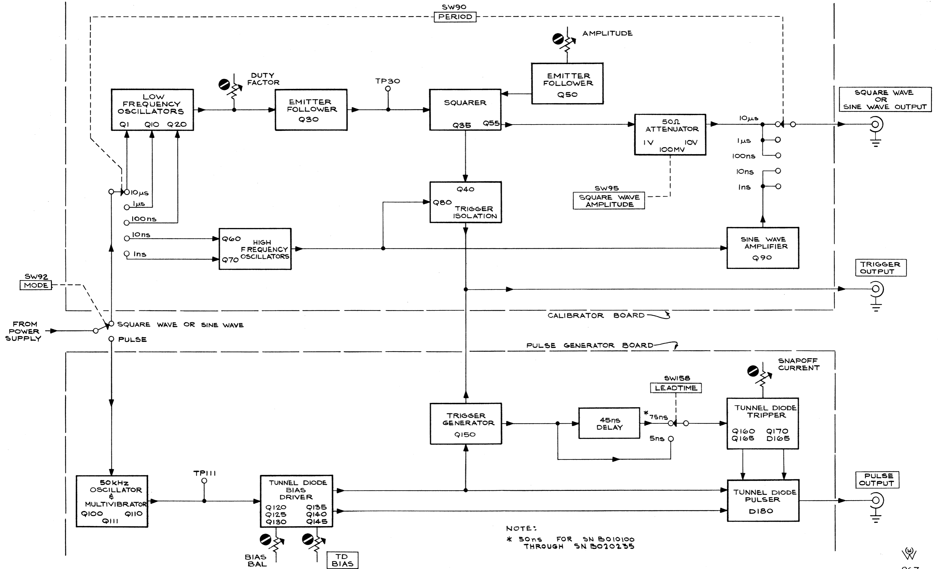
BLOCK DIAGRAM
