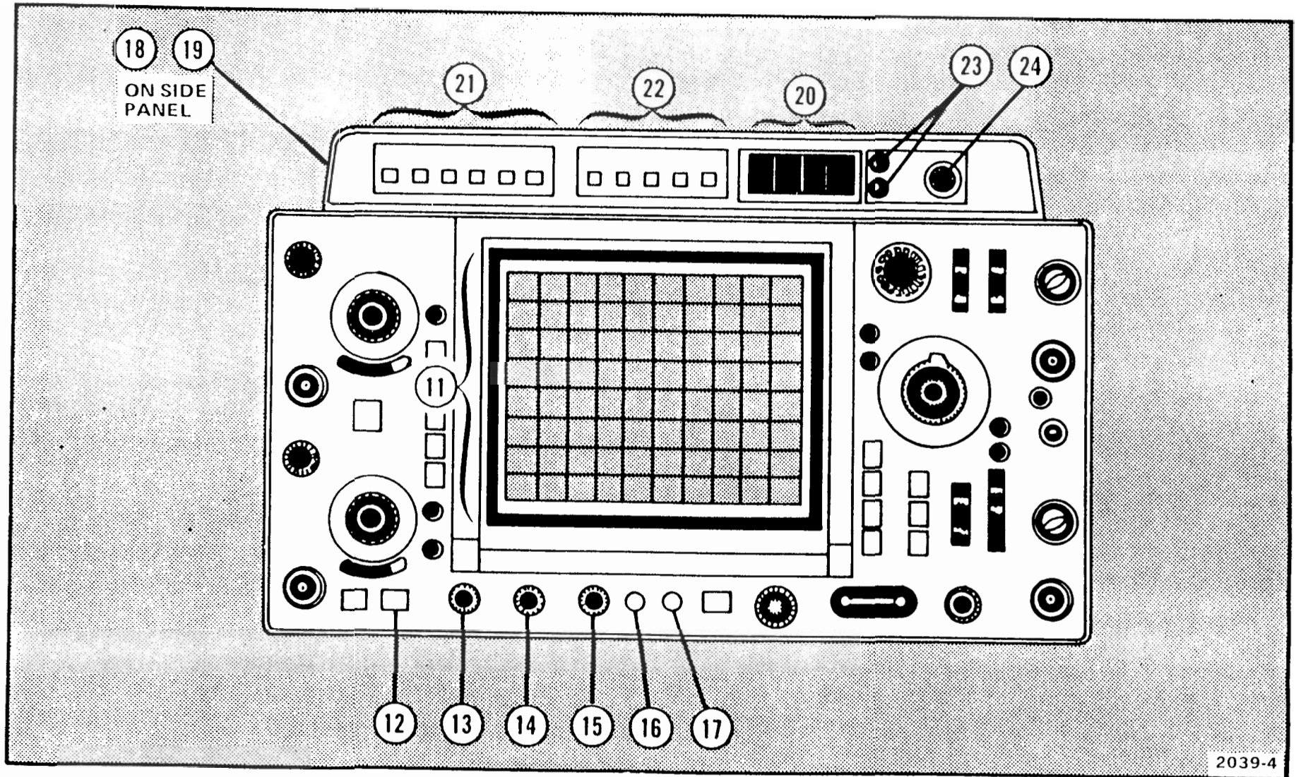
Fig. 3. Display and DM44 controls, connectors, and indicators.
