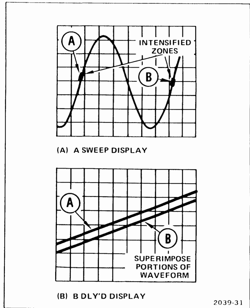
Fig. 30. Time duration and frequency measurements.
