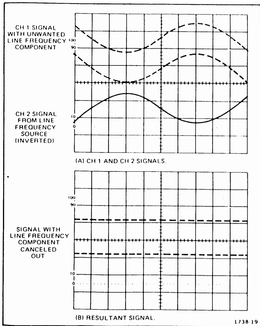
Fig. 17. Common-mode rejection.
