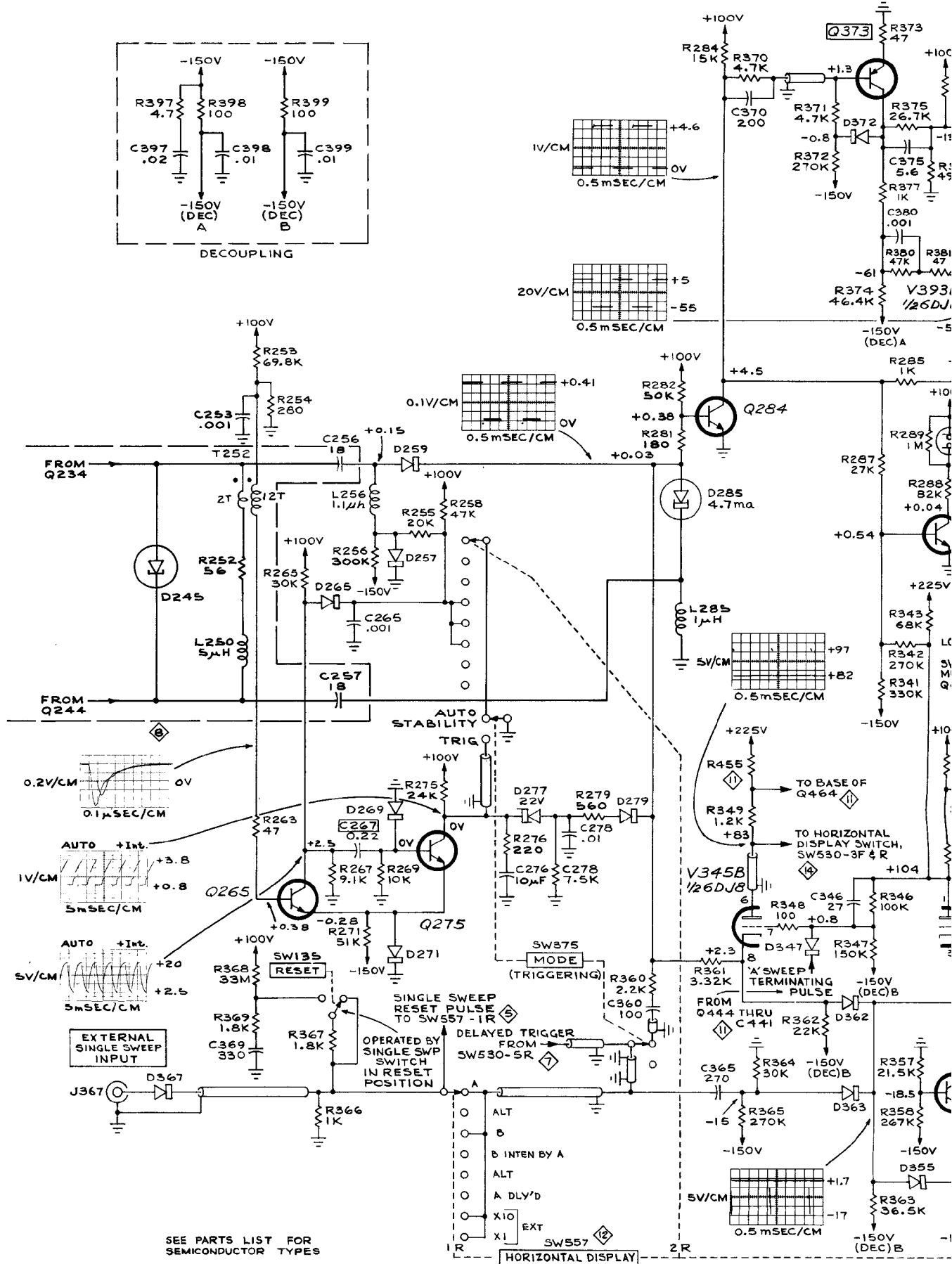
TYPE 547 OSCILLOSCOPE
