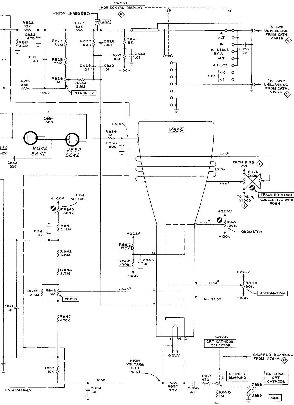
CMP 467 CRT CIRCUIT 2
