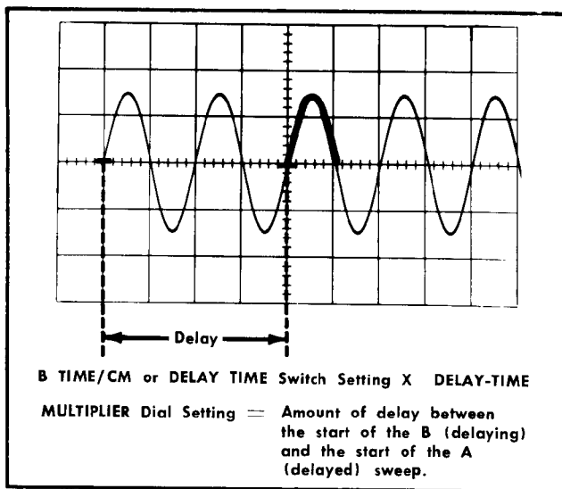
Fig. 2-4. Determining delay time.
