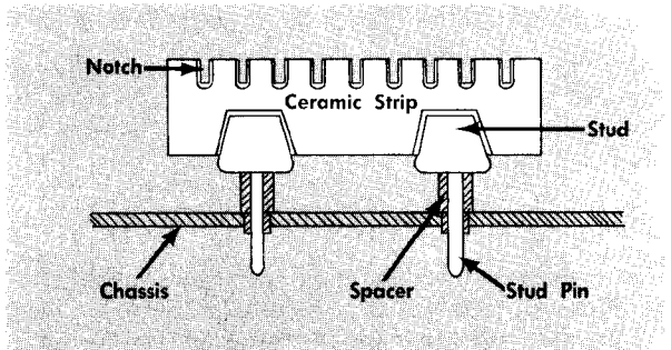
Fig. 4-4. Ceramic strip assembly.
