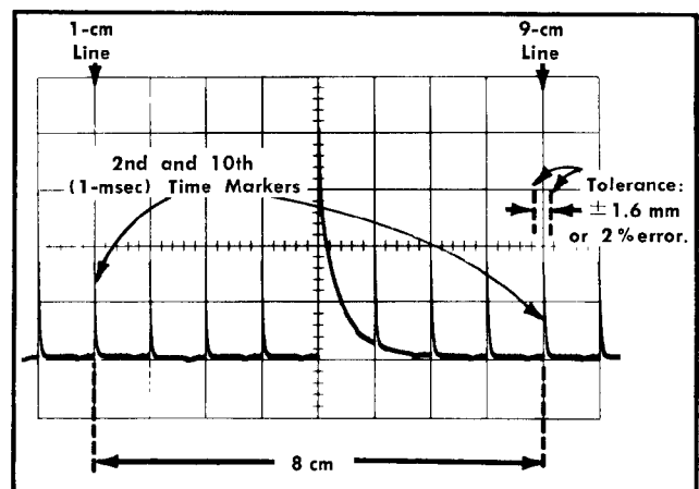
Fig. 5-10. Determining sweep-rate accuracy.
