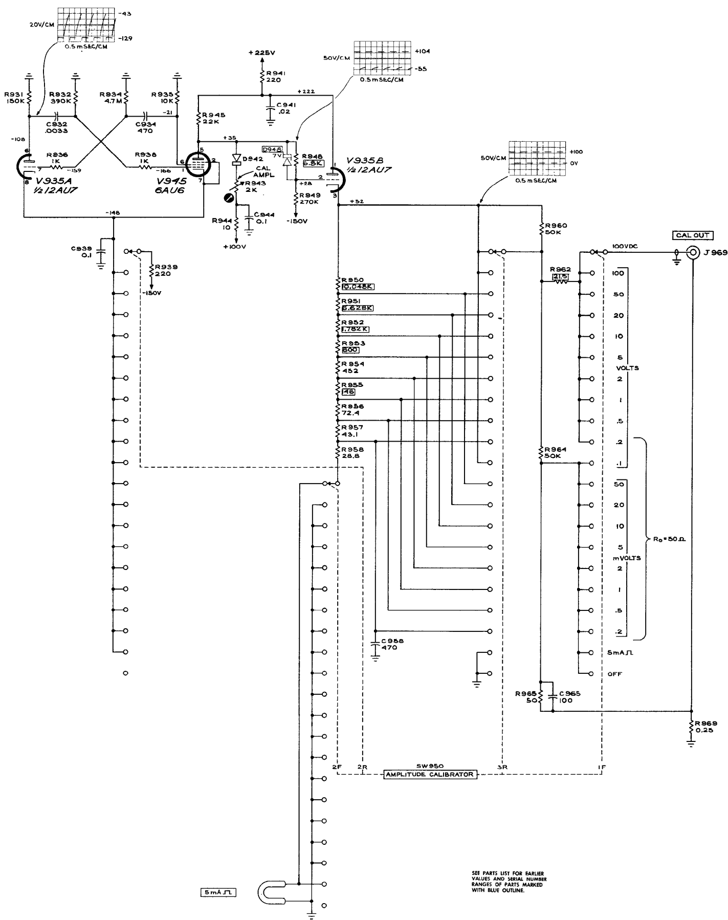
TYPE 547 OSCILLOSCOPE
