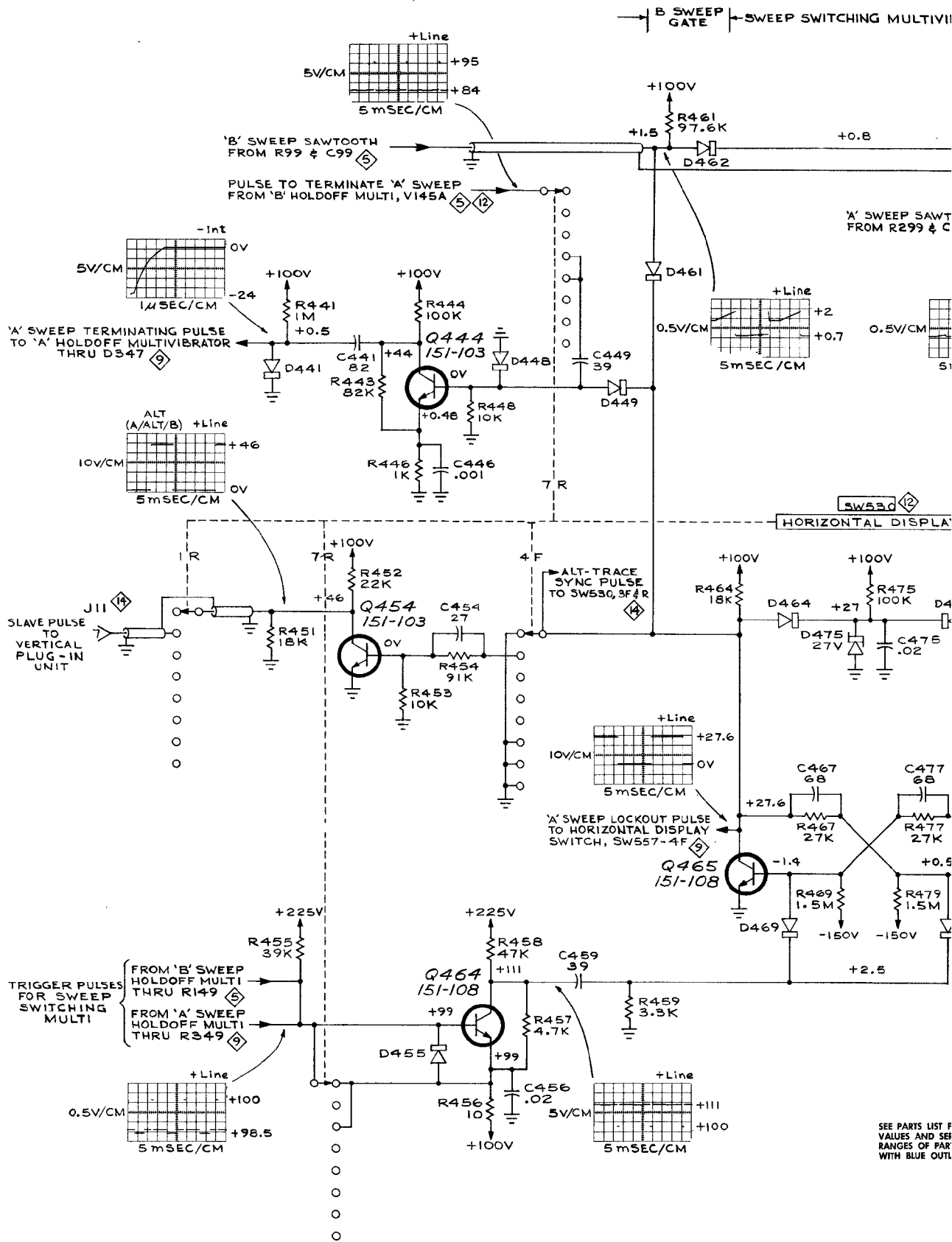
TYPE 547 OSCILLOSCOPE
