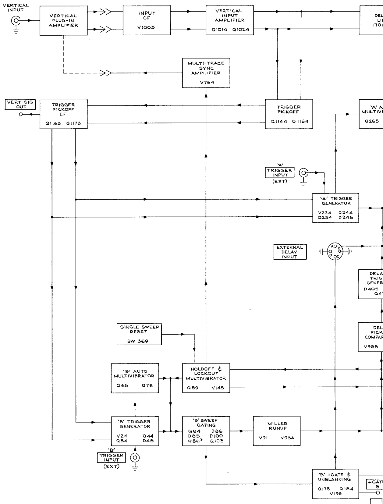
TYPE 547 OSCILLOSCOPE
