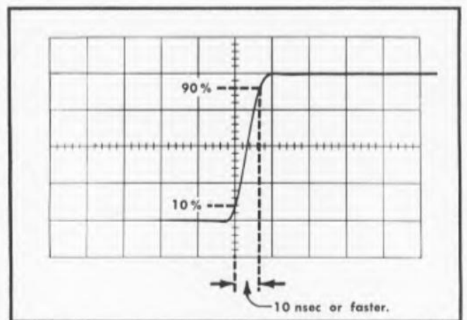
Fig. 5-20. Measuring the risetime of a normal waveform when SW1000 is actuated; sweep rate is 10 \text{ nsec/cm} .
