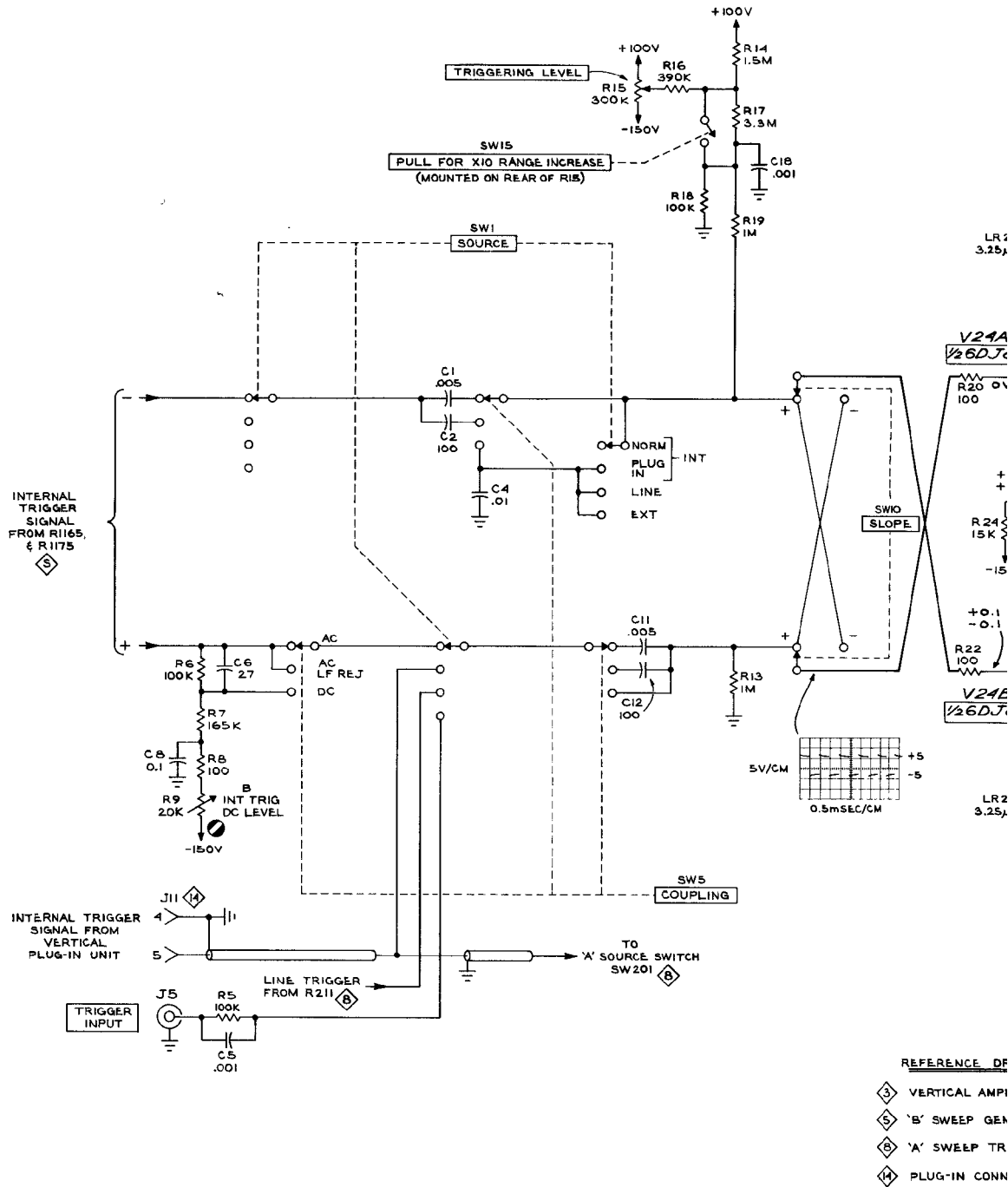
TYPE 547 OSCILLOSCOPE
