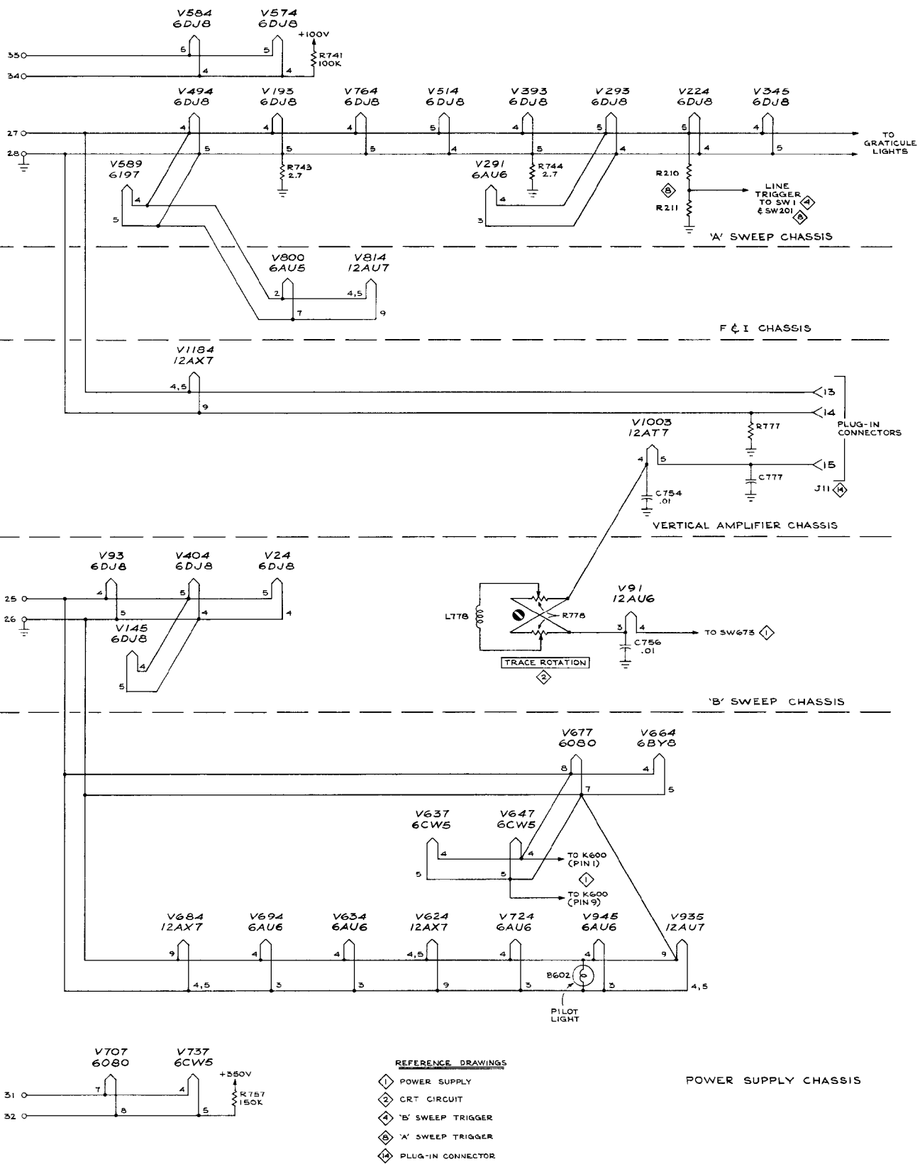
HEATER WIRING DIAGRAM
