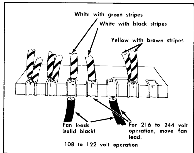
Fig. 2-7. Fan connections for 108 to 244 volt, 50 to 60 cps. SN 7979 and below.
