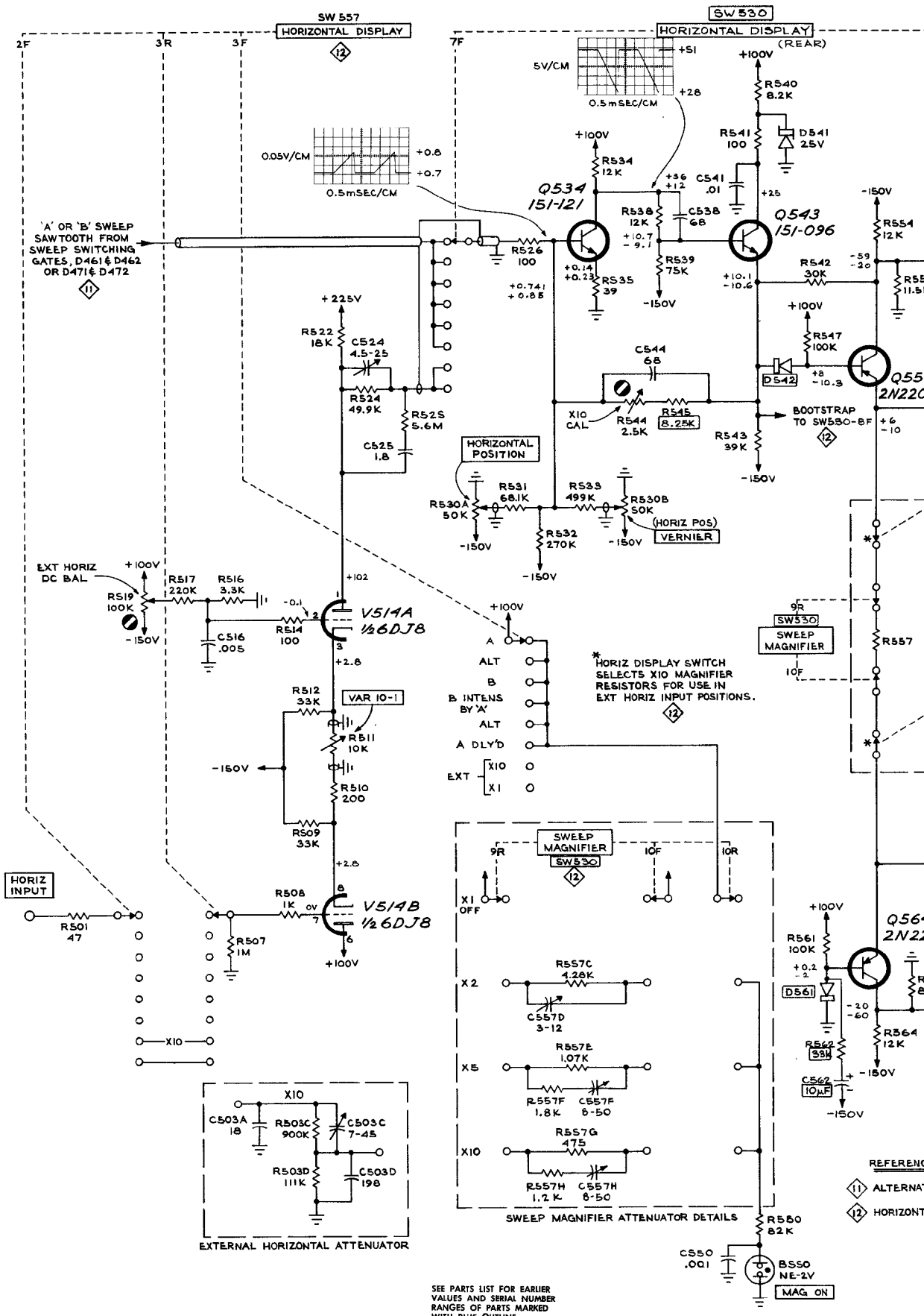
TYPE 547 OSCILLOSCOPE
