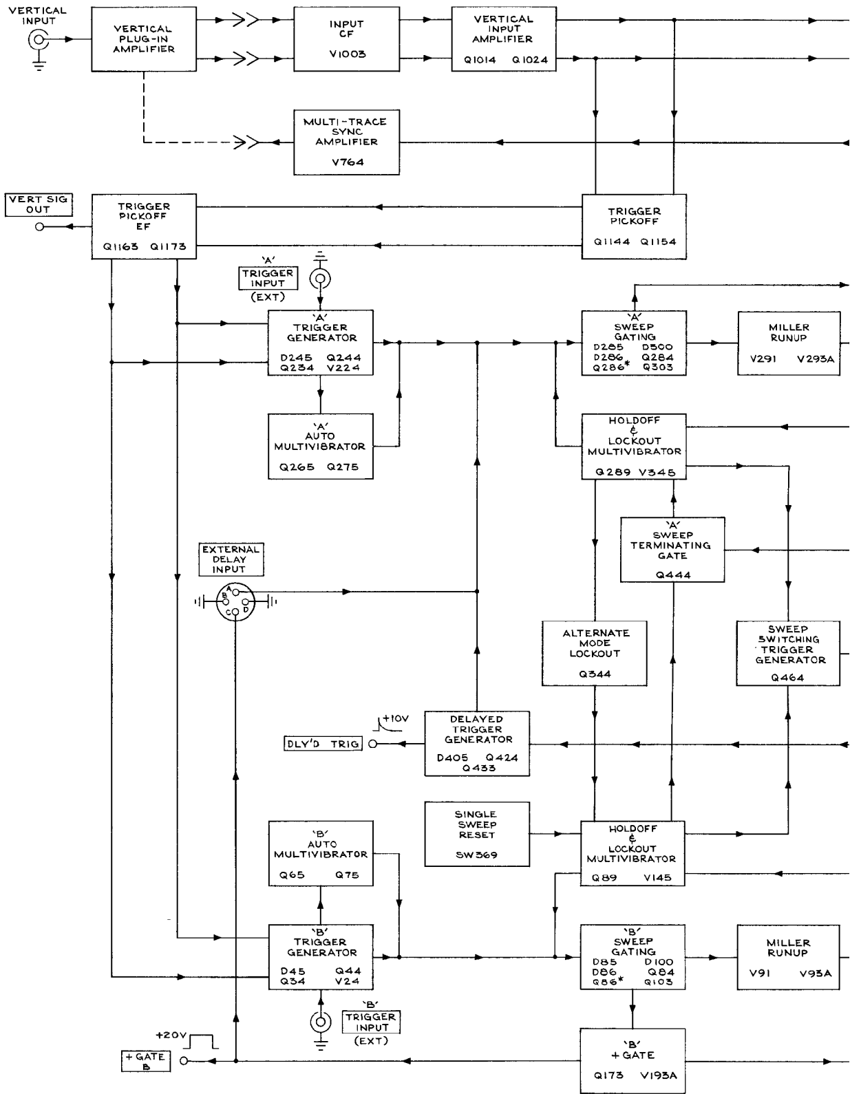
TYPE 547 OSCILLOSCOPE
