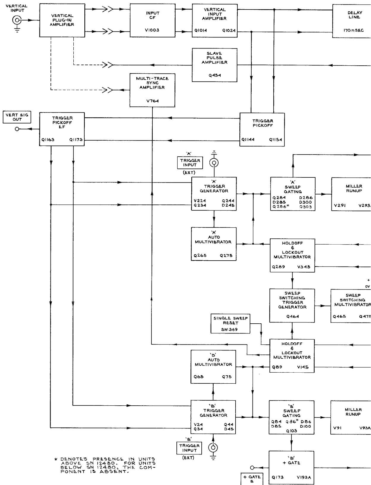
TYPE 547 OSCILLOSCOPE
