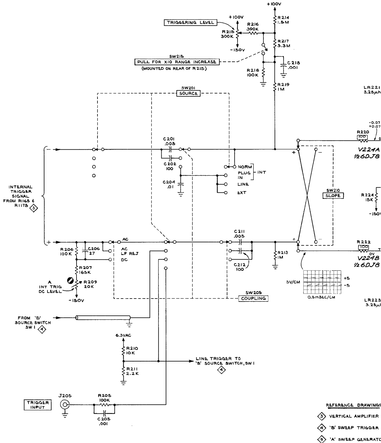
TYPE 547 OSCILLOSCOPE
