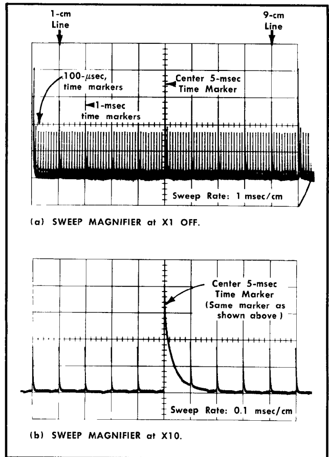
Fig. 5-9. Time-marker displays.
