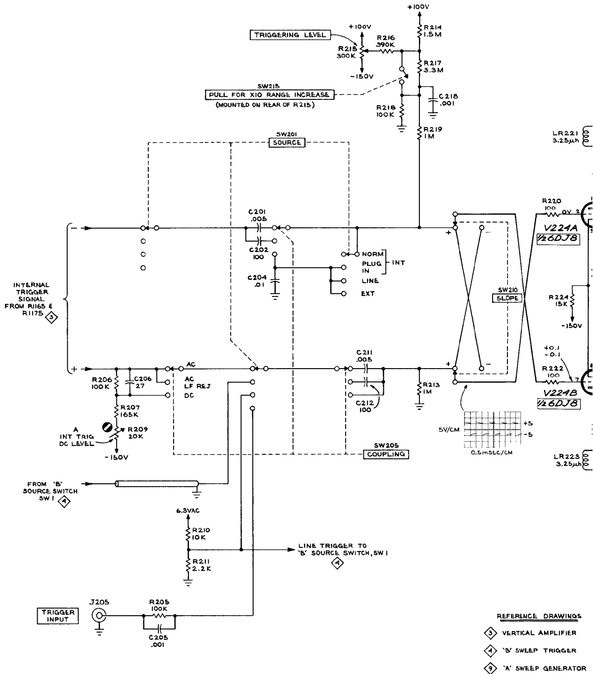
TYPE 547 OSCILLOSCOPE
