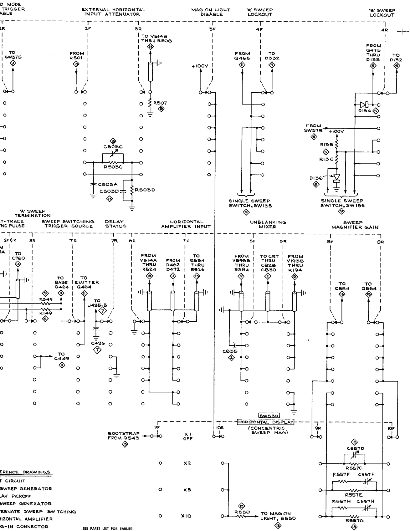
HORIZONTAL DISPLAY SWITCH 12 DON 866
