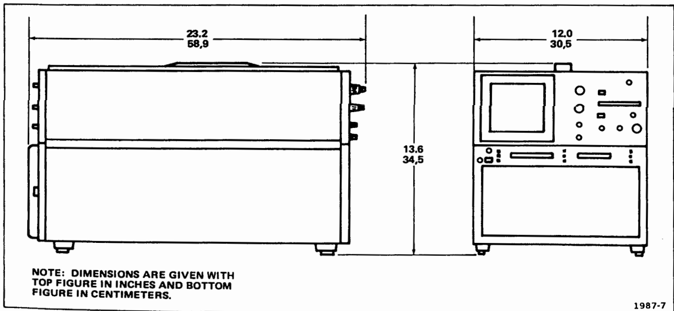
Figure 1-1. 7834 dimensional drawing.
