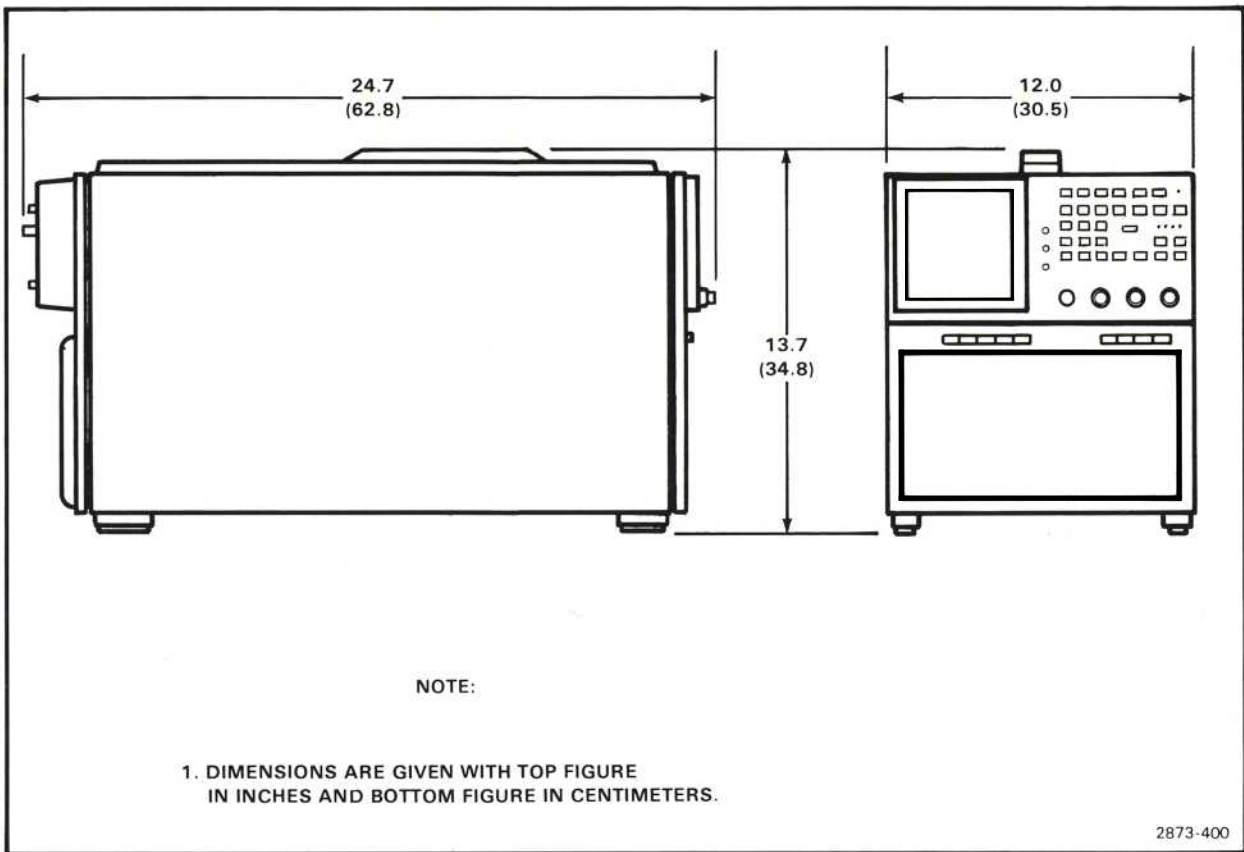
Figure 2-1. 7854 Mainframe dimensional drawing.
