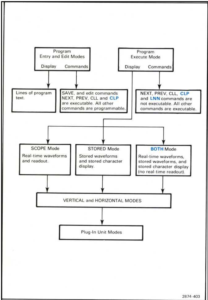
Figure 9-1. The 7854 hierarchy of operational modes.
