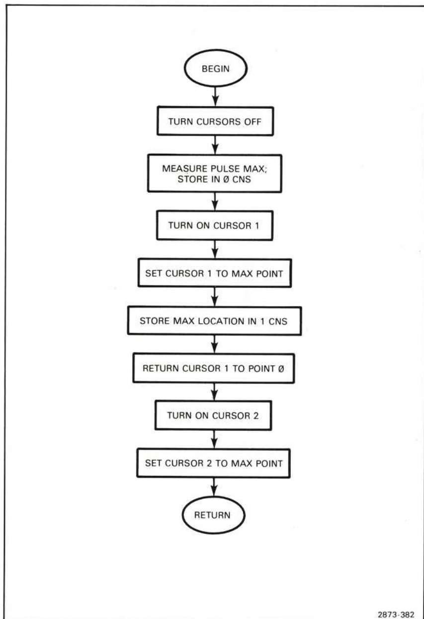
Figure 6-14. Flowchart of the cursor-positioning subroutine.
