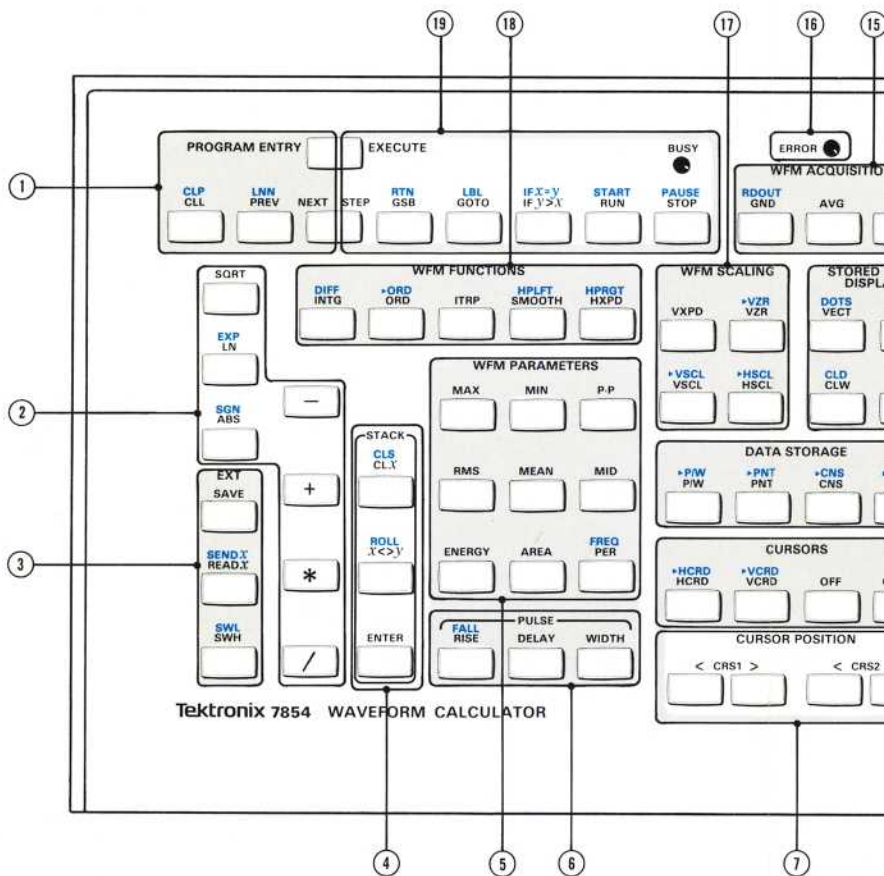
Figure D. Locator for Waveform Calculator keys and i
