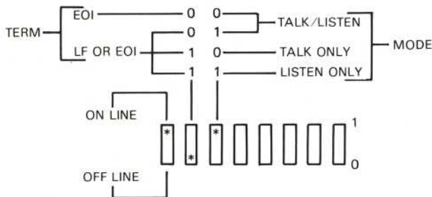
Figure 7-2. Address and mode selection.
