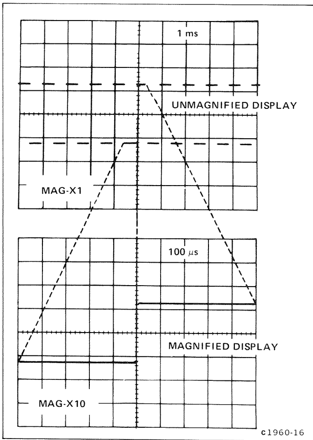
Figure 2-4. Effect of sweep magnifier on crt display.
