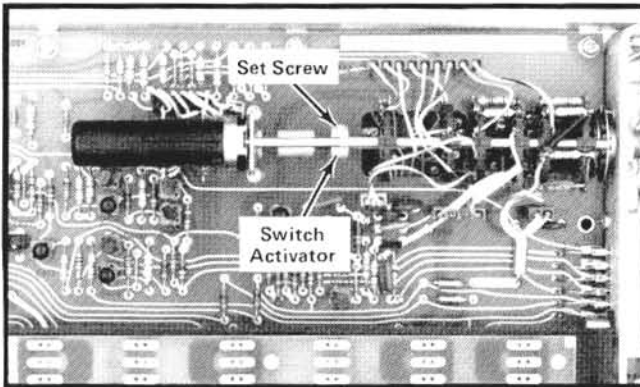
Fig. 4-2. Readout adjustment location, instrument left side.
