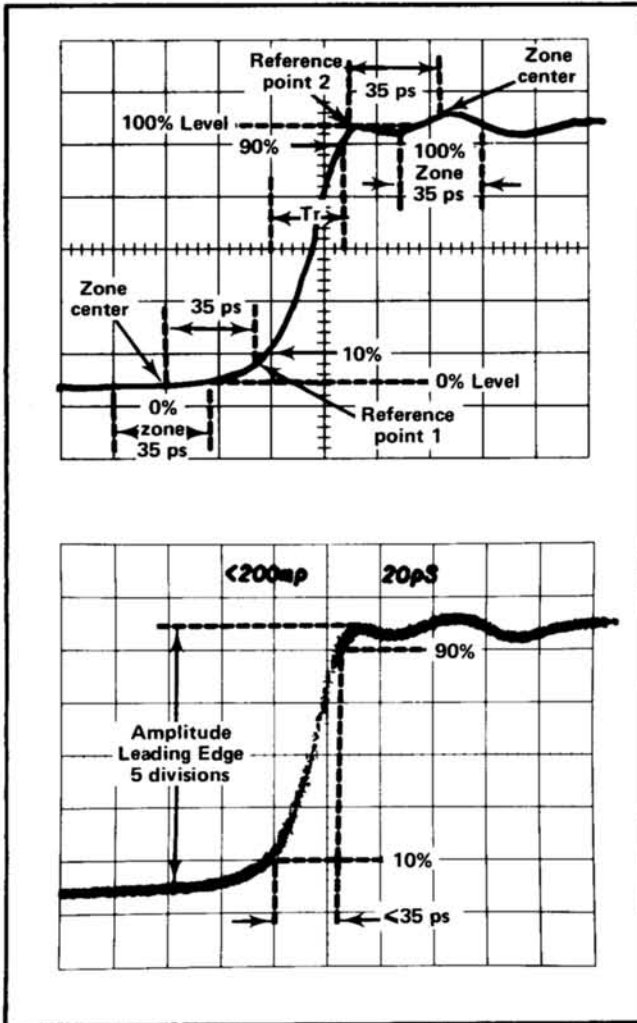
Fig. 5-7. Incident pulse risetime of the S-6, S-52 and 7S12 system.
