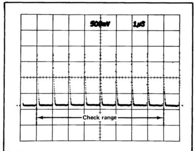
Fig. 5-3. Correct TIME/DIV check range. One μs period markers are shown.
