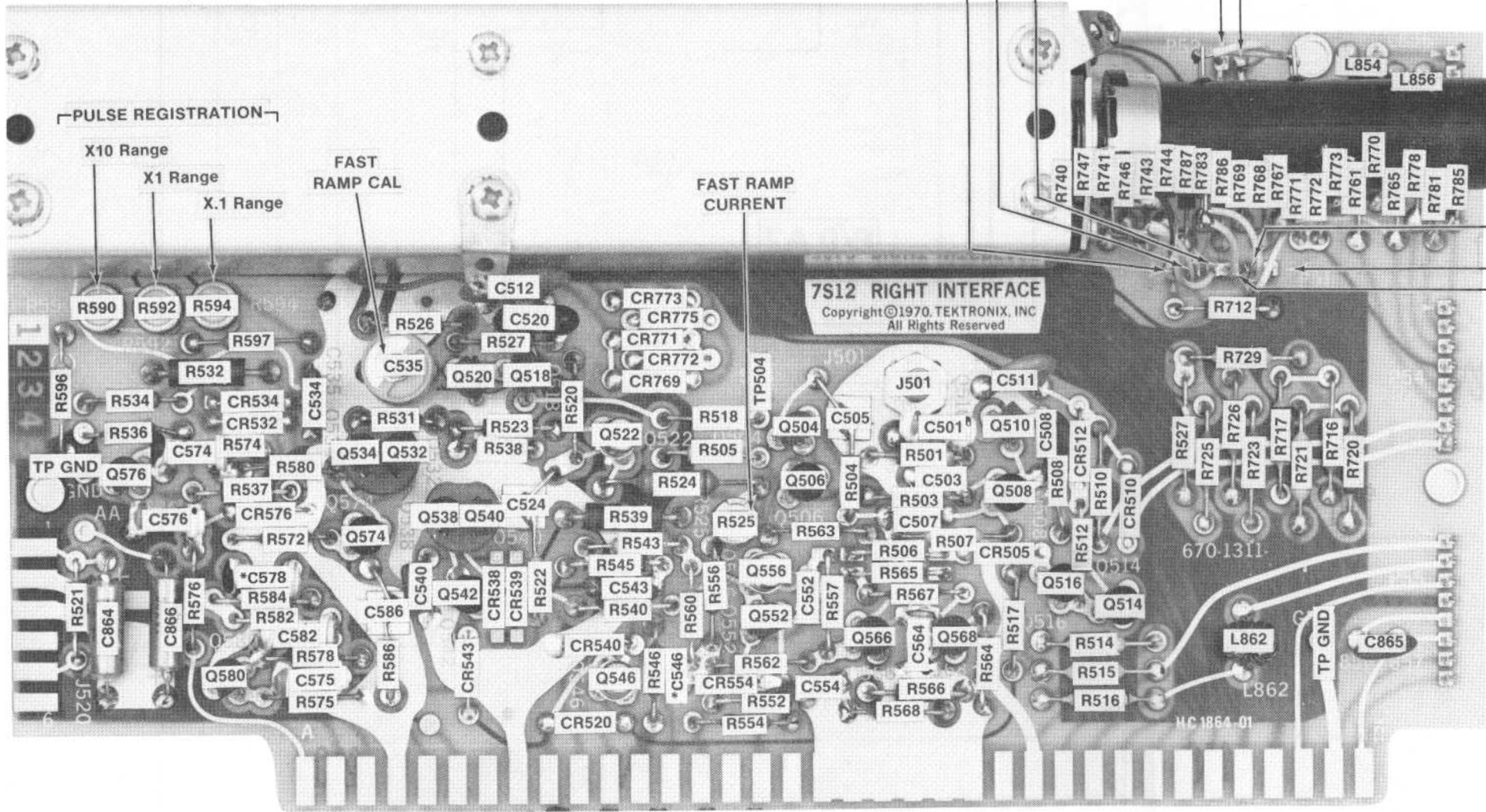
Fig. 7-3a, Assembly A-3, Right Interface (SN B10000 & up).
