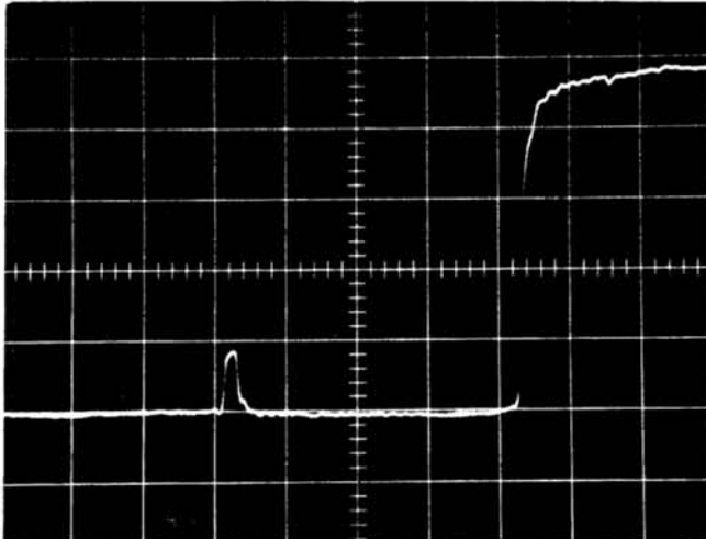
140 ps TDR System Risetime not degraded Amplitude correct
