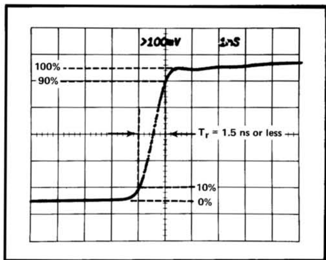
Fig. 5-10. Incident pulse risetime of the S-5, S-54 and 7S12 system.
