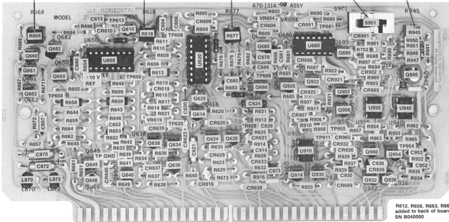
Fig. 7-4a. Assembly A-4, Horizontal Card (SN B10000 & up).
