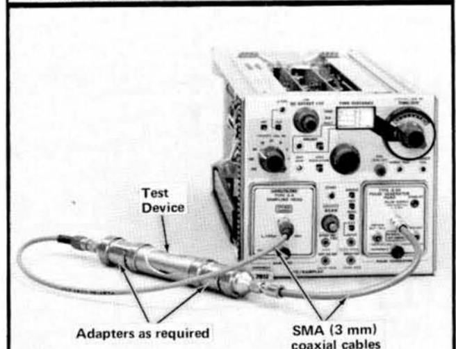
(B) "In Line" connections for short length cable TDR measurements. The transmission system under test must have two ports with low attenuation between them. SMA (3 mm) semi rigid cables are used with the proper adapter to the device under test. Use the 7S12 Multiplier setting of X.1.
