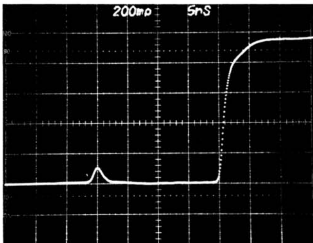
1.5 ns TDR System Risetime not degraded Amplitude reduced
