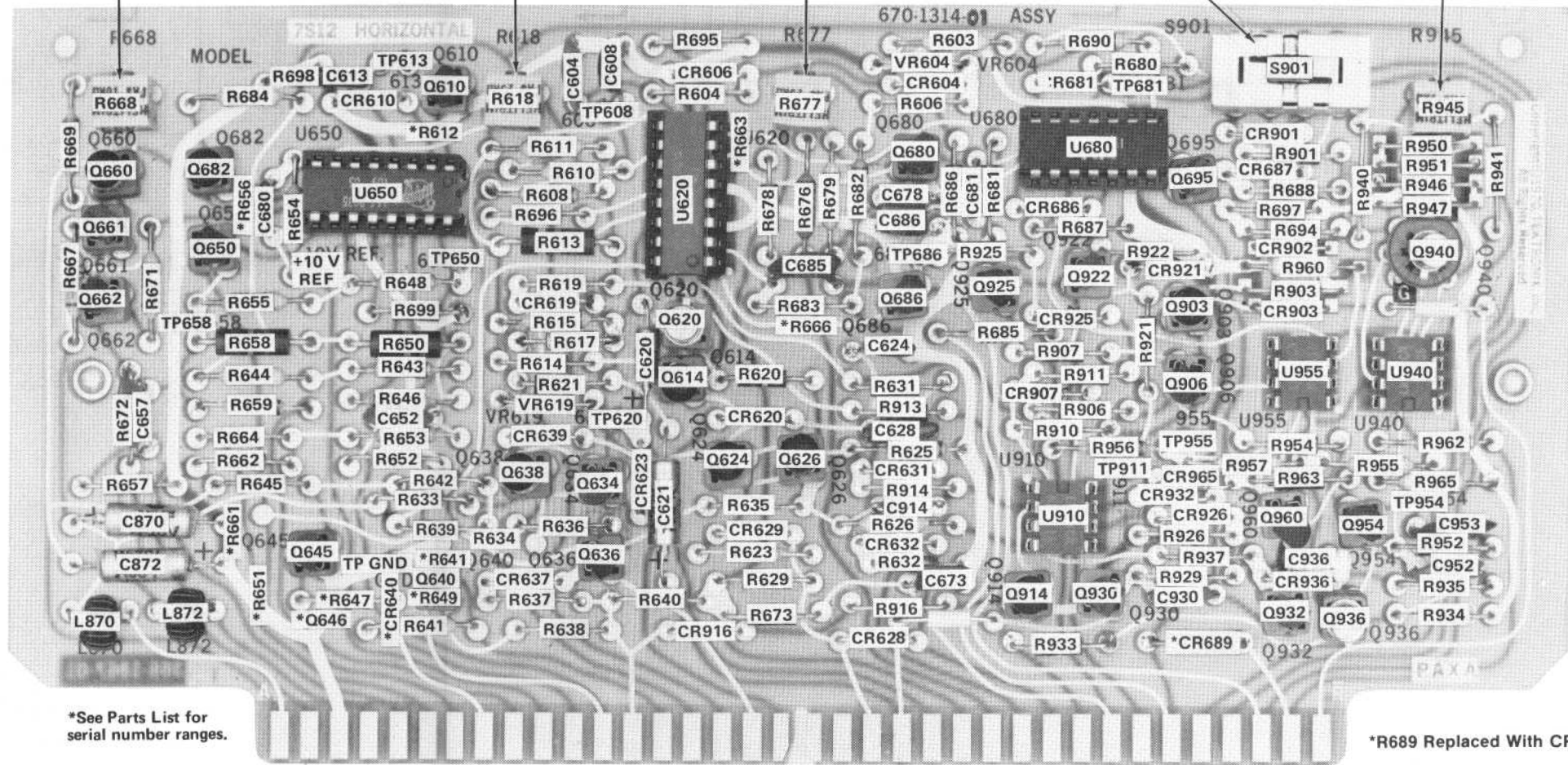
Fig. 7-4b. Assembly A-4, Horizontal Card (below SN B10000).
