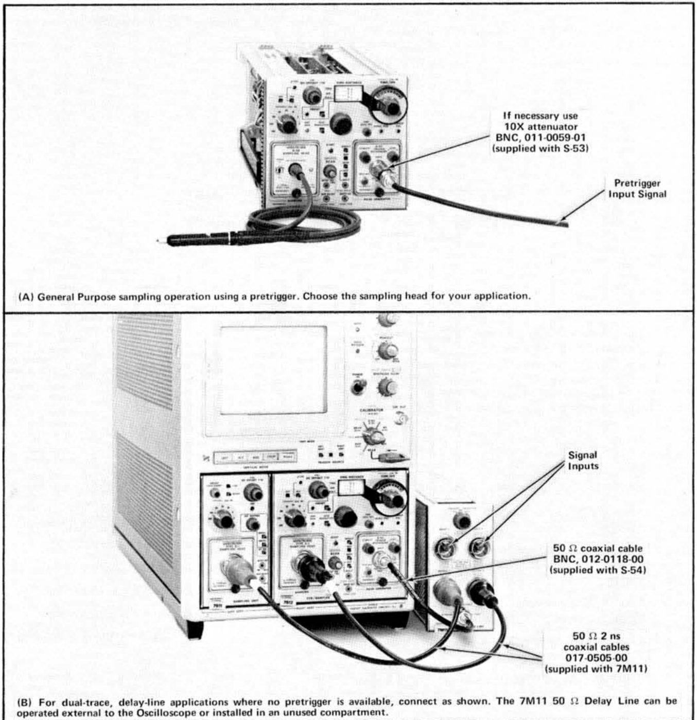
Fig. 2-13. General Purpose sampling.
