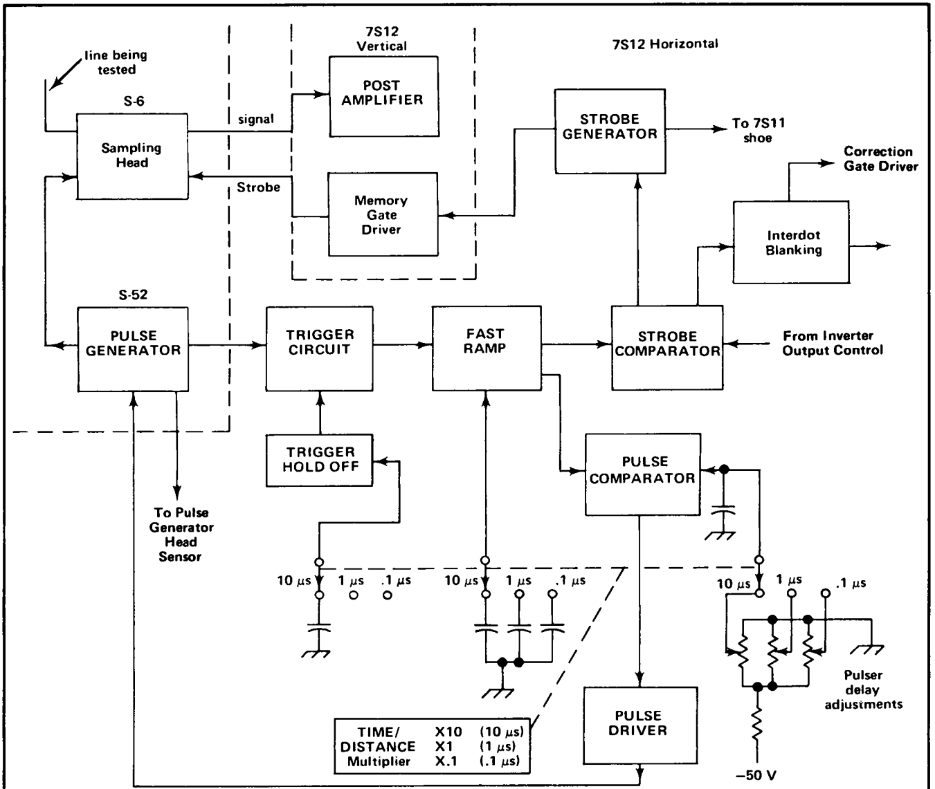
(a) Partial Horizontal Circuit block diagram
