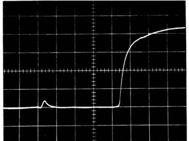
140 ps TDR System Risetime degraded Amplitude reduced
