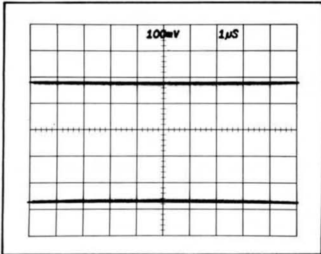
Fig. 5-12. Waveform for Memory Gate Width control R390 adjustment using a Normalizer Head.
