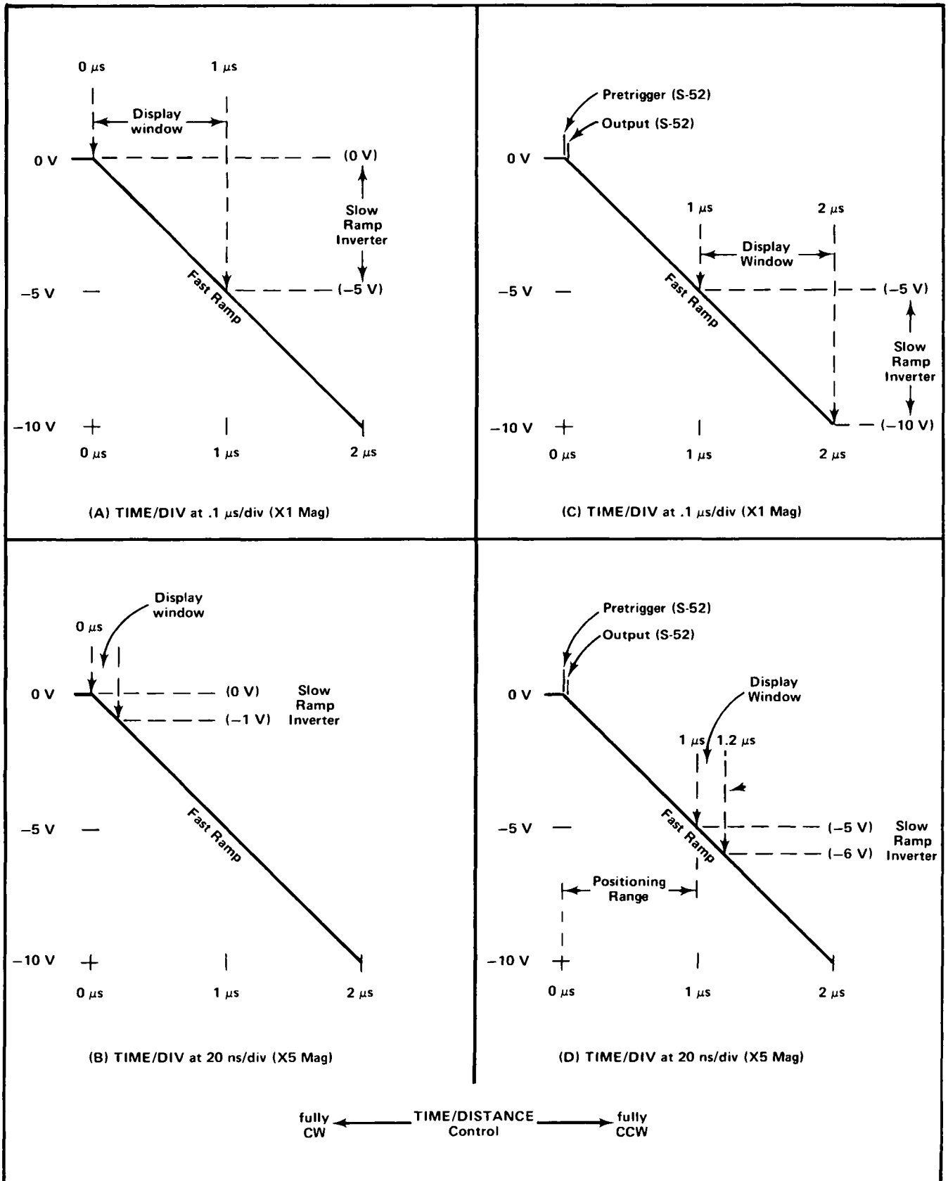
Fig. 3-7. Effect of TIME/DIV and TIME/DISTANCE controls on the display window. (TIME/DISTANCE Multiplier at X1).
