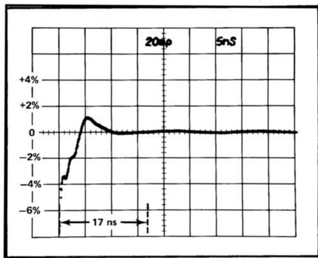
Fig. 5-9. Pulse aberrations of the S-5, S-54 and 7S12 system.
