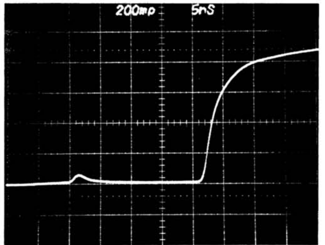
1.5 ns TDR System Risetime degraded Amplitude further reduced
