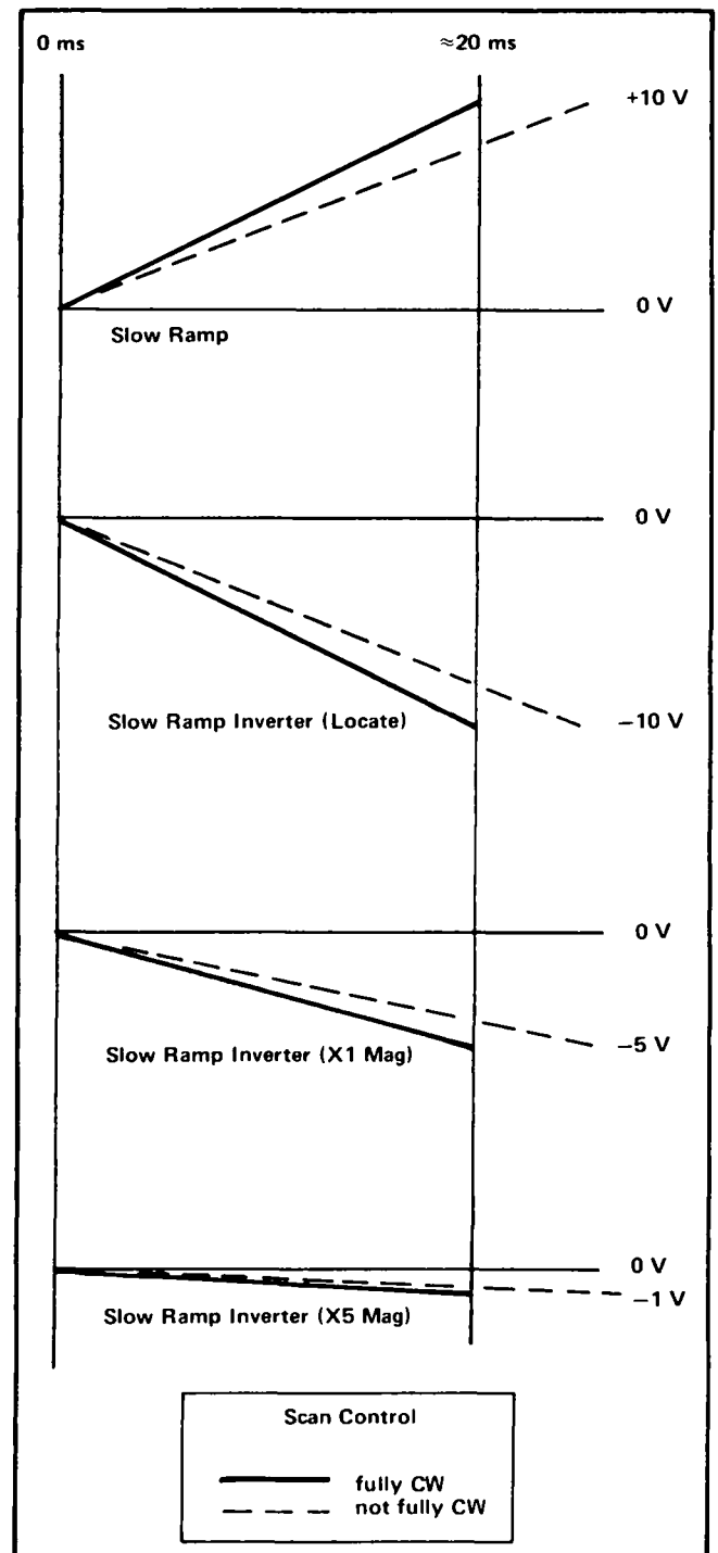
Fig. 3-6. Slow Ramp and Slow Ramp Inverter outputs (TIME/DISTANCE control fully CW to 0 \mu s).
