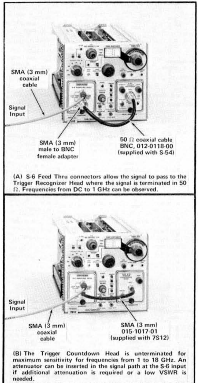
Fig. 2-12. High Frequency Signal Application.
