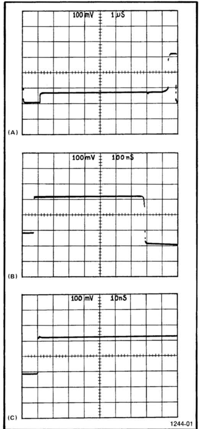
Fig. 2-3. First Time Operation showing Multiplier setting (A) X10, (B) X1 and (C) X.1.
