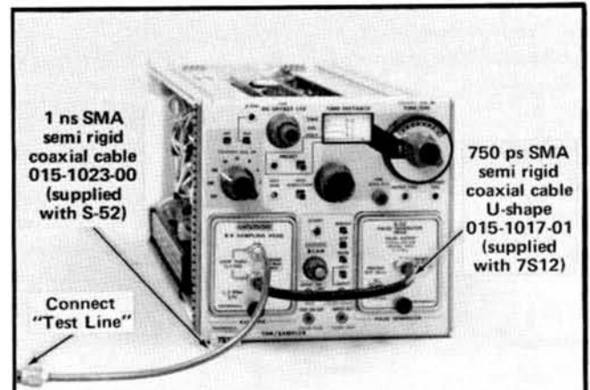
(A) "Loop Thru" connections for short and medium length cable TDR measurements. The "Test Line" is connected to the end of the 1 ns semi rigid line for minimum aberrations and fast risetime. Use the 7S12 Multiplier settings of X.1 and X1 (limited by the S-52 pulse duration).
