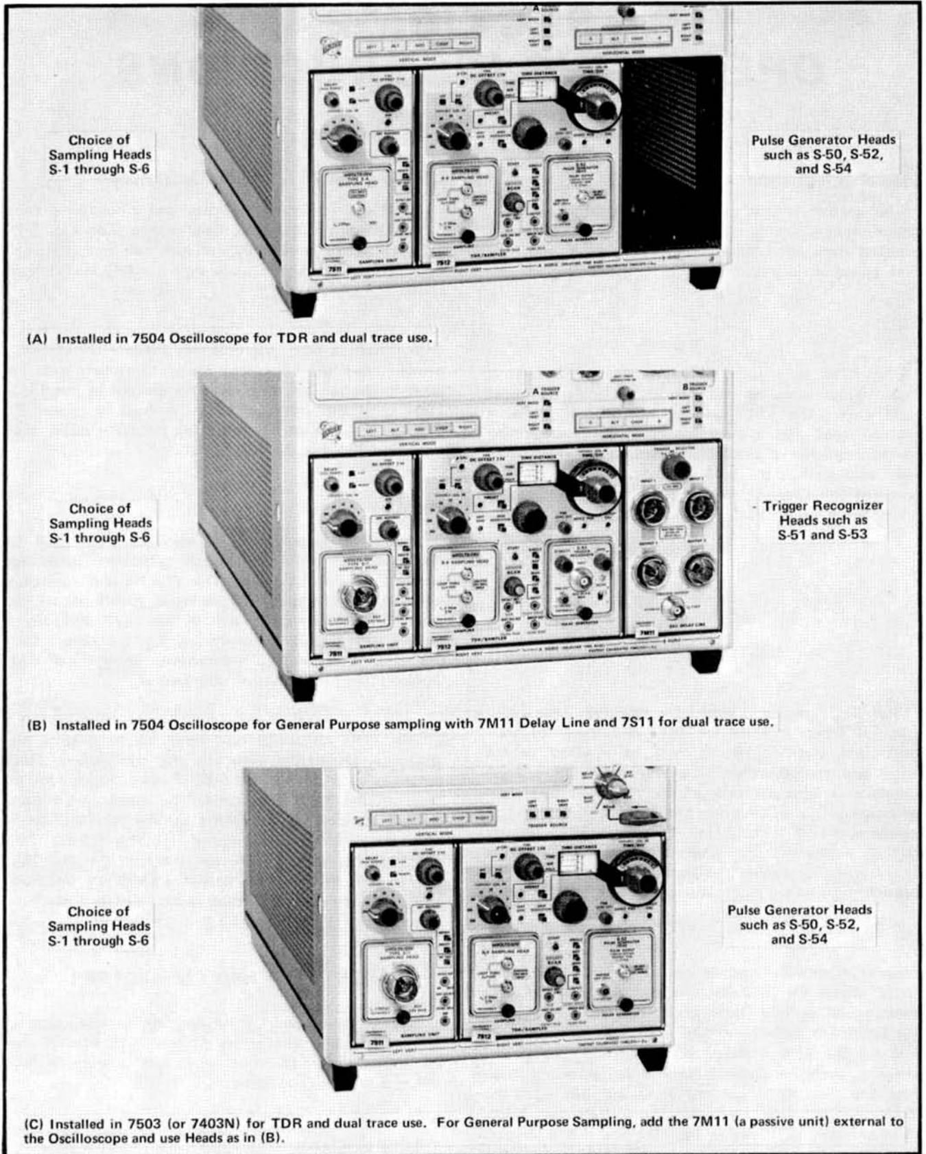
Fig. 2-1. 7S12 Installation Information.
