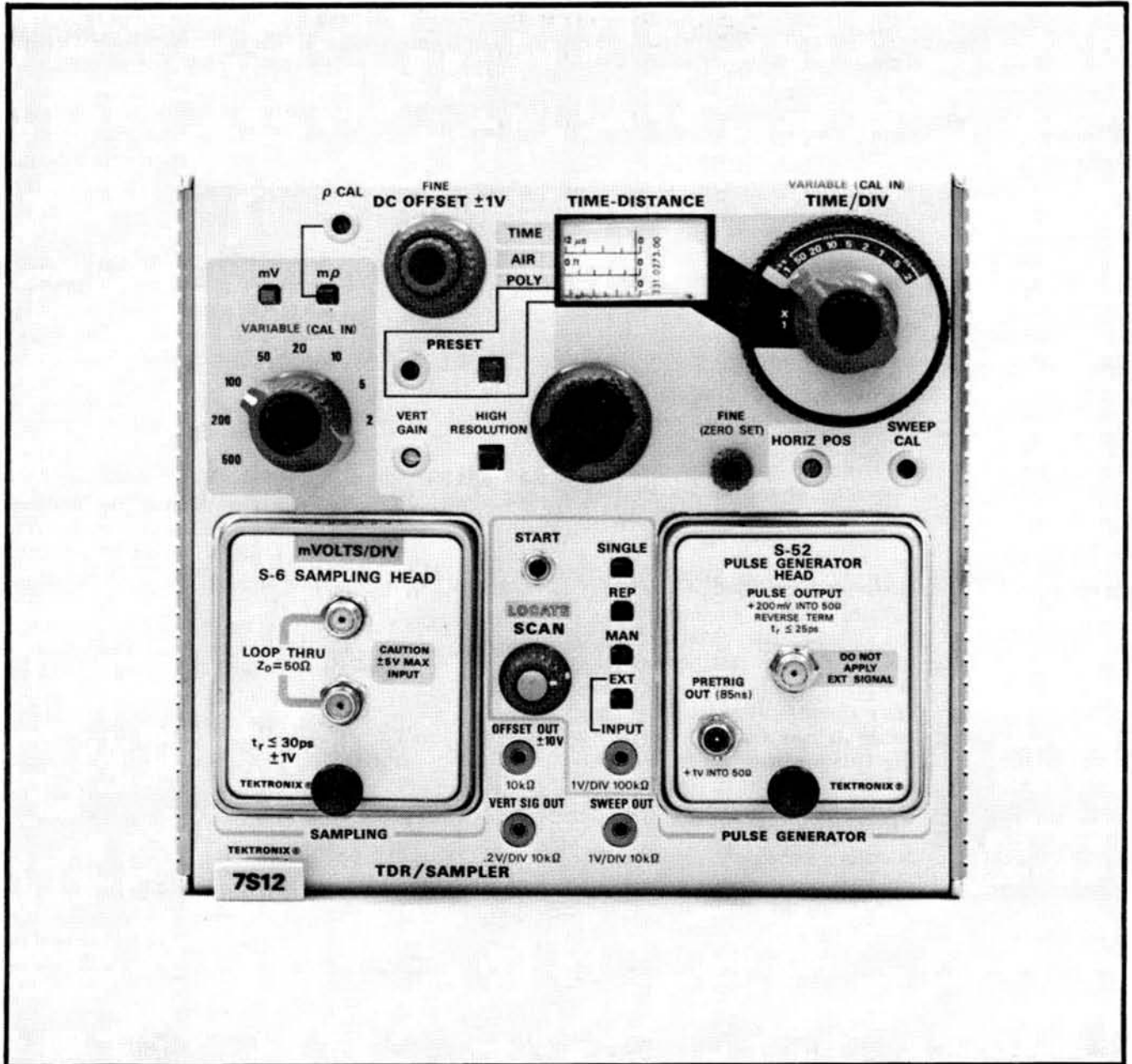
Fig. 2-2. 7S12 front panel.
