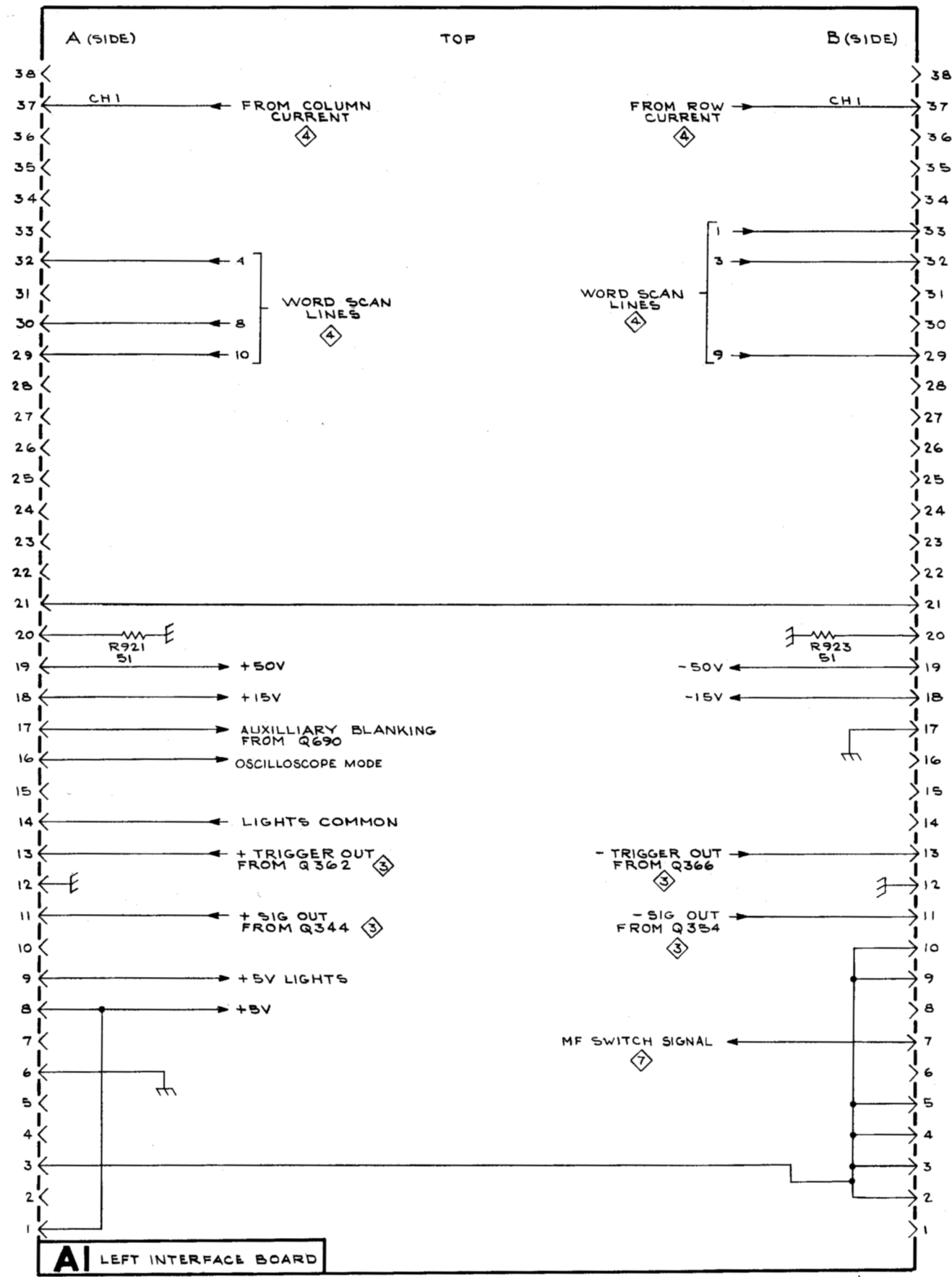
VERTICAL OUTPUT CONNECTORS
