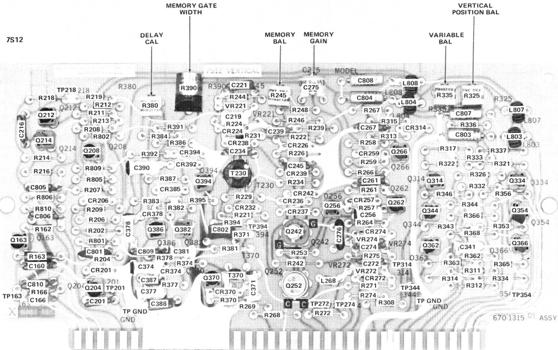
Fig. 7-2. Assembly A-2, Vertical Card.
