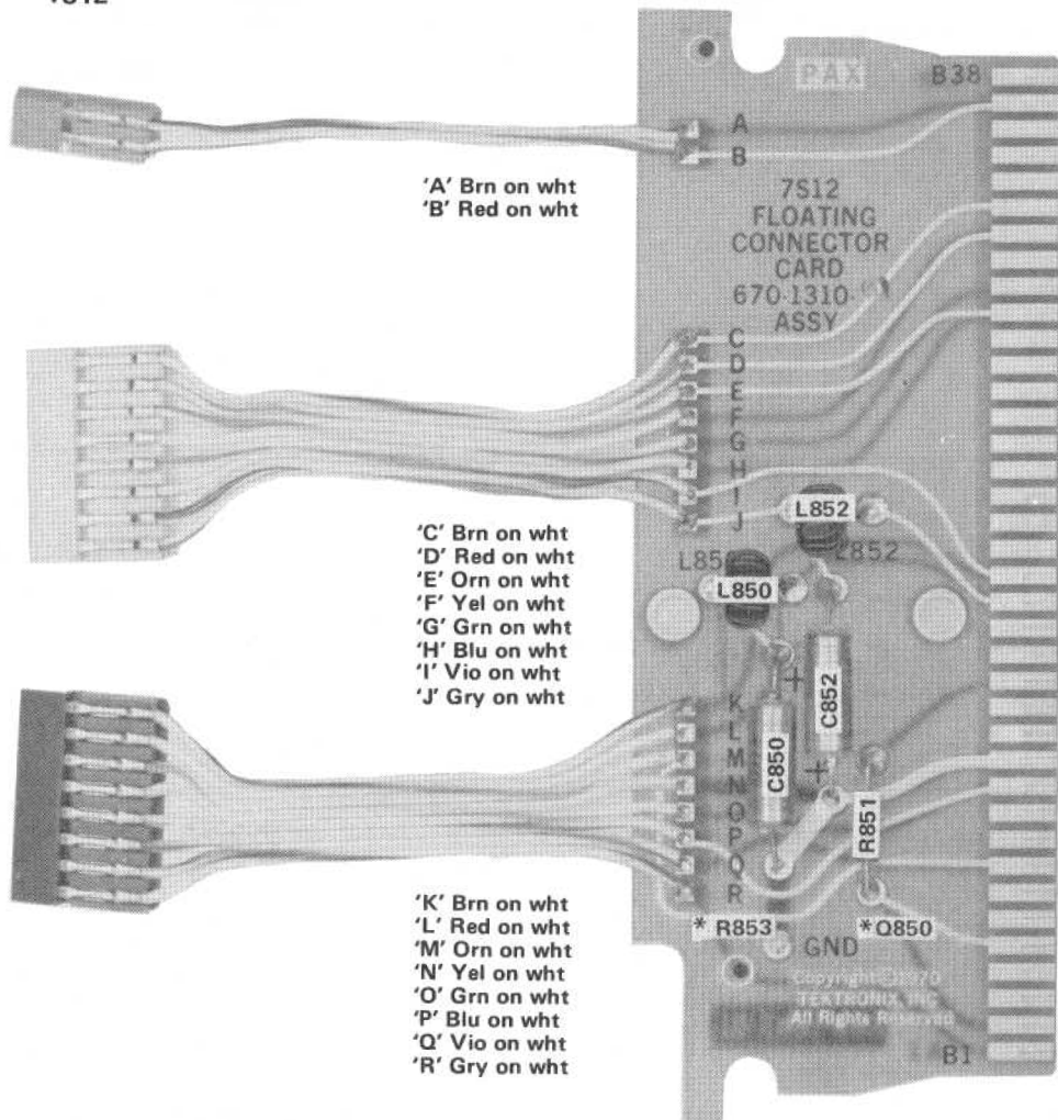
Fig. 7-6. Assembly A-6, Floating Connecting Board.
