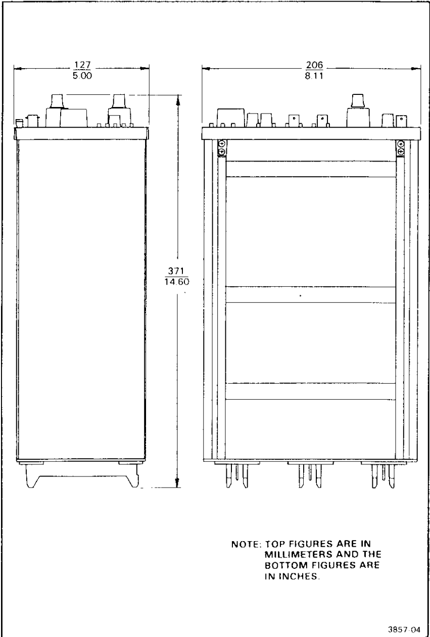
Figure 1-2. Dimensional Drawing.
