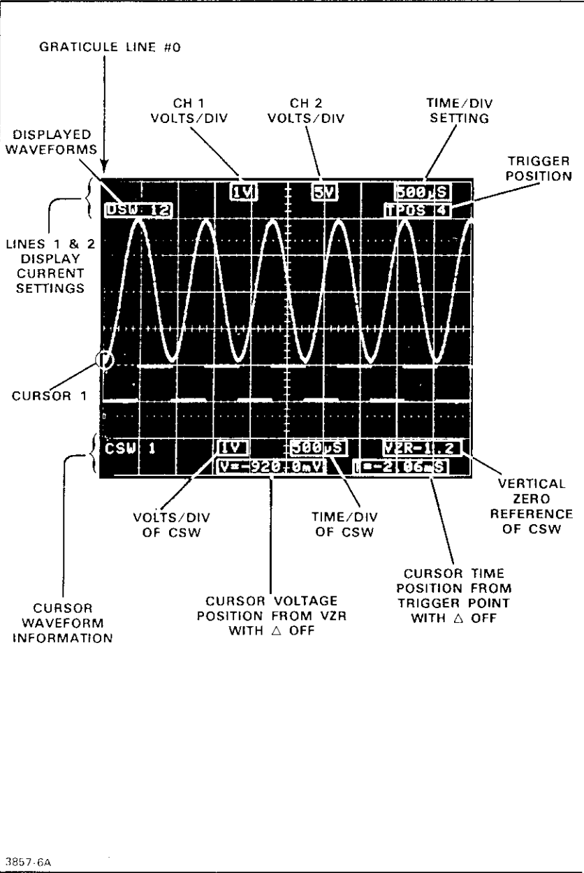
Figure 2-2. 7D20 Display.
