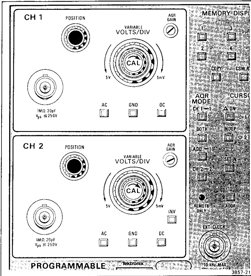
Figure 2-13. Vertical controls.
