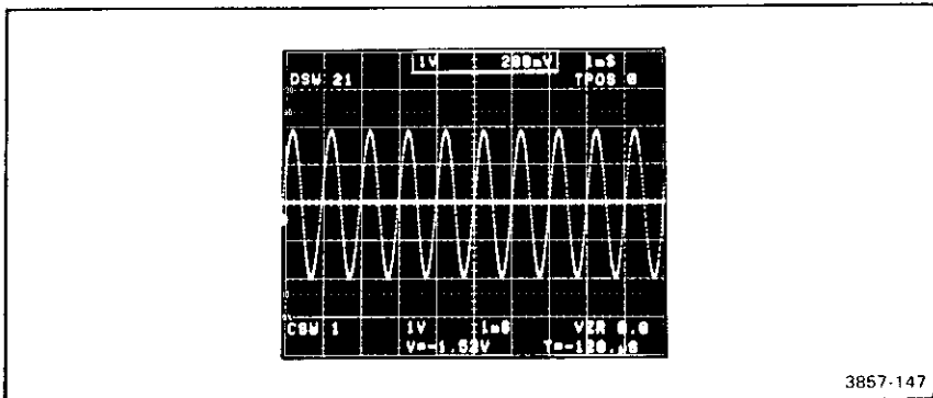
Figure 2-45. VOLTS/DIV readout.
