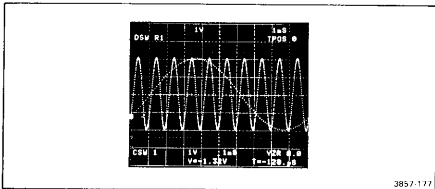
Figure 2-55. DSV readout with R (Reference) Waveform displayed.
