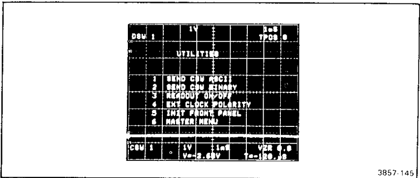
Figure 2-40. UTILITIES MENU.
