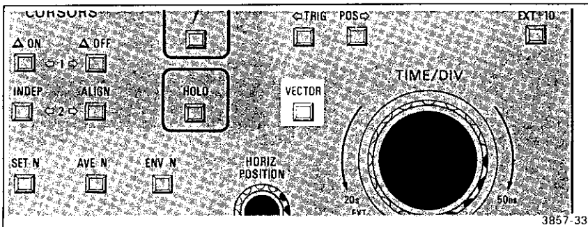
Figure 2-32. VECTOR key.
