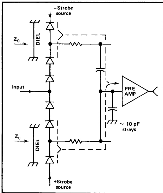
Fig. 3-5. error-signal source and path to Pream shown by dottedlines. DIEL denotes dielectric other than air
