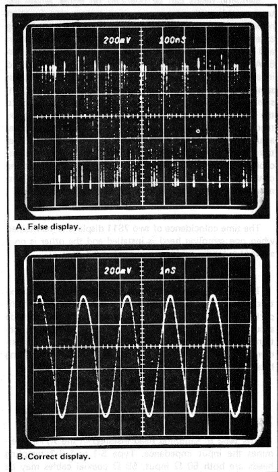
Fig. 2-8. Typical false and correct displays using a 500 MHz signal input
