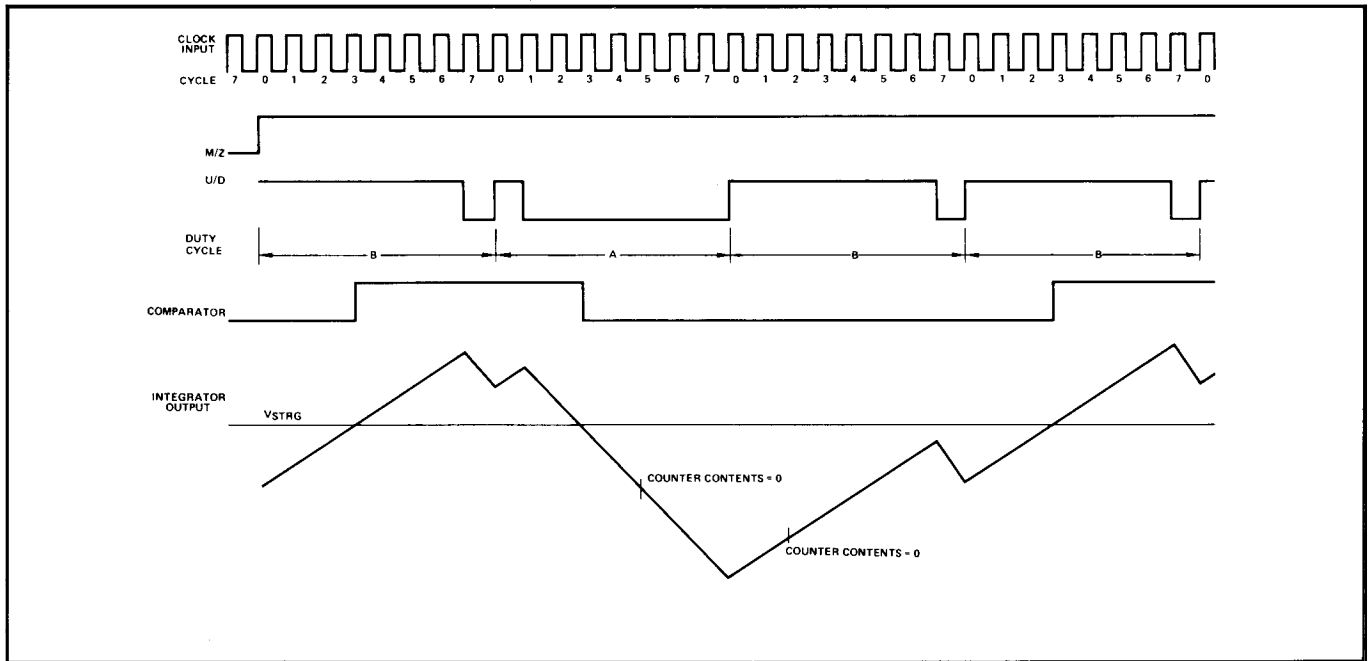
Fig. 2-4. Measurement interval timing. Reprinted by permission of Siliconix, Inc.
