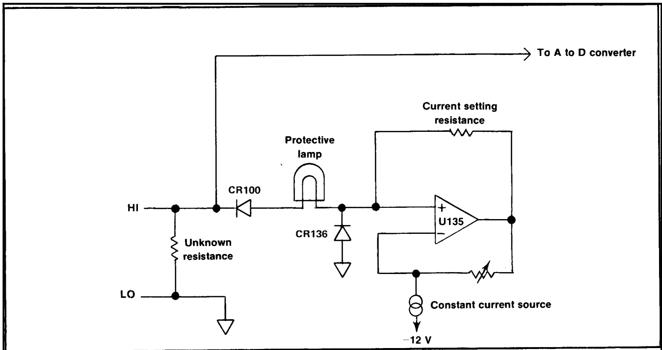
Fig. 2-1. Simplified diagram of Ohms Converter.
