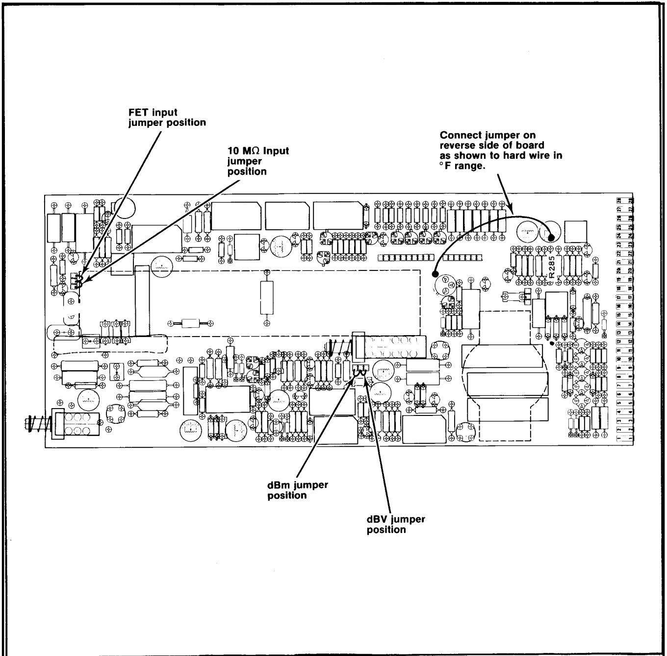
Fig. 1-2. Locations of dB reference jumper, input impedance jumper, and hard wired °C or °F component or wire changes.
