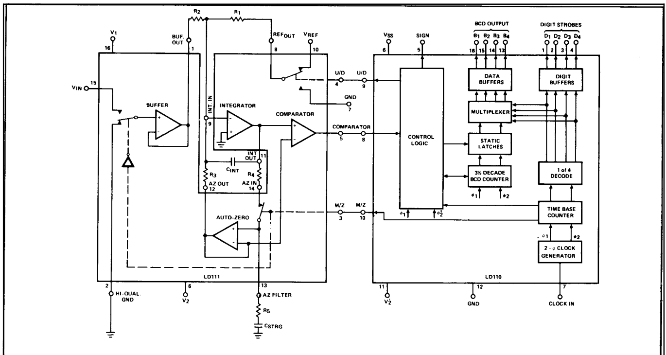
Fig. 2-2. Analog to digital converter and control logic block diagram. Reprinted by permission of Siliconix Inc.
