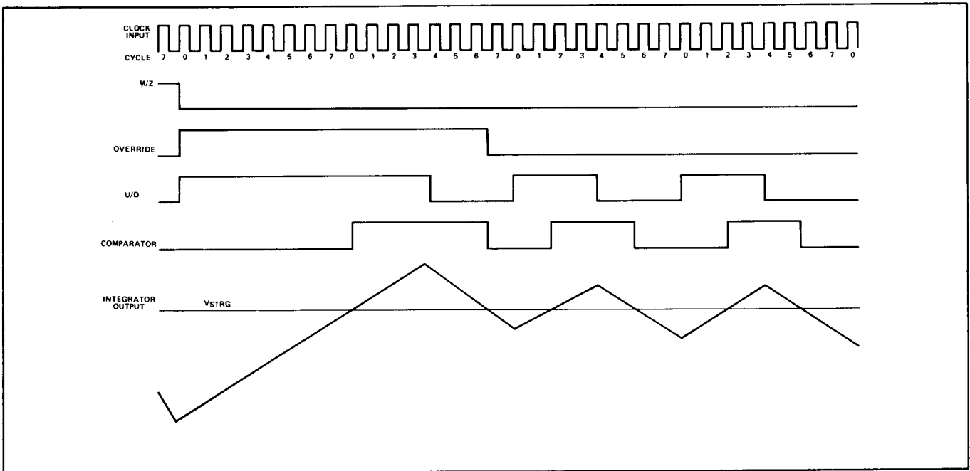
Fig. 2-3. Auto-zero timing intervals. Reprinted by permission of Siliconix Inc.
