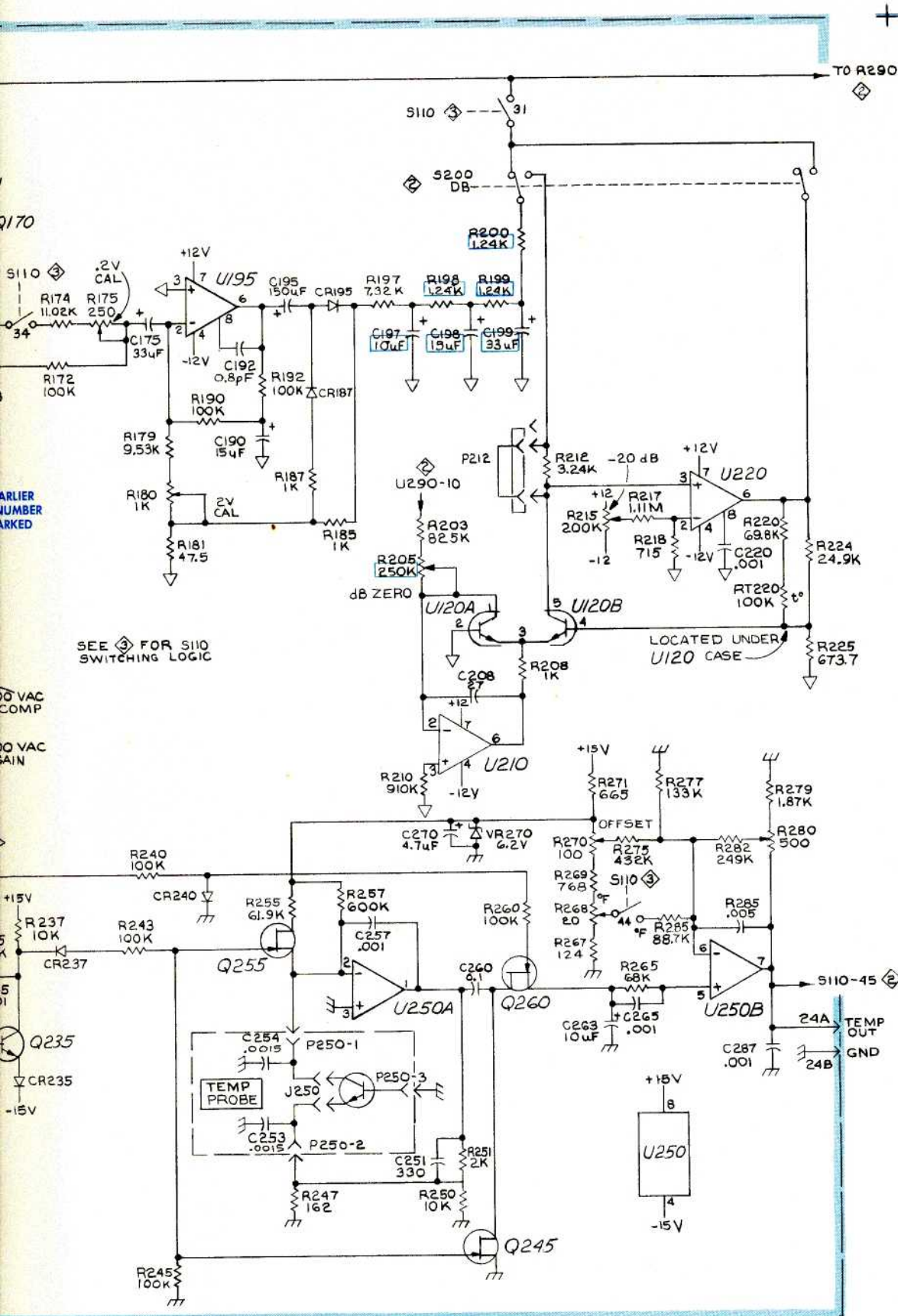
ATTENUATORS & CONVERSION CIRCUITS \diamond NS 8-12-74
