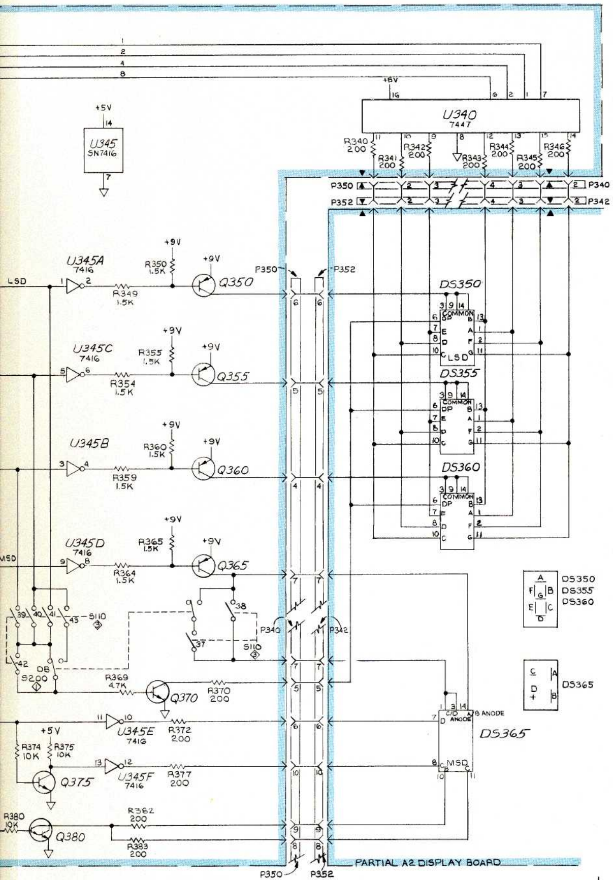
INTEGRATOR, A/D CONVERTER, DISPLAY
