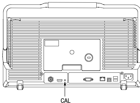
Figure 3- 1: Rear panel
