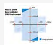
Model 2400 four-quadrant operation characteristics, a feature of all SourceMeter SMU instruments.
