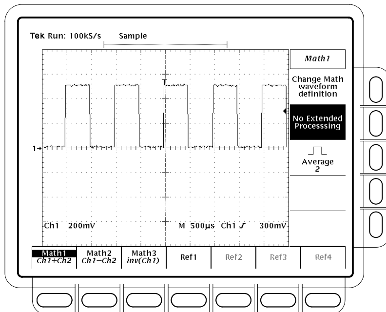
Figure 3–67: More Menu
