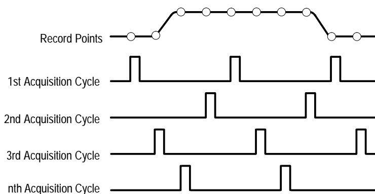
Figure 3–12: Equivalent-Time Sampling
