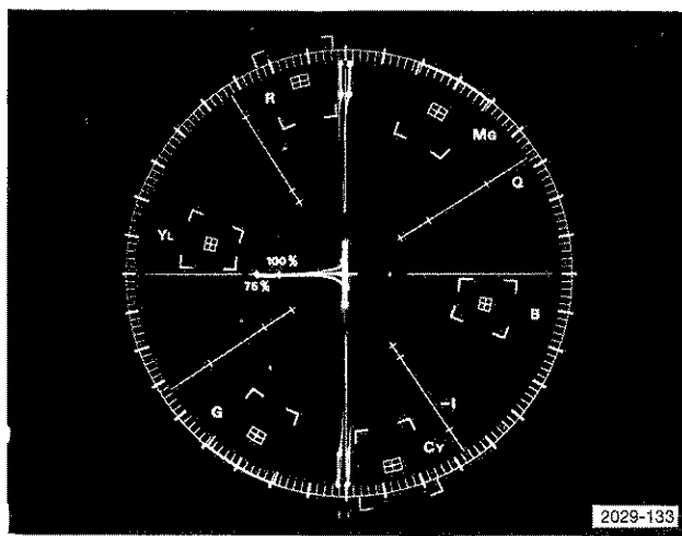
(B) R-Y 180^\circ Phase Switcher misadjusted.
