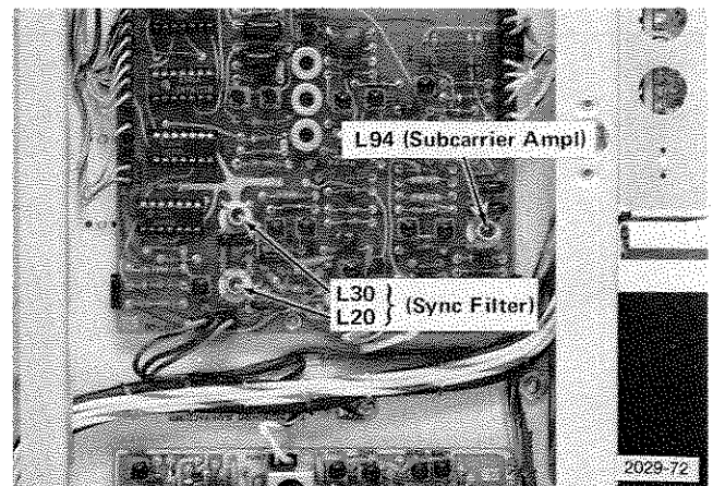
Fig. 3-4. Subcarrier & Sync filter adjustment locations.
