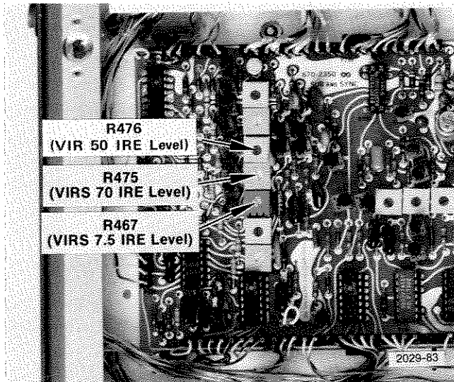
Fig. 3-15. 149A Subcarrier & Sync circuit board showing location of VIRS pedestal adjustments.
