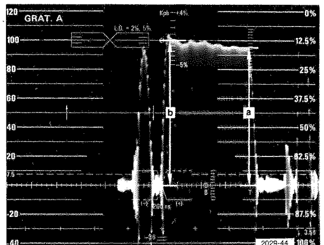
Fig. 1-12. Differential Gain as measured on a waveform monitor, using the COMPOSITE test signal.
