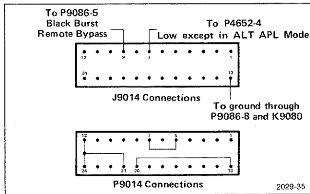
Fig. 1-3. Wiring diagram of Remote Plug for LOCAL operation (factory connected).
