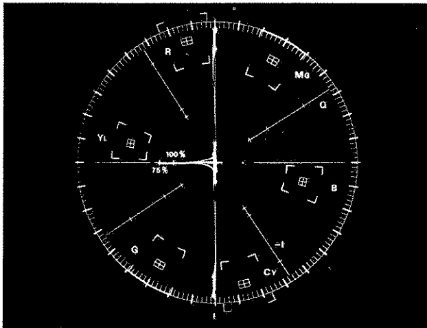
(A) R-Y 180^\circ Phase Switcher properly adjusted.
