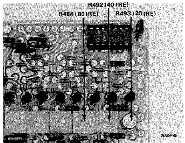
Fig. 3-27. 149A Modulated Pedestal chrominance adjustment locations.
