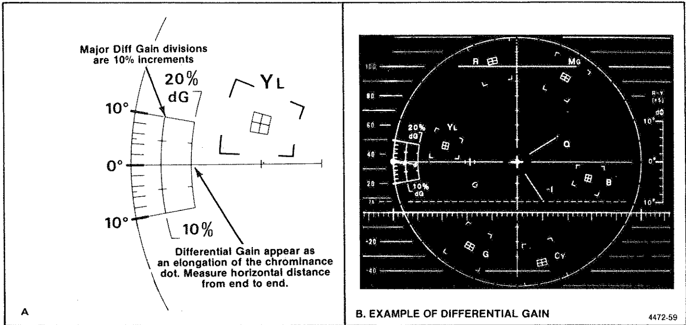
Fig. 2-18. Interpreting a differential gain measurement.
