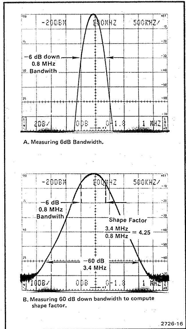
Fig. 3-5. Displays that illustrate how bandwidth and shape factors are determined.
