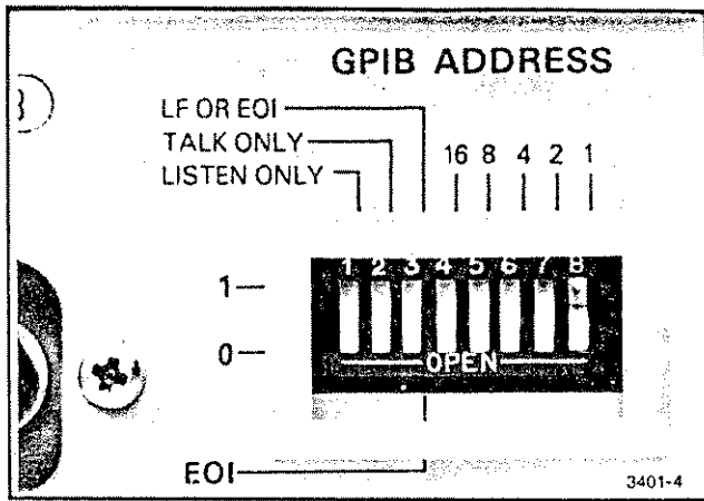
Fig. 3-19. GPIB Address switches on the rear panel.
