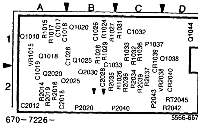
Fig. 10-63. A30A2—Fan Drive circuit board.
