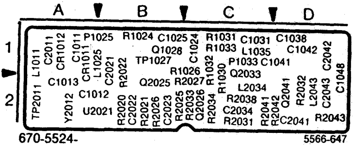
670-5524- Fig. 10-55. A50A5—Controlled Oscillator circuit board.
