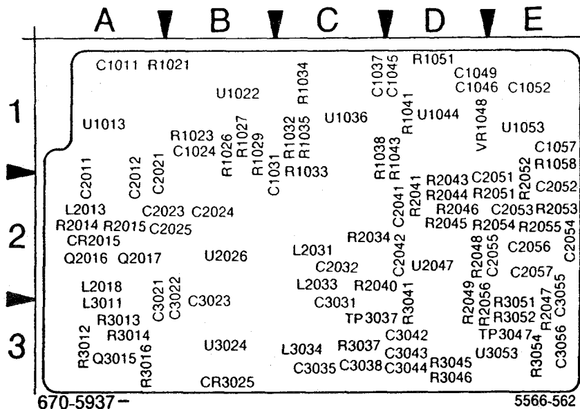
Figure 10-8. A23A2—25 MHz Phase Lock circuit board.
