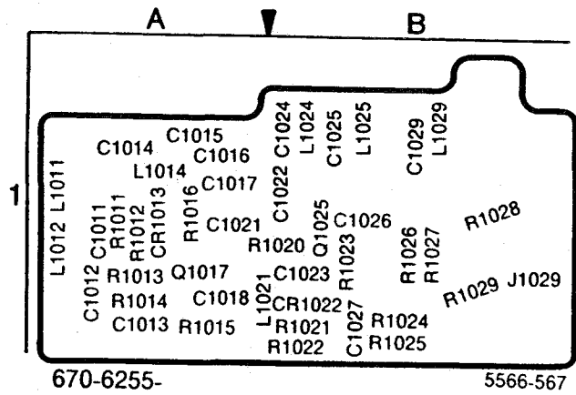
Figure 10-11. A23A5—829 MHz Amplifier circuit board.
