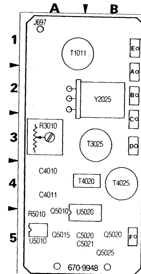
Fig. 10-22 A69A1 — 1st Mixer circuit board (front)
