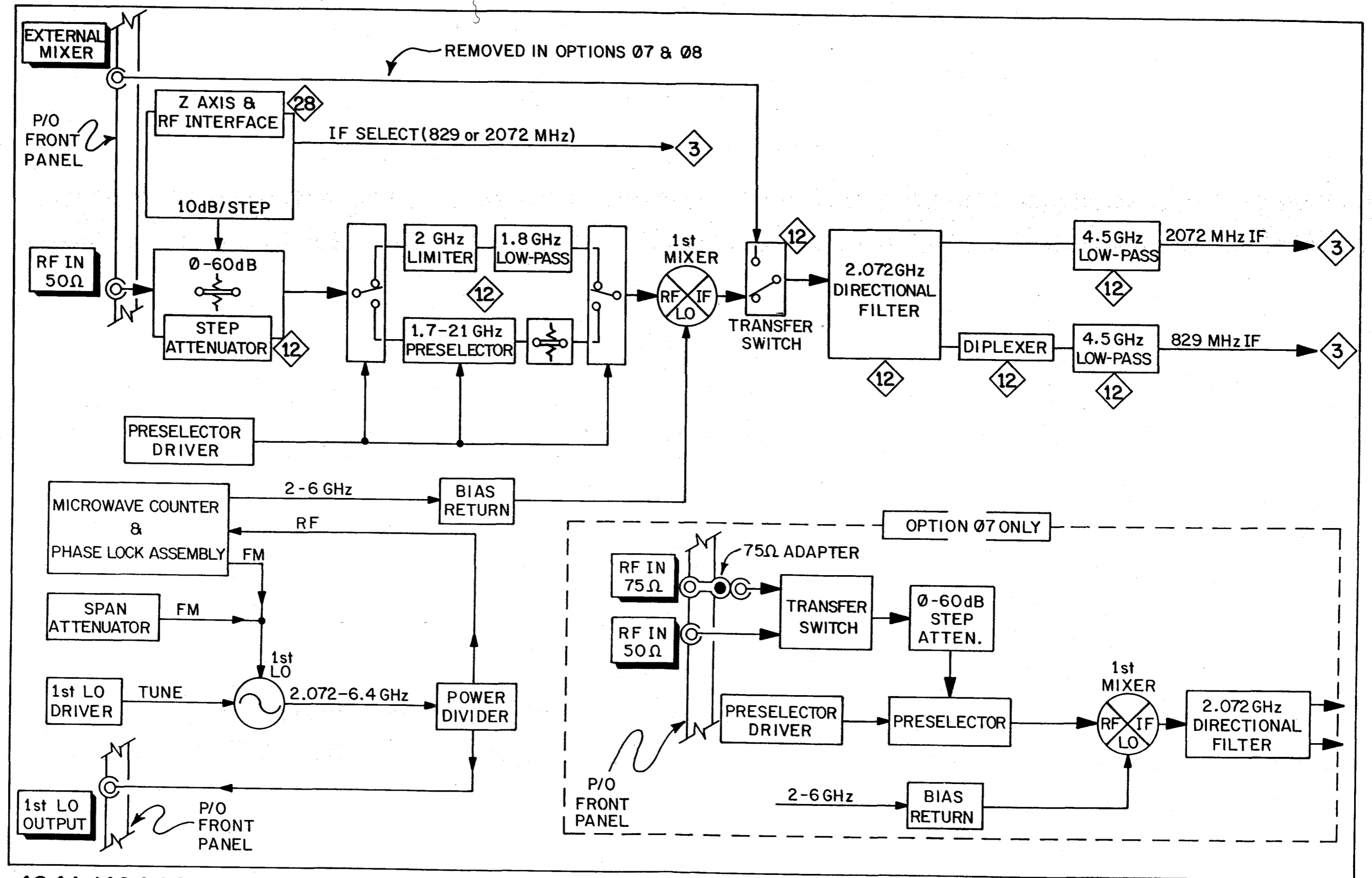
1st CONVERTER BLOCK DIAGRAM 2
