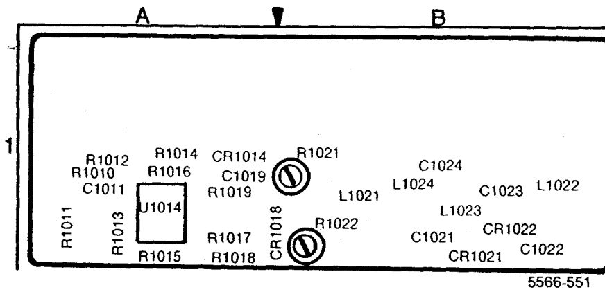
Figure 10-2. A18A1—2072 MHz 2nd Converter circuit board.
