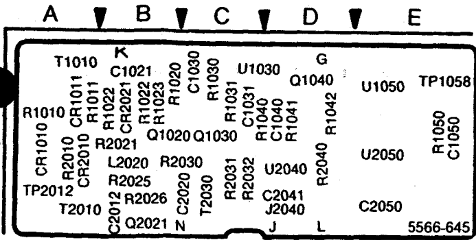
670-5522- Fig. 10-53. A50A3—Offset Mixer circuit board.
