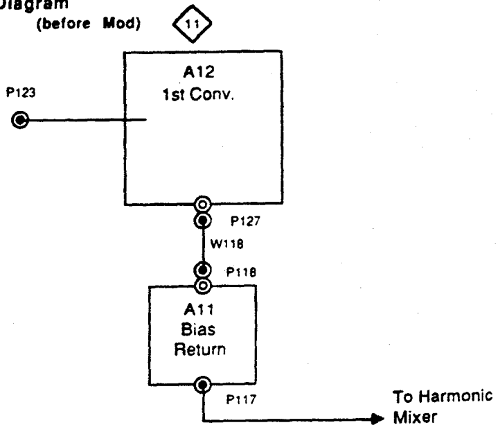
RF Interconnect Diagram (after Mod)
