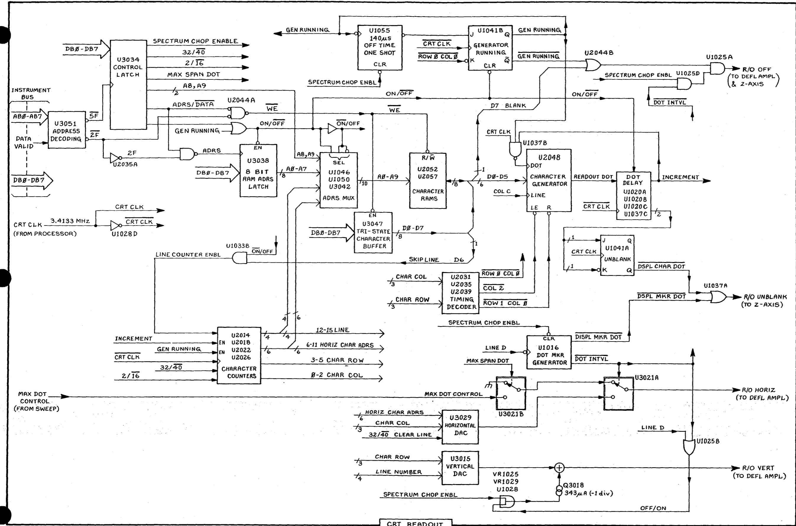
CRT READOUT 5566-616
