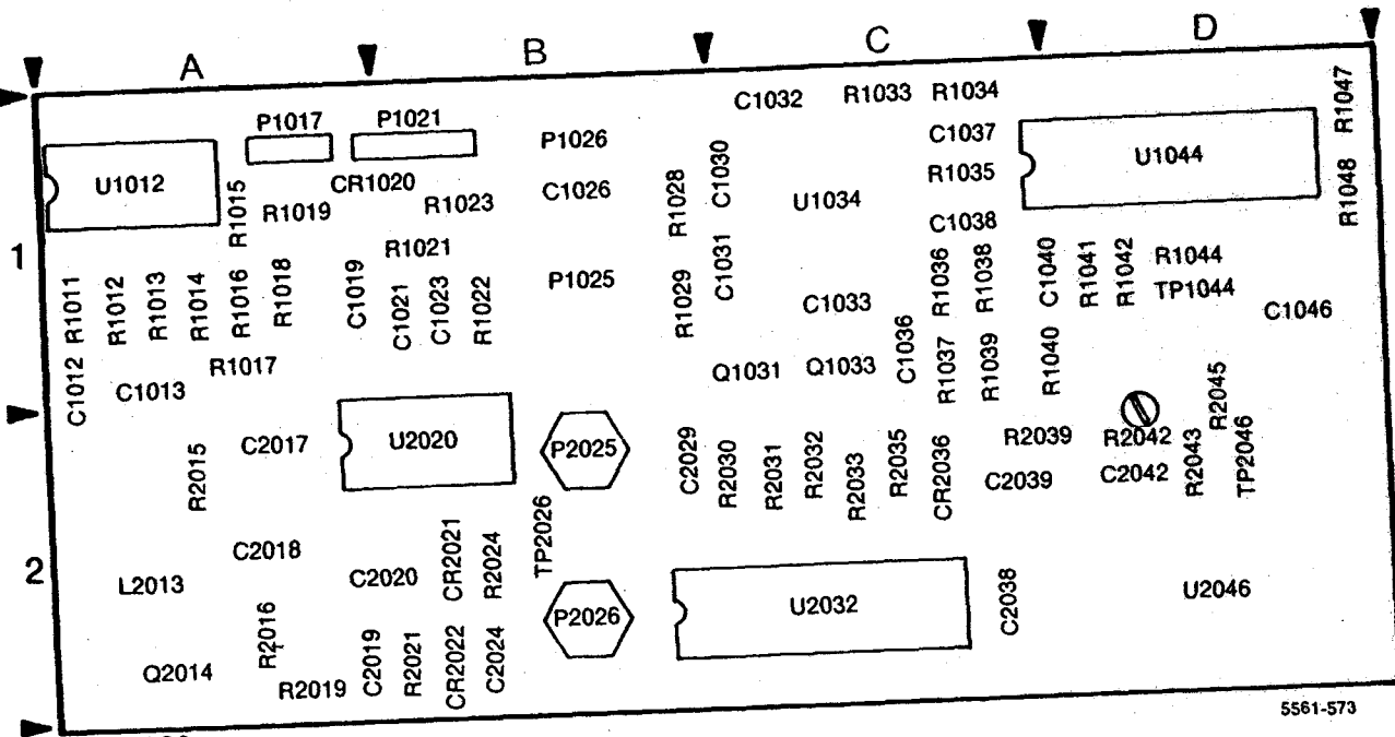
Fig. 10-64. A36A1—Reference Lock circuit board.
