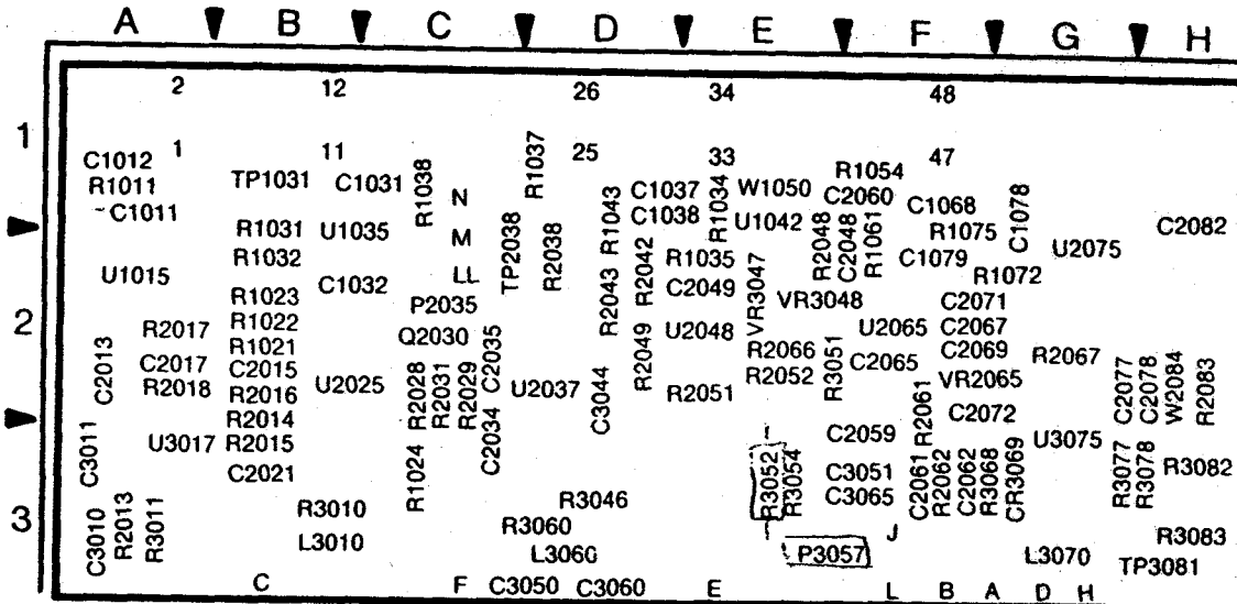
670-7921- Fig. 10-54. A50A4—Error Amplifier circuit board.
