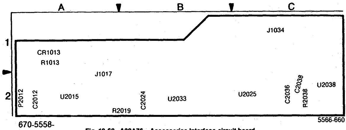
Fig. 10-60. A30A76—Accessories Interface circuit board.
