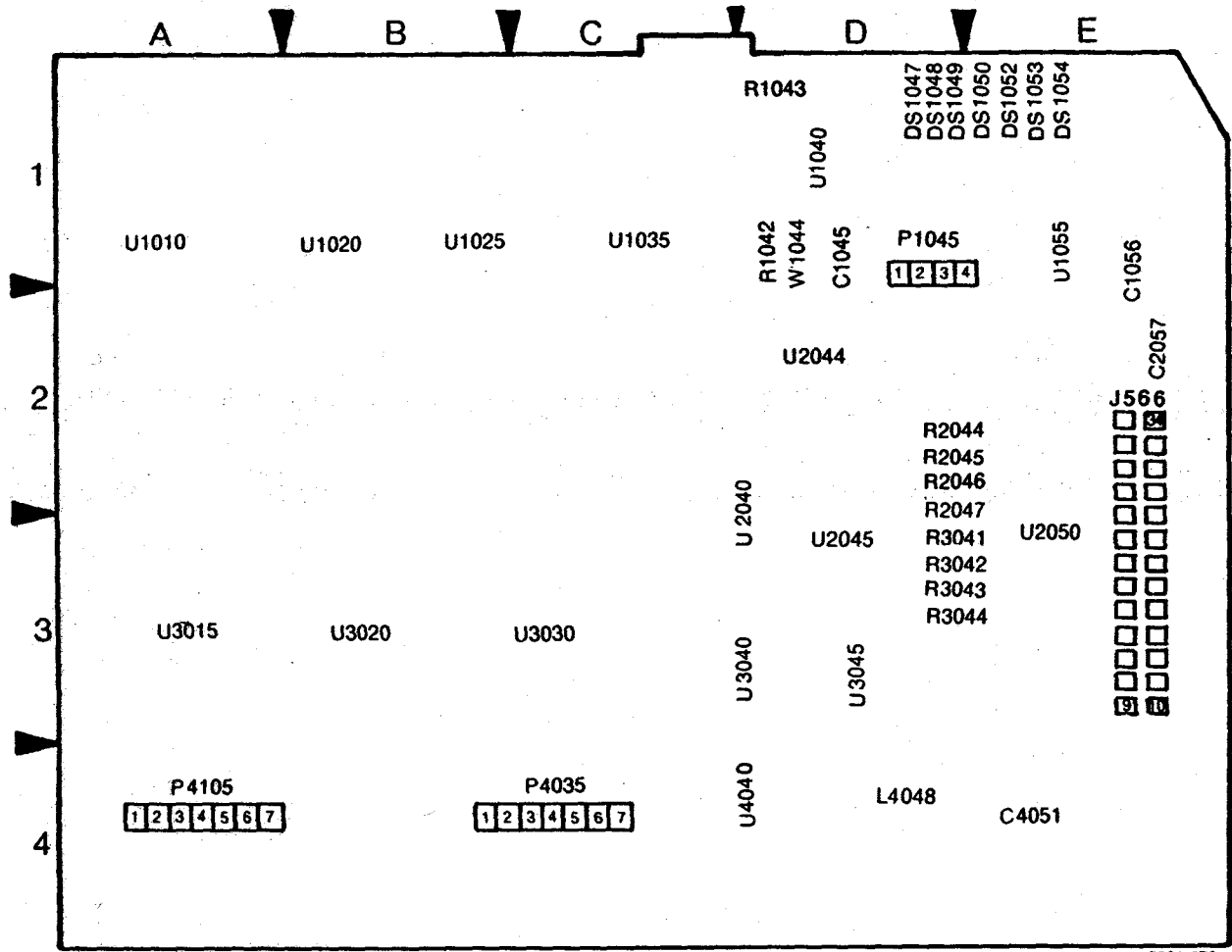
Fig. 10-58. A56—GPIB circuit board. (FRONT)
