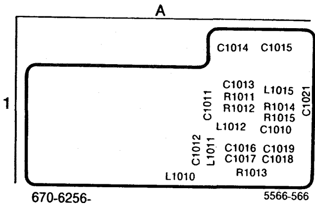
Figure 10-10. A23A4—829 MHz Diplexer circuit board.
