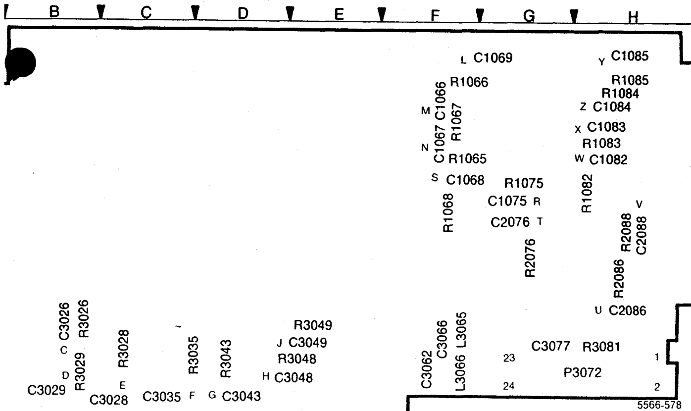
Figure 10-18. A68A1—VR Mother board #1 circuit board.
