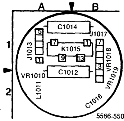
Figure 10-1. A16A1—1st LO Interface circuit board.
