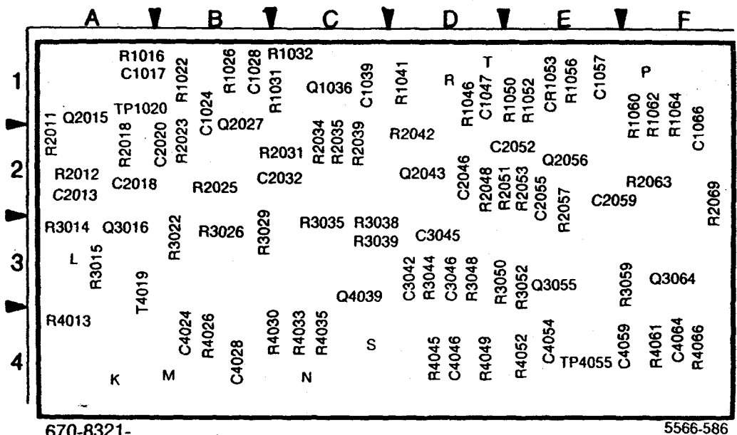
Fig. 10-29. A68A5—VR 10dB Gain Steps circuit board.
