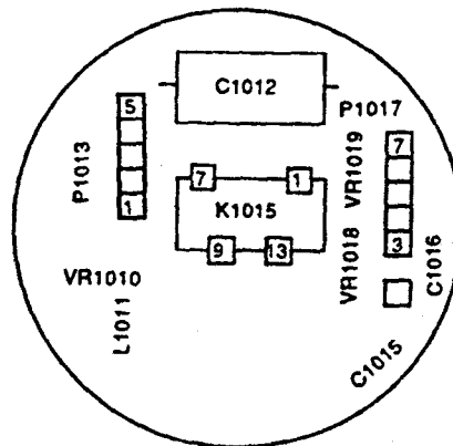
NEW A16A1 - 1ST LO Interface Circuit Board
