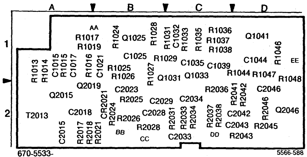
Fig. 10-31. A68A7—VR Band Leveling circuit board.
