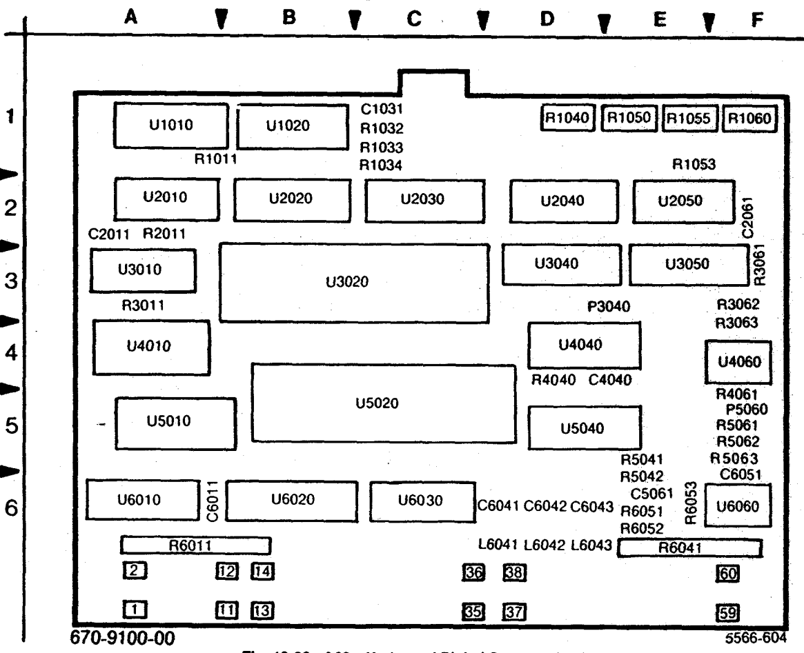
Fig. 10-38. A60—Horizontal Digital Storage circuit board.
