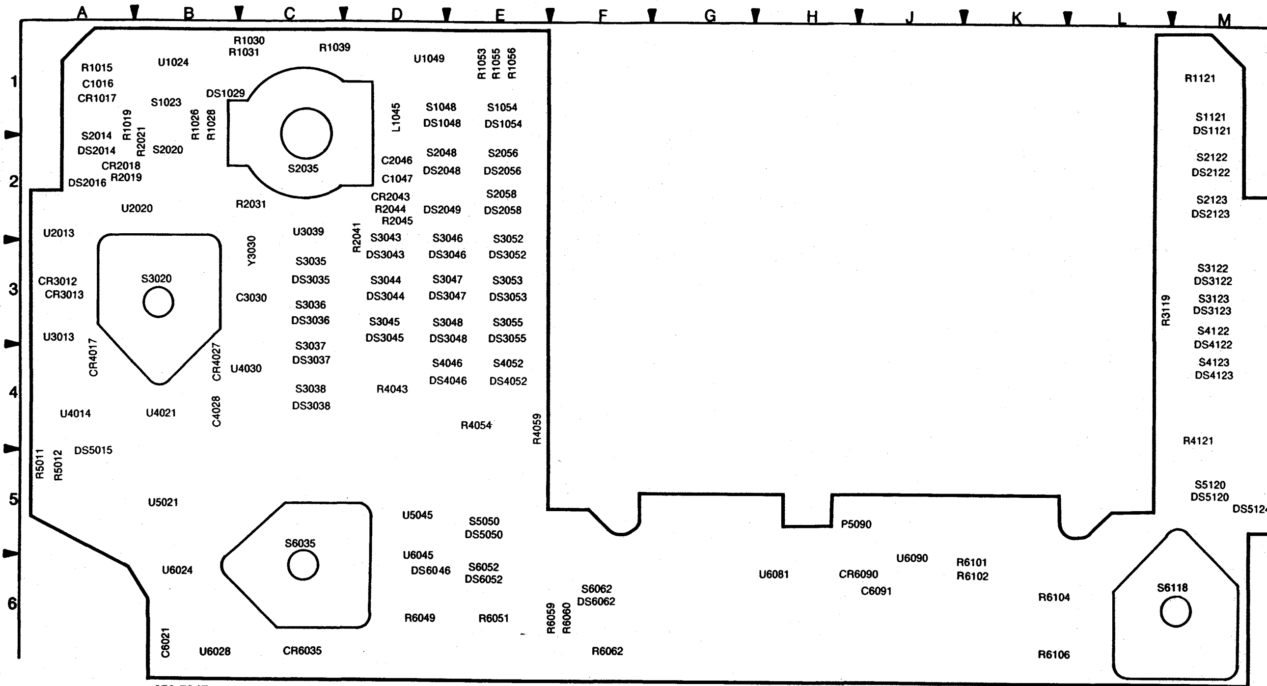
Fig. 10-61. A38—Front Panel circuit board.
