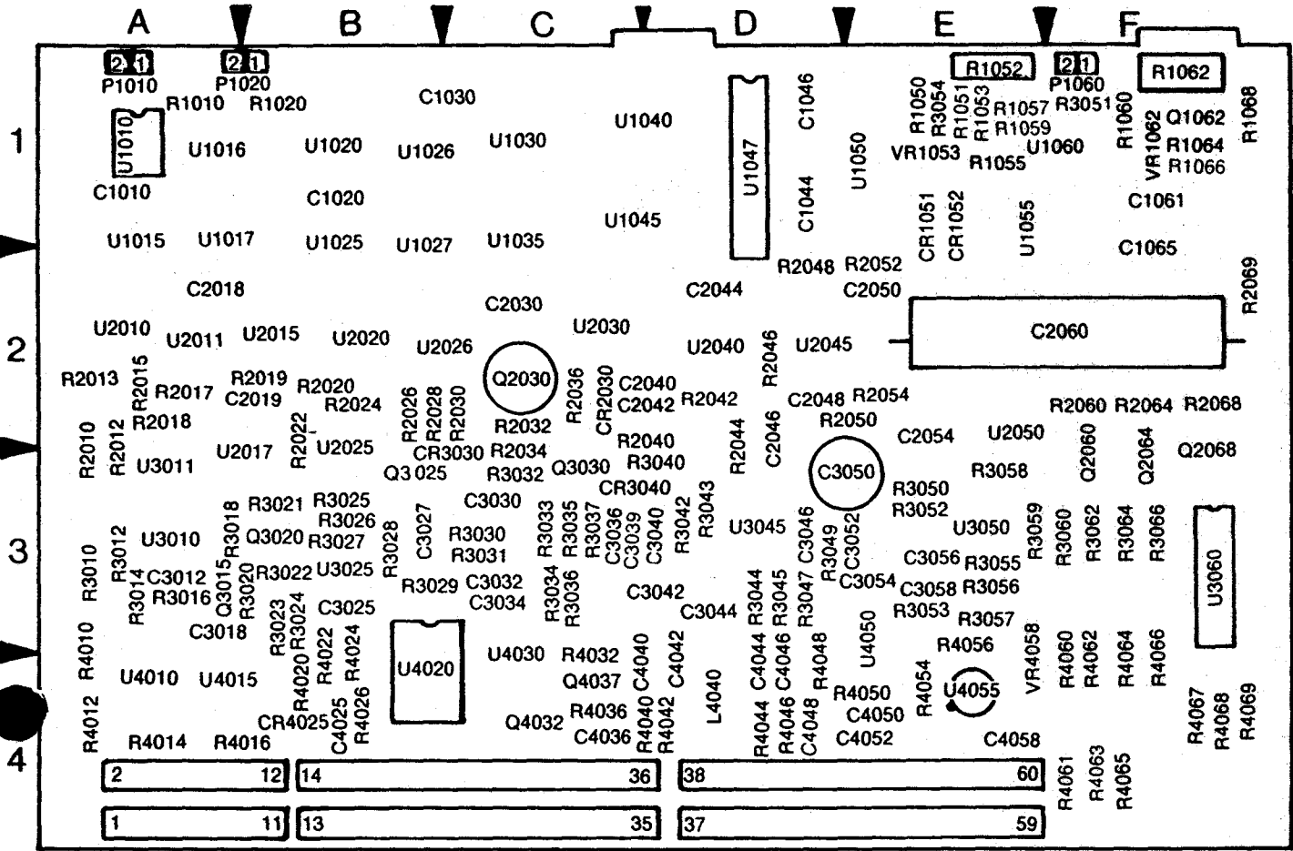
Fig. 10-43. A72—Sweep circuit board.
