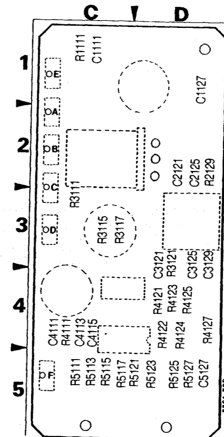
Fig. 10-26 A69A1 — 1st Mixer circuit board (rear)
