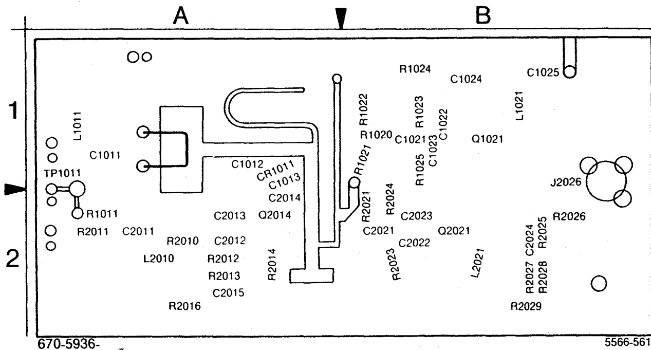
Figure 10-7. A23A1—719 MHz 2nd LO circuit board.
