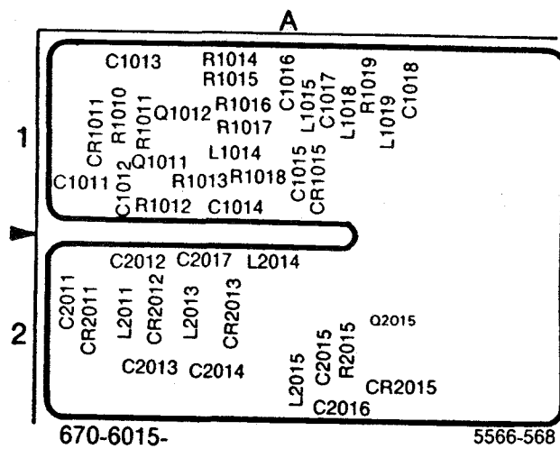
Figure 10-12. A23A6—110 MHz IF Select circuit board.
