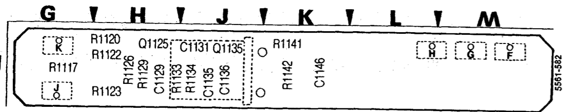
Fig. 10-28 A69A4 — Local Oscillator circuit board (rear)
