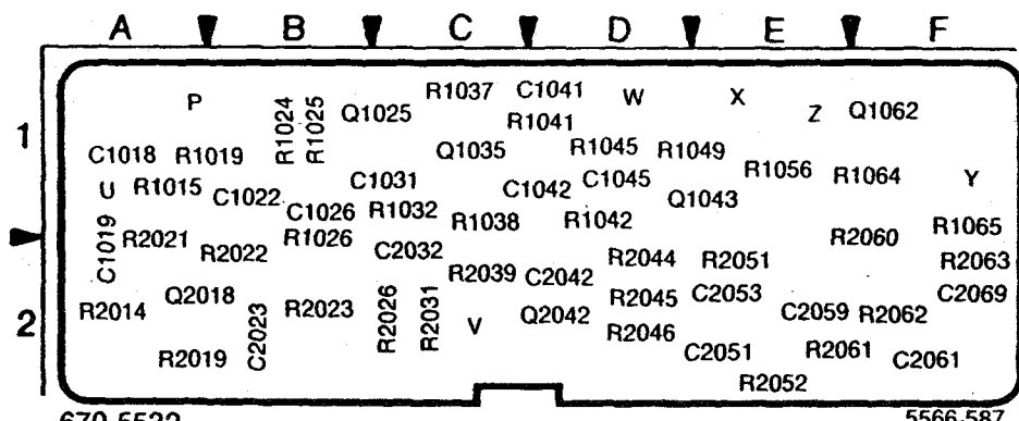
Fig. 10-30. A68A6—VR 20 dB Gain Steps circuit board.
