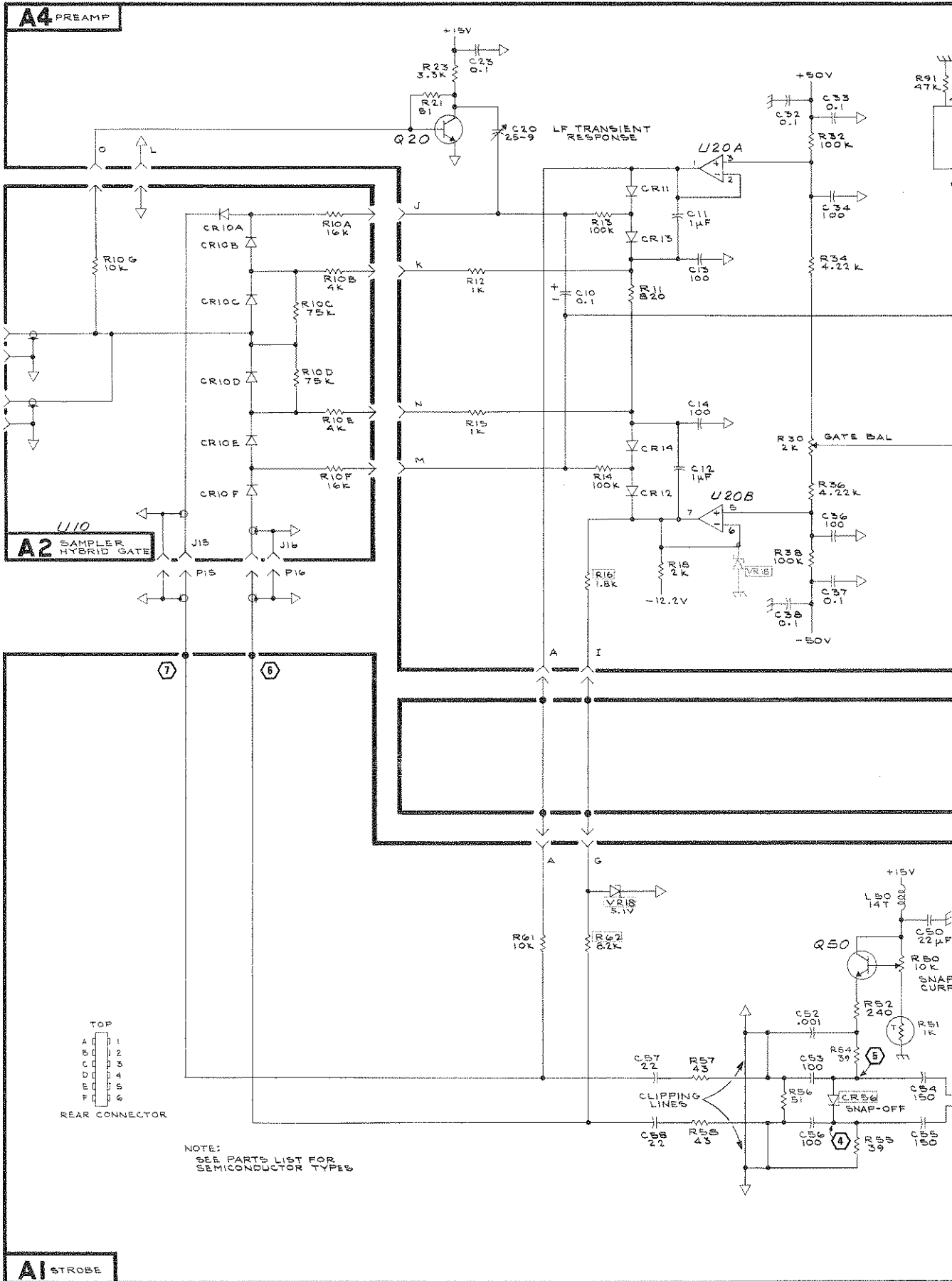
S6 SAMPLING HEAD
