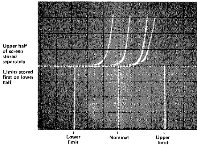
Fig. 35. Display of tolerance limits stored on lower screen and Zener characteristics stored in upper screen.
