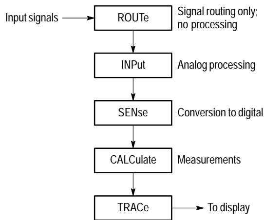
Figure 1–8: AM700 SCPI systems for measurements
