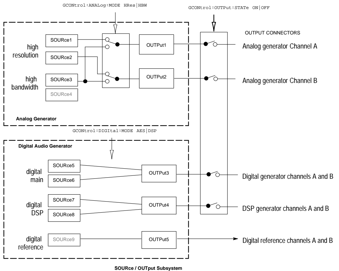
Figure 1-13: GCONtroll subsystem for the AM700 generator
