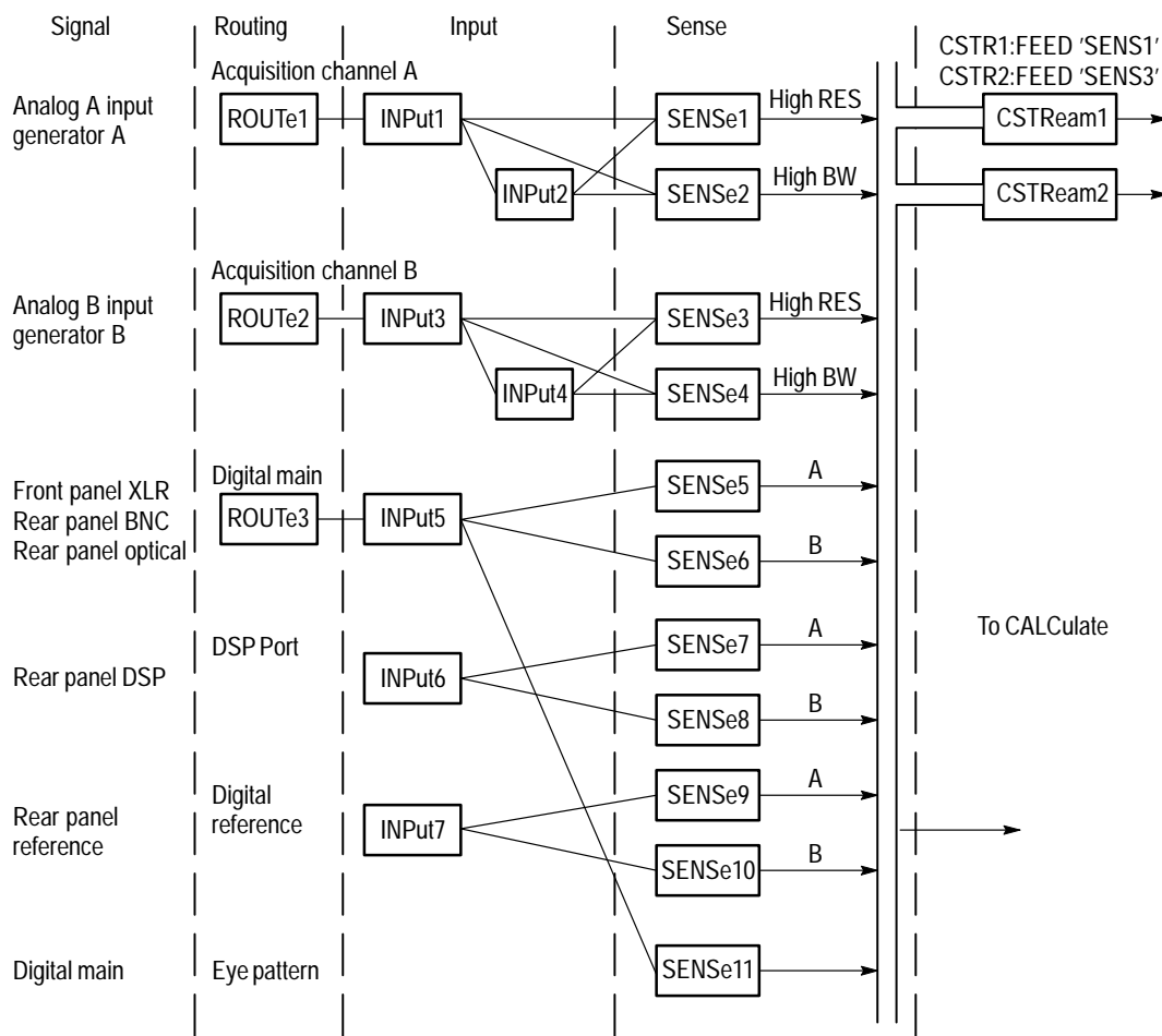
Figure 1-10: AM700 signal routing to CSTR1 and CSTR2
