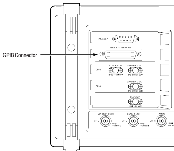
Figure 1-2: GPIB Connector
