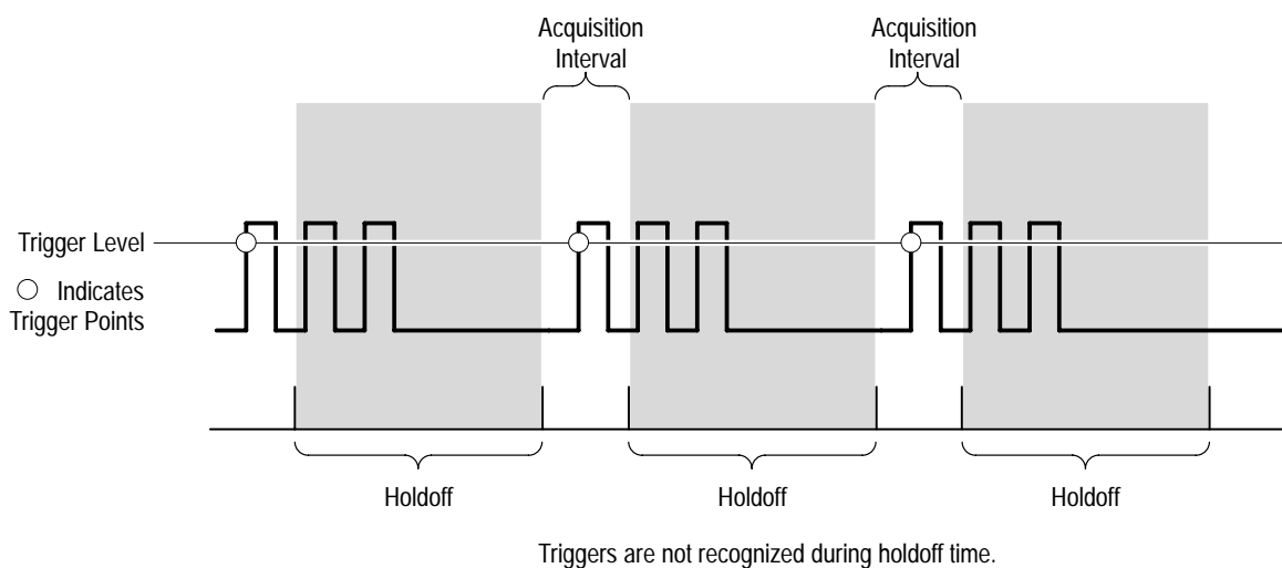
Figure 3–24: Trigger Holdoff Time Ensures Valid Triggering
