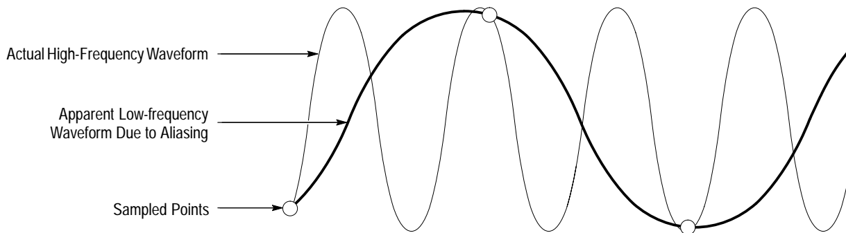
Figure 3–13: Aliasing
