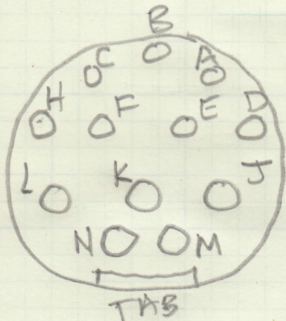
AM503X FRONT CONNECTOR VIEW
