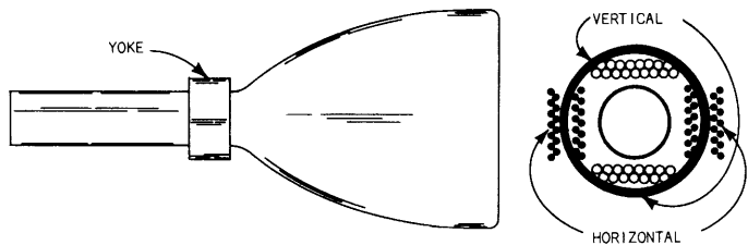
Fig. 6-25. Yoke position.
