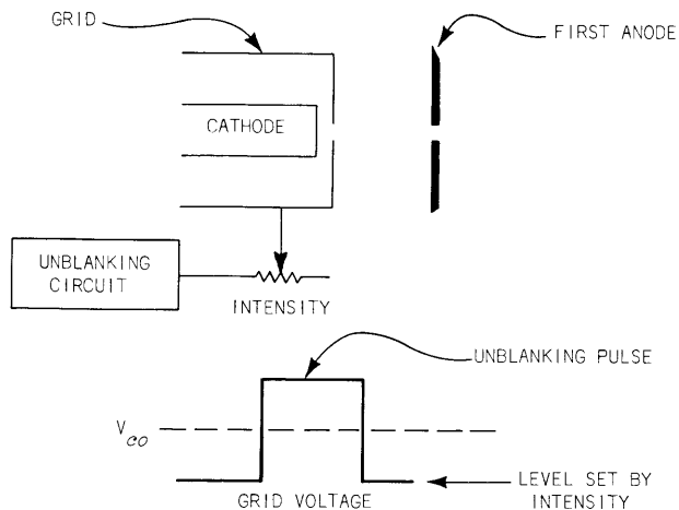
Fig. 4-1. Grid unblanking.
