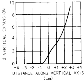
Fig. 6-15. T5470 single-ended deflection.
