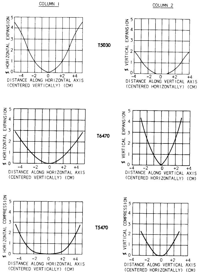
Fig. 6-14. Deflection-linearity characteristics.
