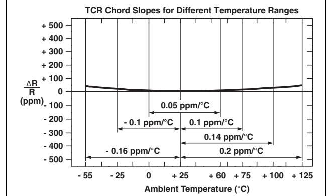
FIGURE 5 - TYPICAL RESISTANCE/TEMPERATURE CURVE (Z-FOIL)
