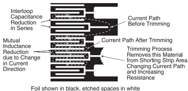
FIGURE 4 - TRIMMING TO VALUES (Conceptual Illustration)
