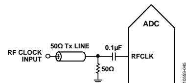
Figure 49. Typical RF Clock Input Circuit
