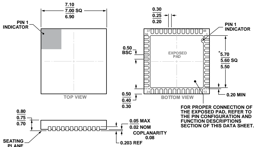
Figure 63. 48-Lead Lead Frame Chip Scale Package [LFCSP_WQ] 7 mm × 7 mm Body, Very Very Thin Quad (CP-48-13) Dimensions shown in millimeters
