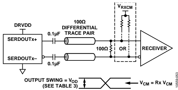
Figure 57. AC-Coupled Digital Output Termination Example
