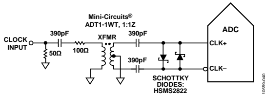
Figure 44. Transformer-Coupled Differential Clock (Up to 200 MHz)
