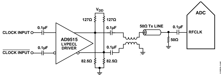
Figure 50. Differential PECL RF Clock Input Circuit
