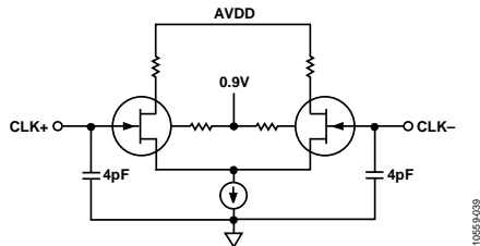
Figure 43. Equivalent Nyquist Clock Input Circuit
