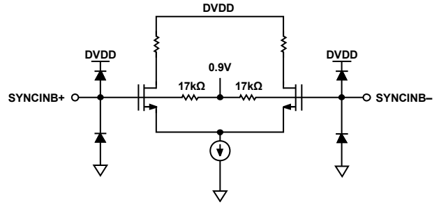
Figure 37. SYNCINB± Circuit
