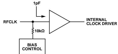
Figure 48. Equivalent RF Clock Input Circuit
