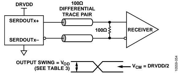
Figure 58. DC-Coupled Digital Output Termination Example
