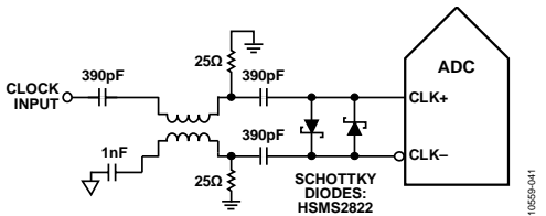
Figure 45. Balun-Coupled Differential Clock (Up to 625 MHz)
