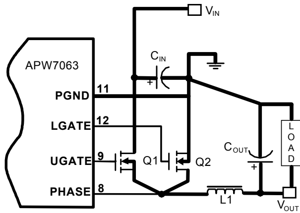
Figure 8. Recommended Layout Diagram
