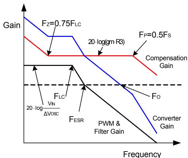
Figure 6. Converter Gain & Frequency
