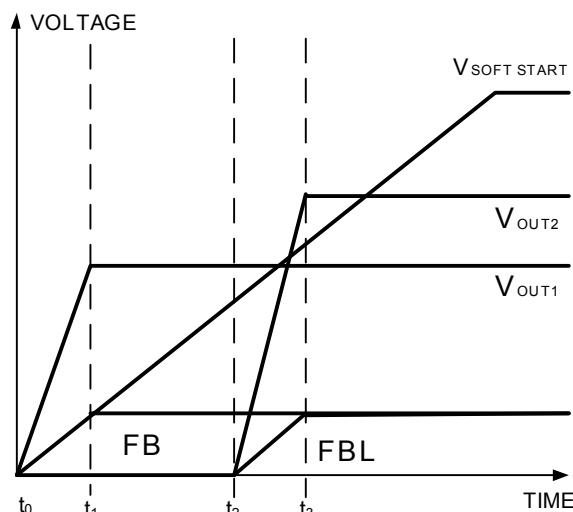
Figure 1. Soft-Start Interval
