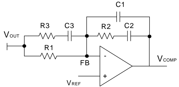
Figure 12. Compensation Network
