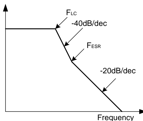
Figure 10. The LC Filter Gain & Frequency
