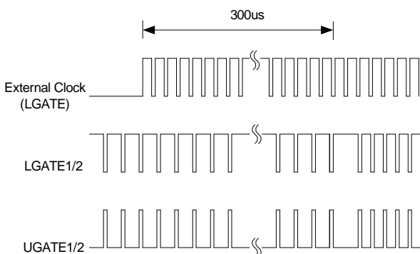
Figure 8. The timing chart of synchronization function
