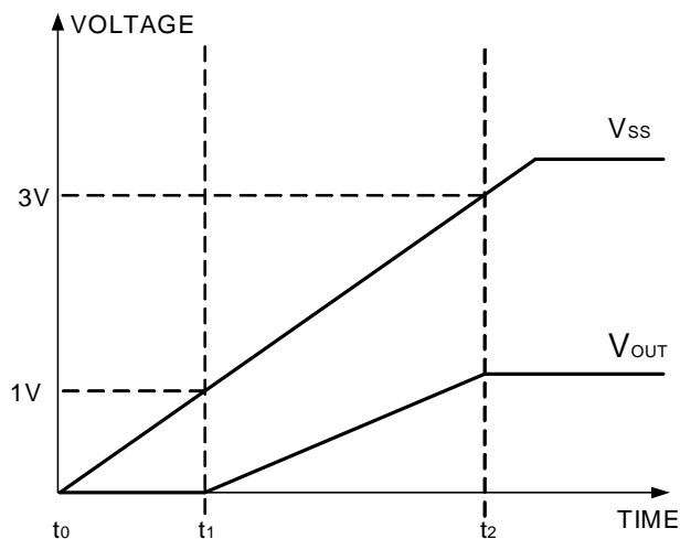
Figure 4. Soft-Start Interval
