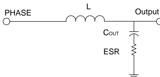
Figure 9. The Output LC Filter
