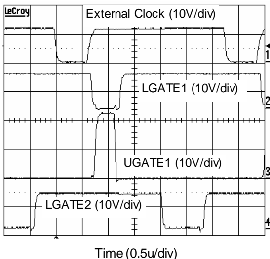
Figure7. The switching timing of synchronization function
