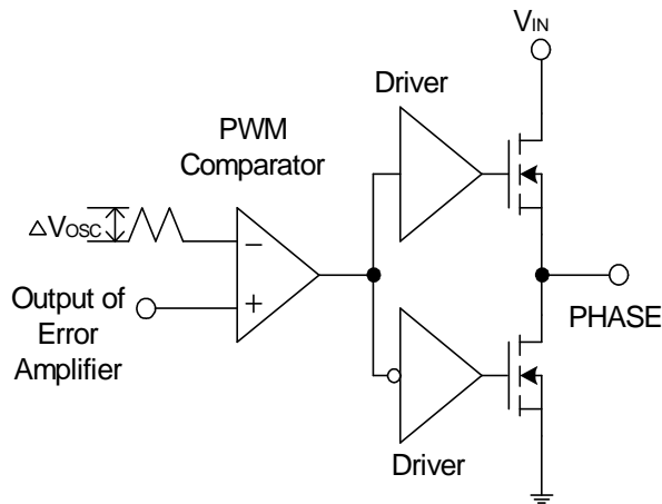
Figure 11. The PWM Modulator
