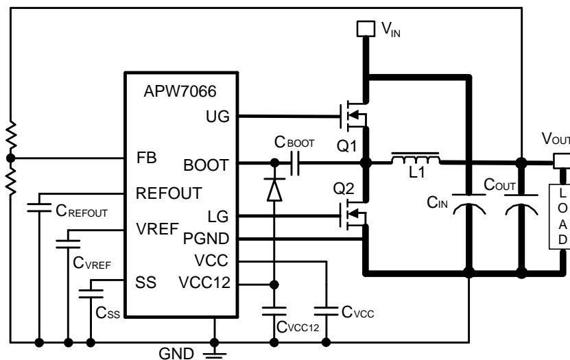
Figure 14. Layout Guidelines
