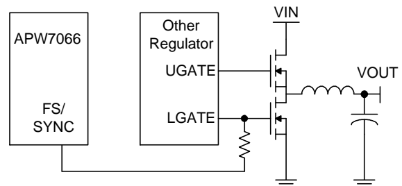
Figure 6. Connecting the LGATE signal from other regulator to FS/SYNC pin
