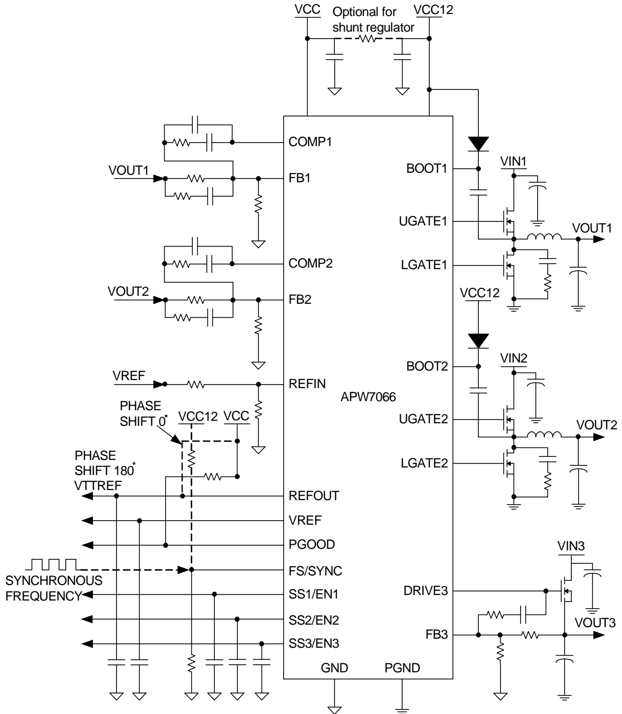
APW7066 INDEPENDENT MODE
