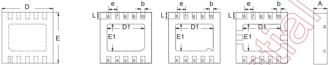
Top view
