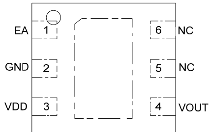
Figure 3a TDFN6-2x2 Package
