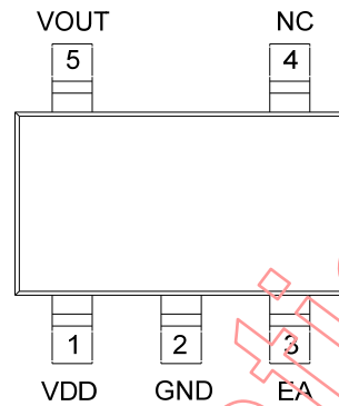
Figure 3b SOT-23-5, SOT-353 Package
