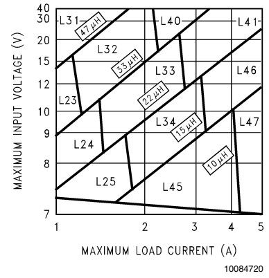
FIGURE 4. LM2679-5.0
