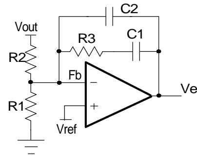
Figure 8 - Type II compensator
