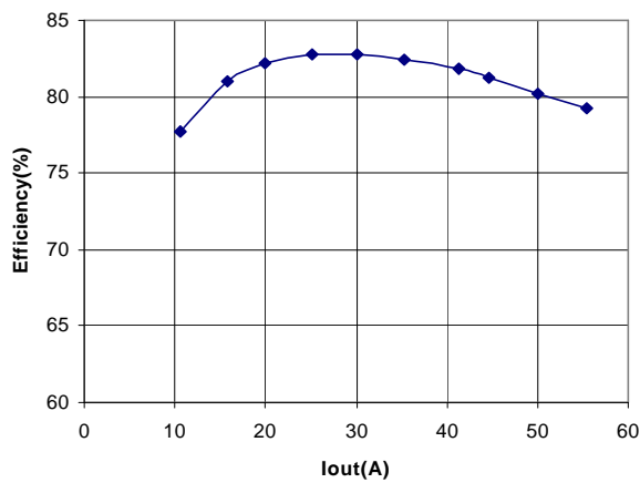
Figure 7: Efficiency
