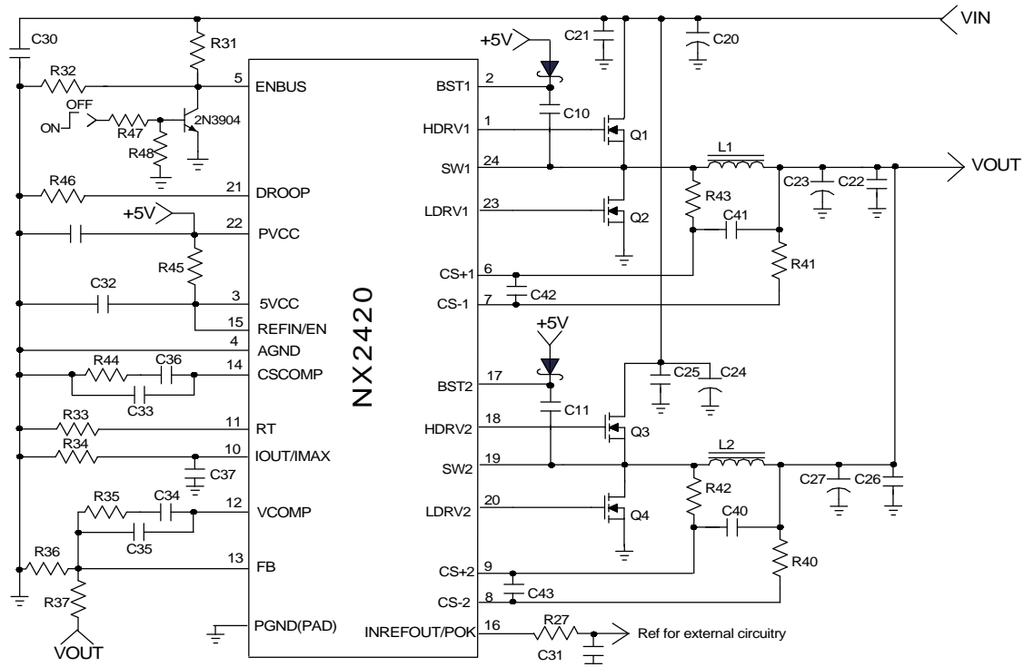
Figure1 - Typical application of NX2420
