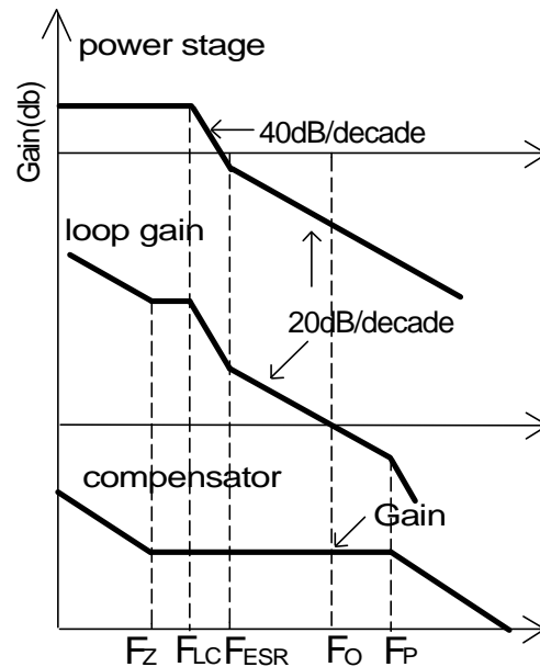
Figure 9 - Bode plot of Type II compensator
