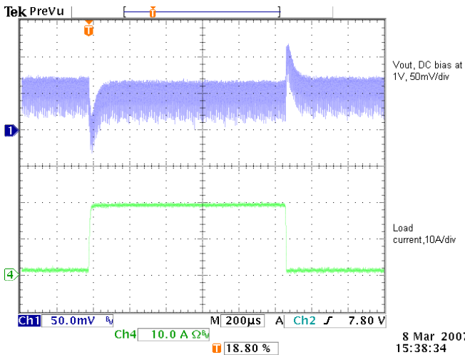
Figure 5 - Transient response
