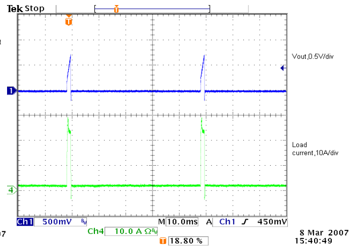
Figure 6 - Over current protection
