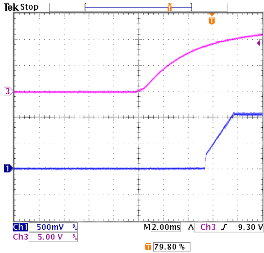
Figure 3 - Start up
