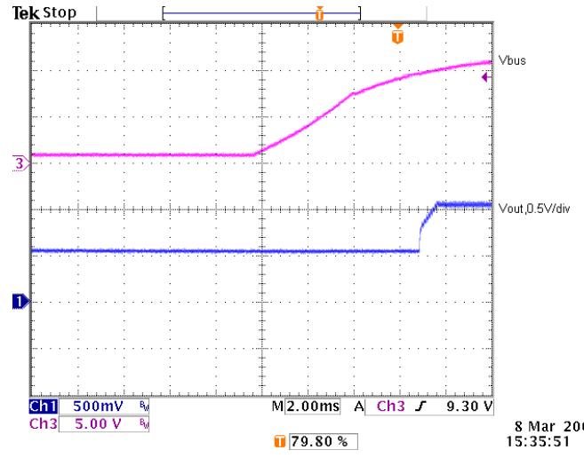
Figure 4 - Prebias start up
