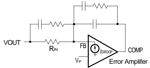
Figure 18 - Output voltage droop function
