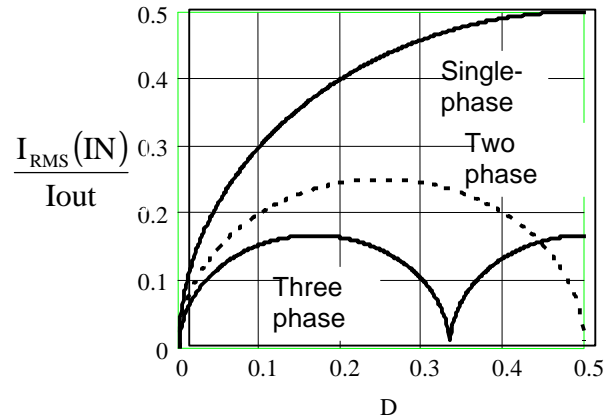
Figure 19 - Normalized input RMS current vs. duty cycle.
