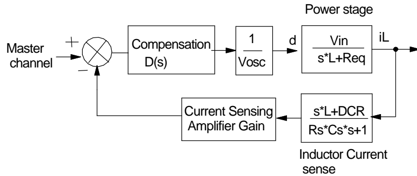
Figure 12 - Current loop control diagram
