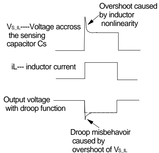
Figure 15 - Droop accuracy affected by the nonlinearity of inductor.
