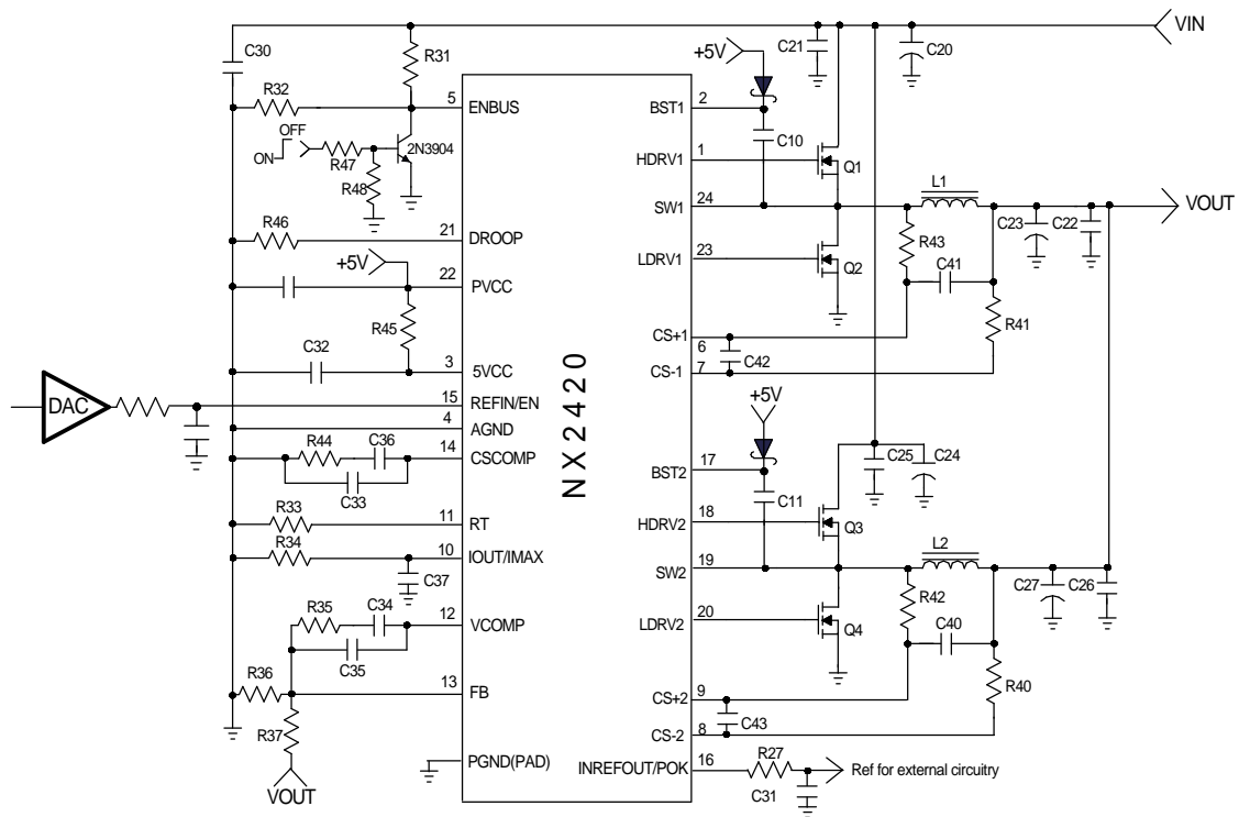
Figure 20 - Typical application of NX2420 with external reference
