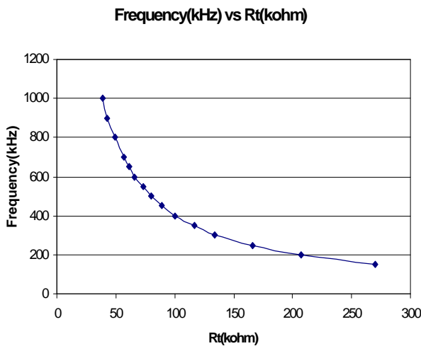
Figure 17 - Frequency vs R_t chart
