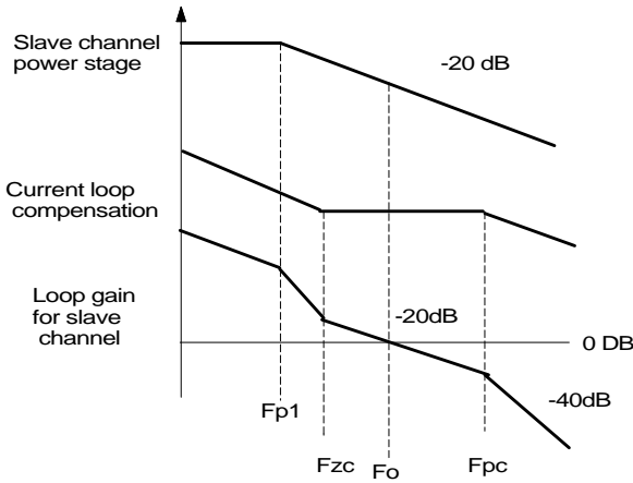
Figure 16 - Bode plot of current loop
