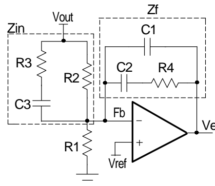
Figure 10 - Type III compensator
