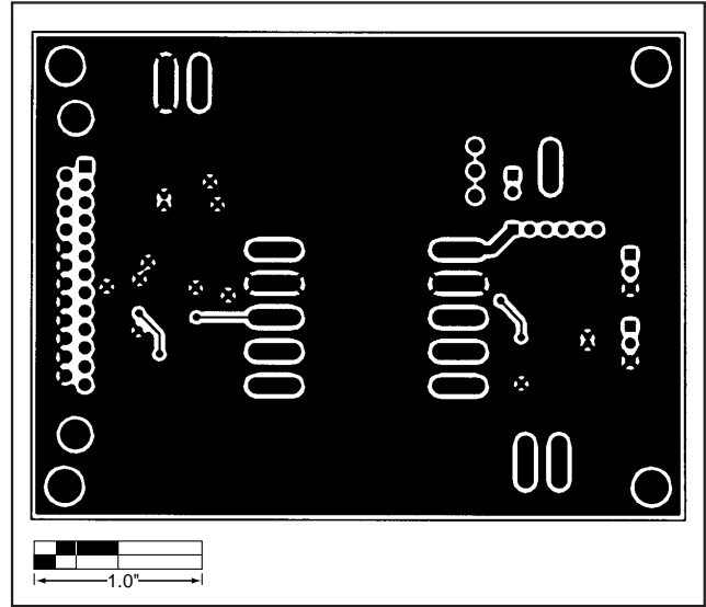
Figure 4. MAX1617 EV Kit PC Board Layout—Solder Side
