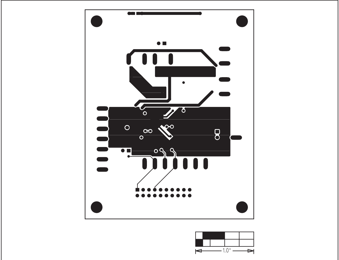
Figure 8. MAX17088 EV Kit PCB Layout—Solder Side
