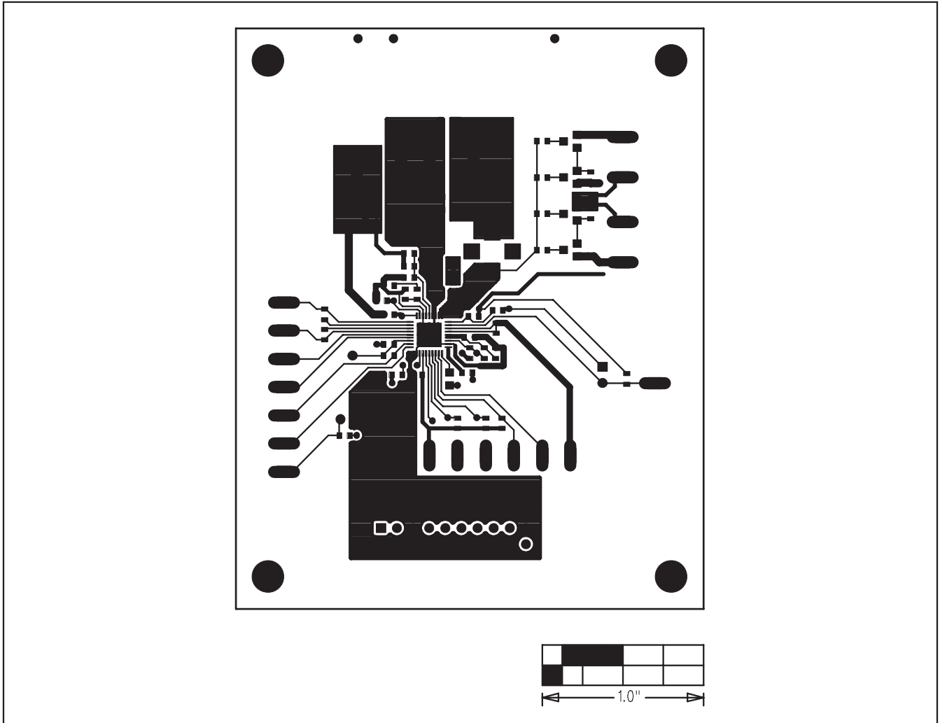
Figure 5. MAX17088 EV Kit PCB Layout—Component Side
