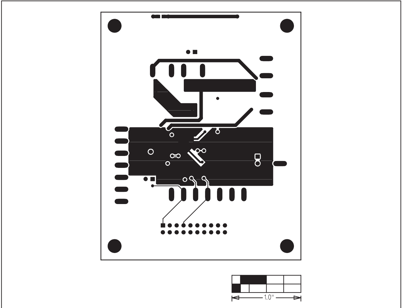
Figure 7. MAX17088 EV Kit PCB Layout—Layer 3
