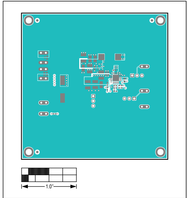
MAX17504EVKITBE# PCB Layout—Top Layer
