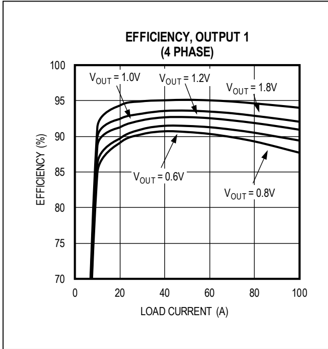
Figure 8. Output 1 Efficiency
