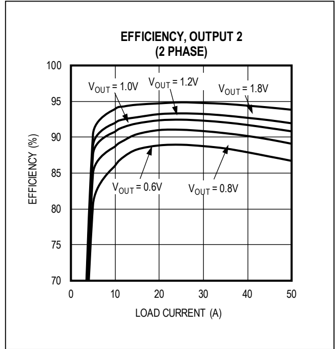
Figure 9. Output 2 Efficiency
