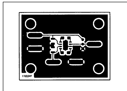
Figure 3. PC Board Layout—Component Side
