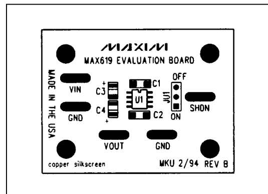
Figure 2. Component Placement Guide—Component Side
