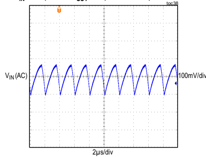
MAXM15464 INPUT VOLTAGE RIPPLE V_{IN} = 24V , FIXED V_{OUT} = 5V , FULL LOAD, PWM MODE
