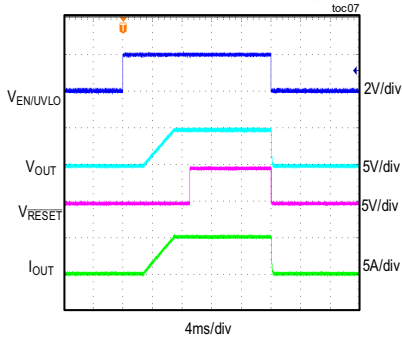
POWER-UP AND DOWN THROUGH EN/UVLO (VIN = 24V, VOUT = 5V, IOUT = 5A PWM MODE, MODE = SGND)
