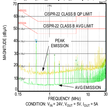
CONDUCTED EMISSION PLOT (WITH FILTER C18 = 4.7µF, L1 = 8.2µH, C19 = C20 = C21 = C22 = 4.7µF, C23 = 0.1µF, C1 = 220pF)
