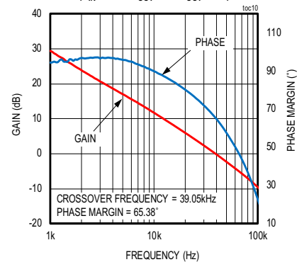
BODE PLOT (VIN = 24V, VOUT = 5V, IOUT = 5A)
