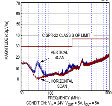
RADIATED EMISSION PLOT (NO FILTER C18 = OPEN, L1 = SHORT, C19 = C20 = C21 = C22 = C23 = C1 = OPEN)
