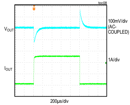
LOAD TRANSIENT (VIN = 24V, VOUT = 5V, IOUT = 0A TO 2.5A PWM MODE, MODE = SGND)
