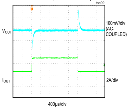
LOAD TRANSIENT (VIN = 24V, VOUT = 5V, IOUT = 2.5A TO 5A PWM MODE, MODE = SGND)
