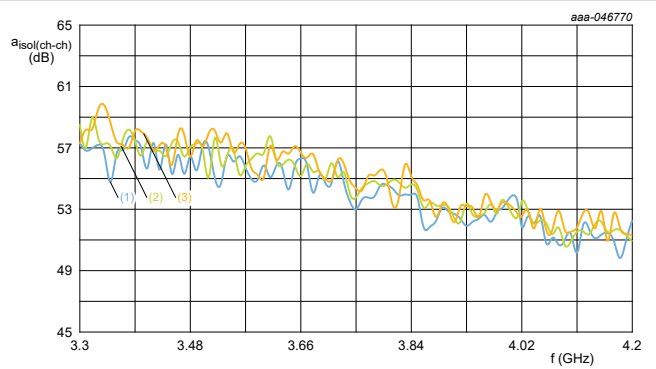
Figure 19. Low gain RX mode, Channel Isolation versus frequency
