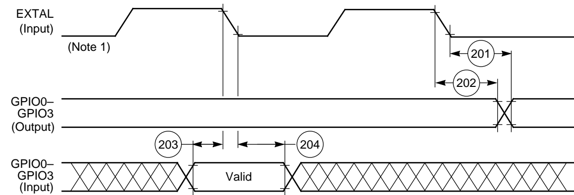
Figure 2-22 GPIO Timing
