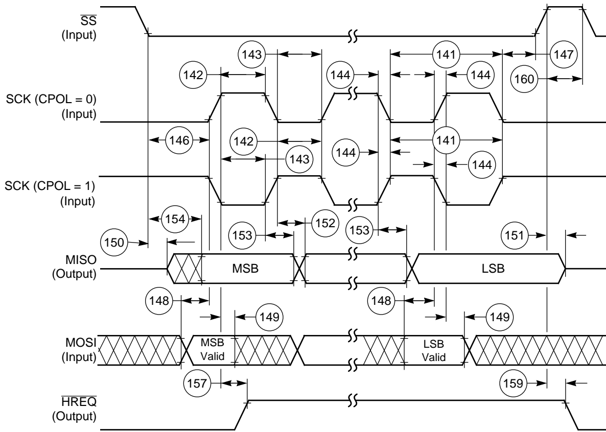
Figure 2-19 SPI Slave Timing (CPHA = 0)
