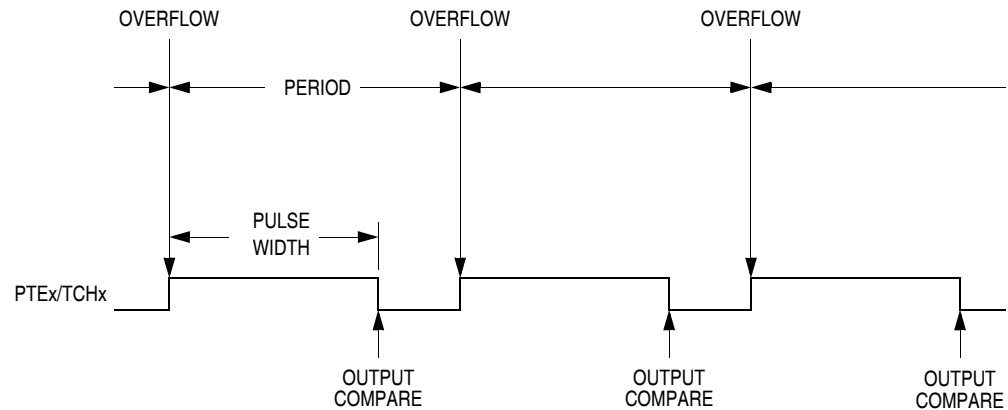
Figure 25-2. PWM Period and Pulse Width
