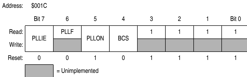
Figure 8-3. PLL Control Register (PCTL)
