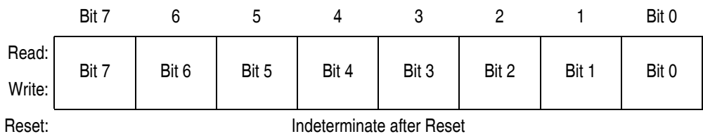
Figure 18-8. TIMA Channel Registers (TACH0H/L–TACH3H/L) (Sheet 2 of 2)
