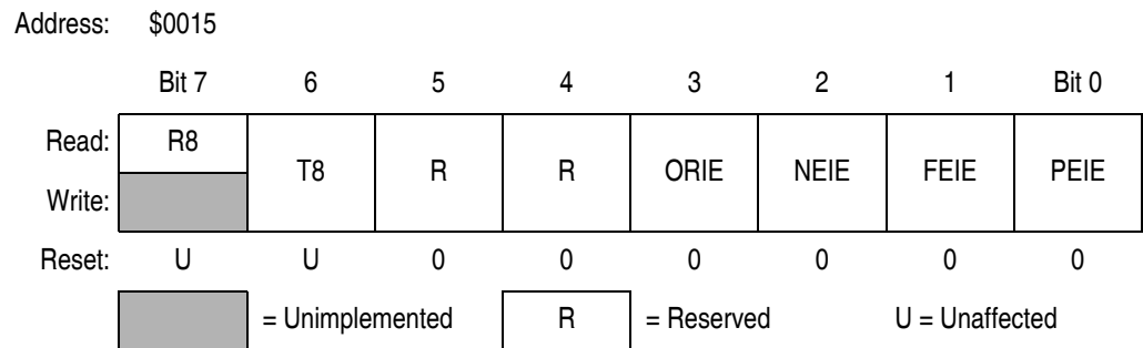
Figure 16-10. SCI Control Register 3 (SCC3)
