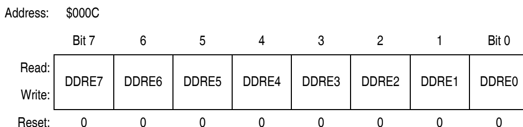
Figure 22-14. Data Direction Register E (DDRE)
