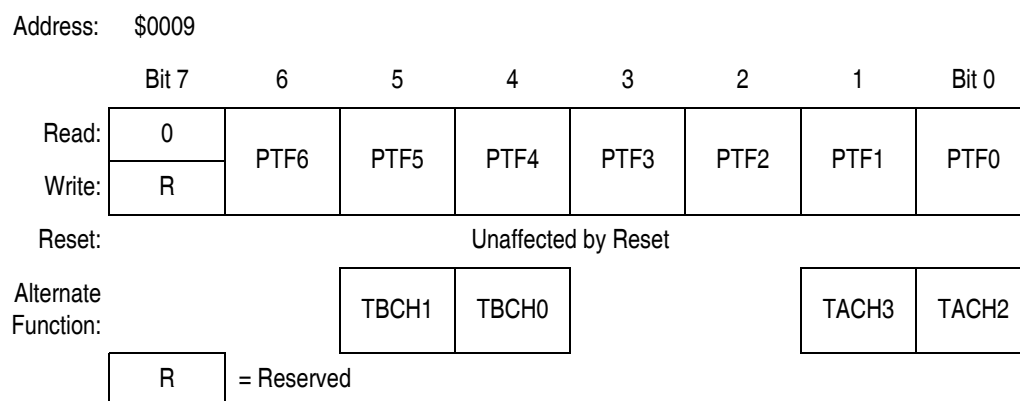
Figure 22-16. Port F Data Register (PTF)
