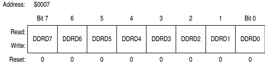
Figure 22-11. Data Direction Register D (DDRD)
