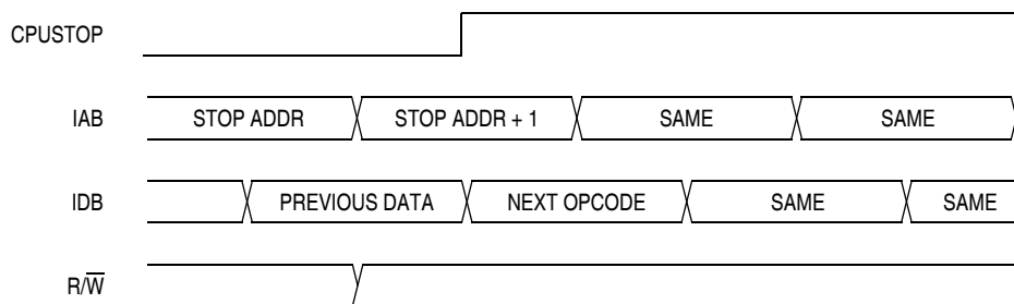
Figure 7-14. Stop Mode Entry Timing
