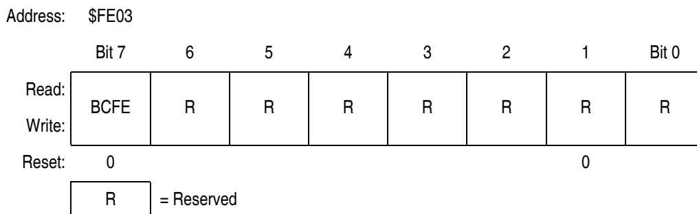
Figure 7-18. SIM Break Flag Control Register (SBFCR)
