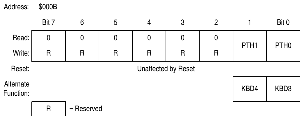
Figure 22-22. Port H Data Register (PTH)
