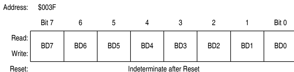
Figure 28-20. BDLC Data Register (BDR)
