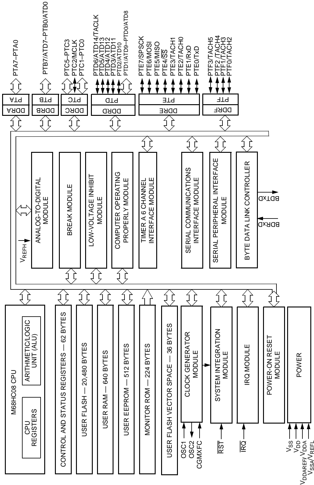
Figure 1-2. MCU Block Diagram for the MC68HC08AS20 Emulator (52-Pin PLCC)
