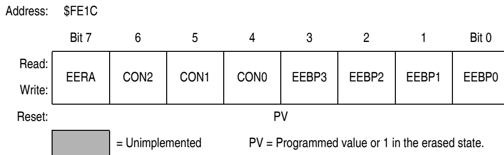
Figure 5-2. EEPROM Nonvolatile Register (EENVR)
