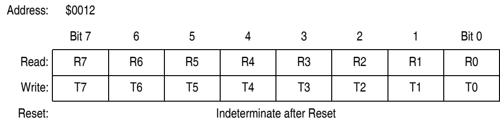
Figure 17-13. SPI Data Register (SPDR)
