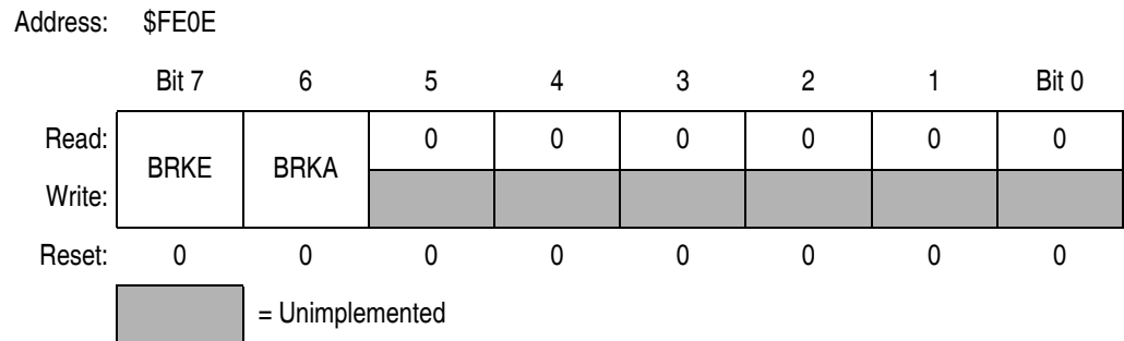
Figure 11-2. Break Status and Control Register (BSCR)
