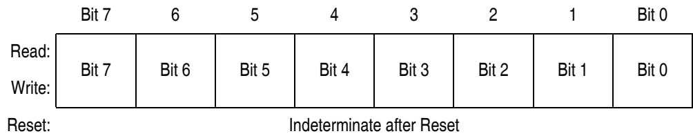
Figure 25-8. TIMA Channel Registers (TACH0H/L–TACH3H/L) (Sheet 3 of 3)
