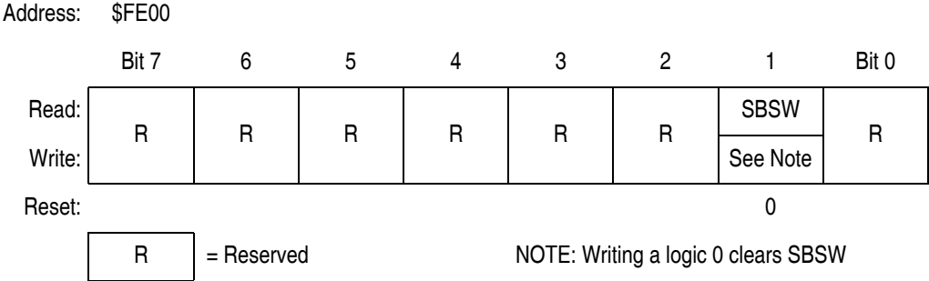
Figure 7-16. SIM Break Status Register (SBSR)
