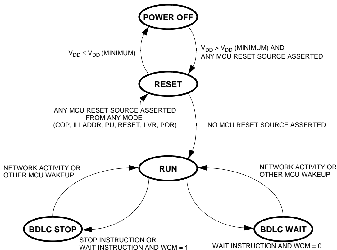
Figure 28-2. BDLC Operating Modes State Diagram
