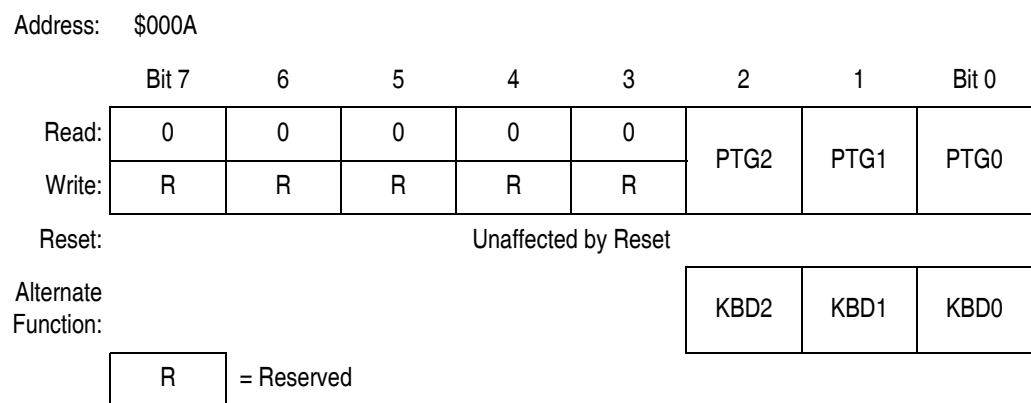
Figure 22-19. Port G Data Register (PTG)
