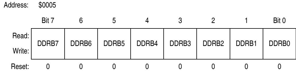
Figure 22-5. Data Direction Register B (DDRB)
