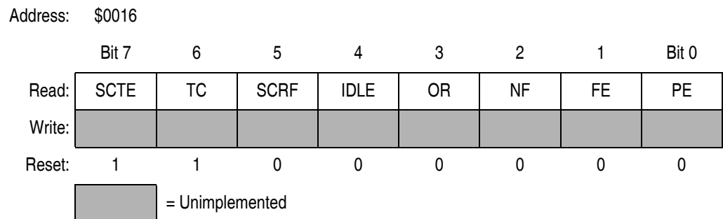
Figure 16-11. SCI Status Register 1 (SCS1)
