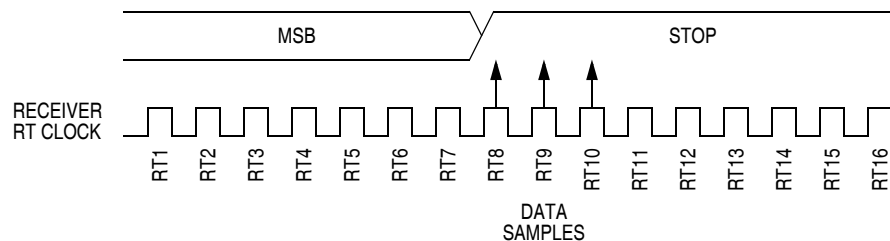
Figure 16-6. Slow Data
