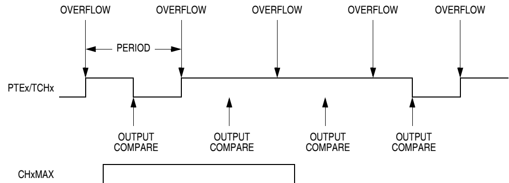
Figure 18-7. CHxMAX Latency
