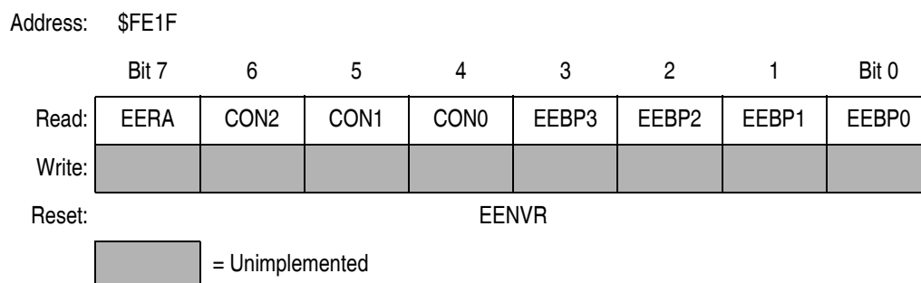
Figure 5-3. EEPROM Array Control Register (EEACR)
