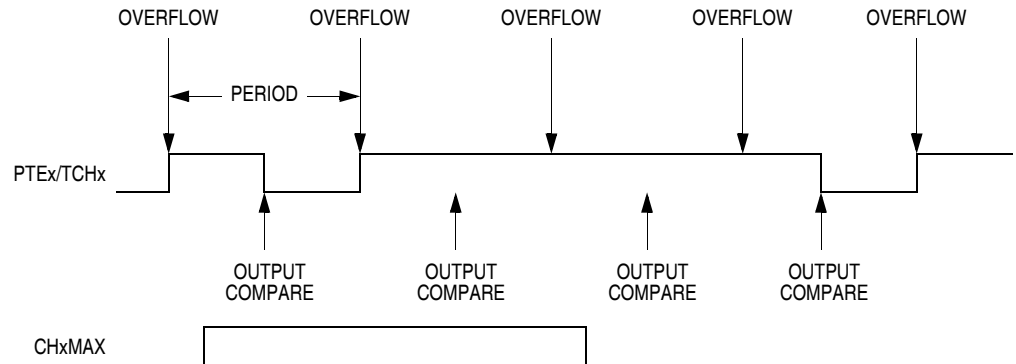
Figure 25-7. CHxMAX Latency
