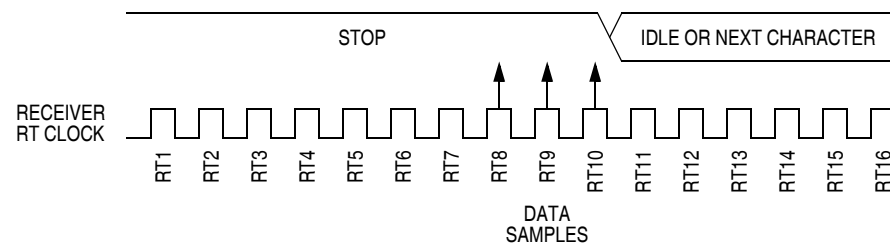
Figure 16-7. Fast Data
