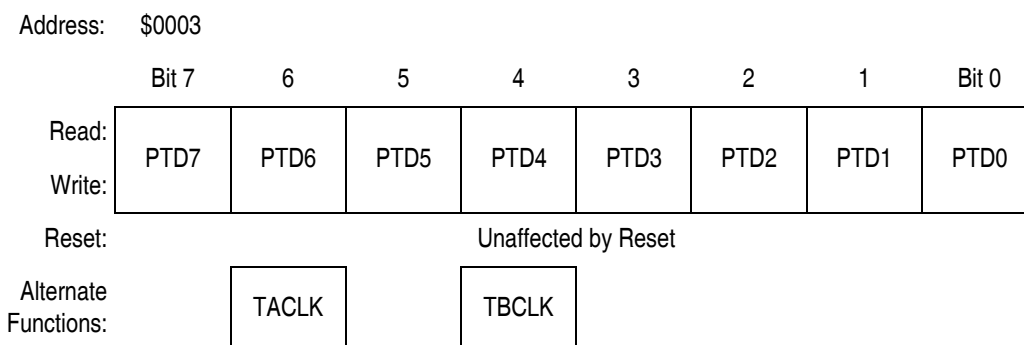
Figure 22-10. Port D Data Register (PTD)
