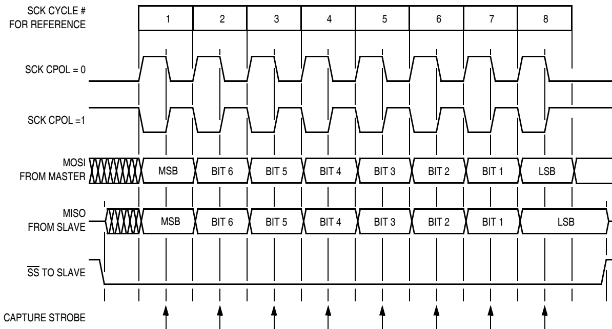
Figure 17-4. Transmission Format (CPHA = 1)
