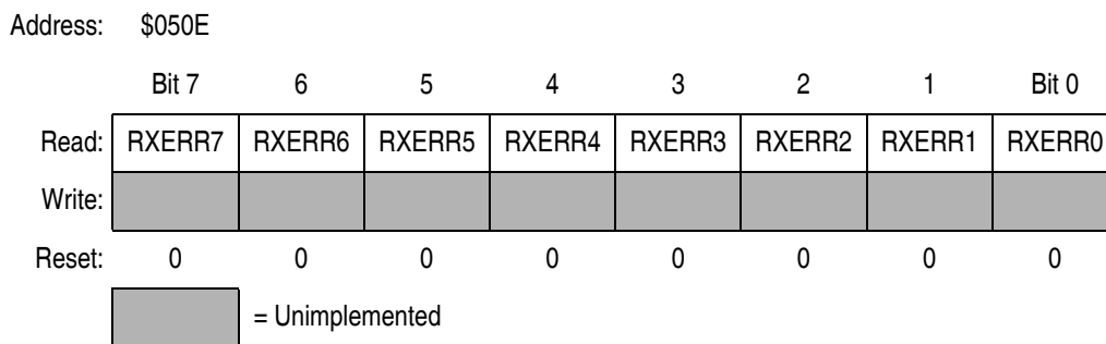
Figure 23-24. Receiver Error Counter (CRXERR)
