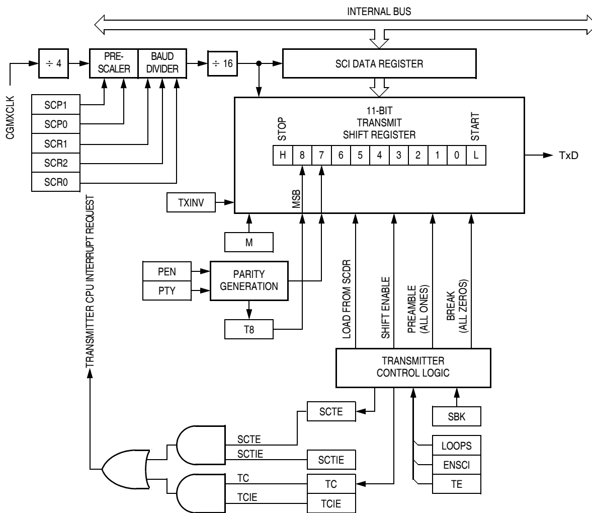
Figure 16-3. SCI Transmitter
