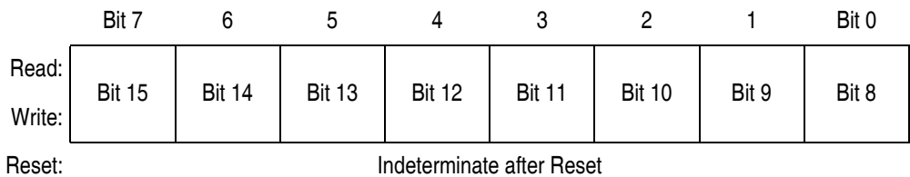
Figure 25-8. TIMA Channel Registers (TACH0H/L–TACH3H/L) (Sheet 1 of 3)
