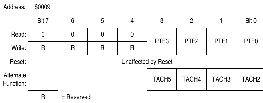
Figure 27-16. Data Direction Register E (DDRE)
