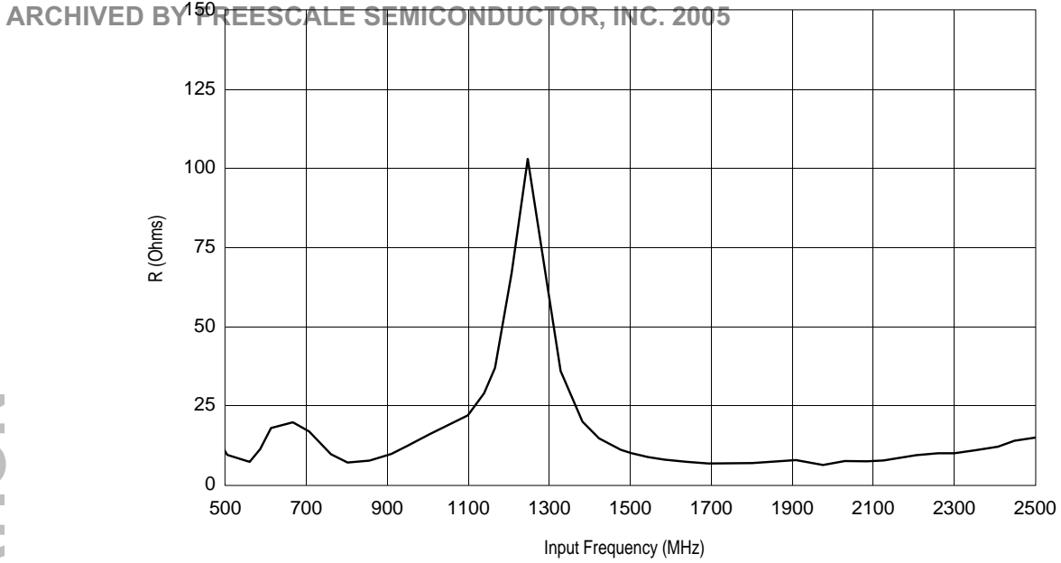
Figure 4. Input Impedance versus Frequency
