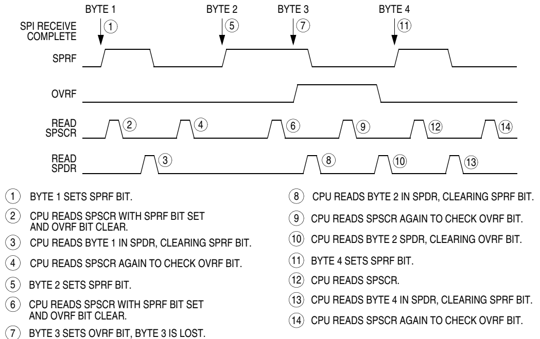
Figure 16-11. Clearing SPRF When OVRF Interrupt Is Not Enabled
