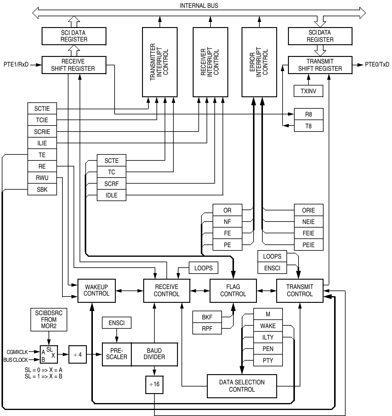
Figure 14-3. SCI Module Block Diagram
