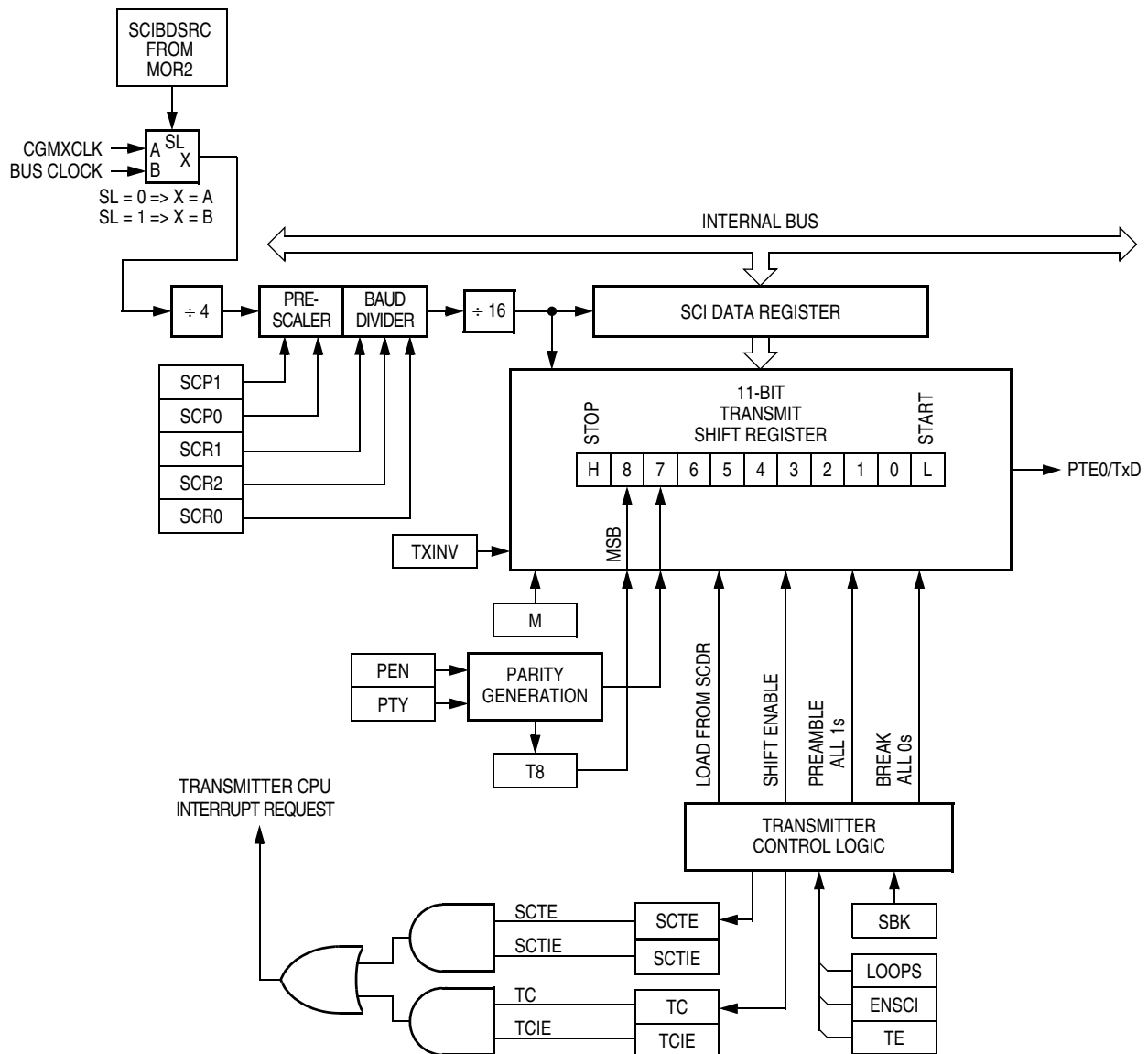
Figure 14-5. SCI Transmitter
