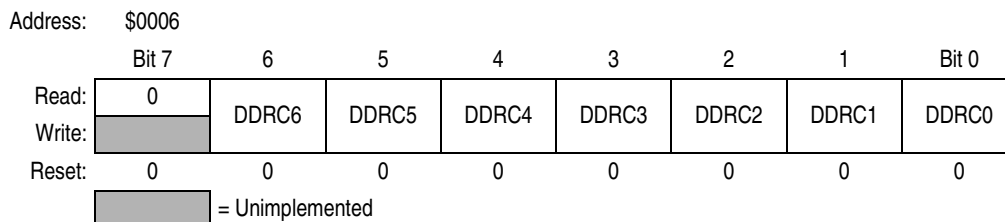
Figure 12-10. Data Direction Register C (DDRC)
