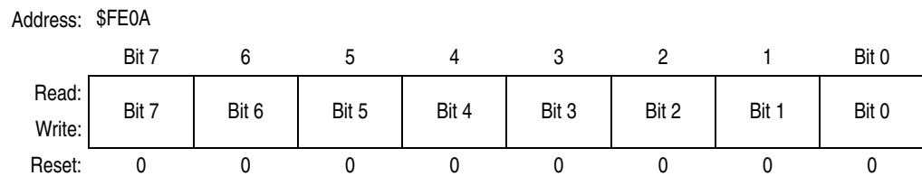
Figure 19-5. Break Address Register Low (BRKL)
