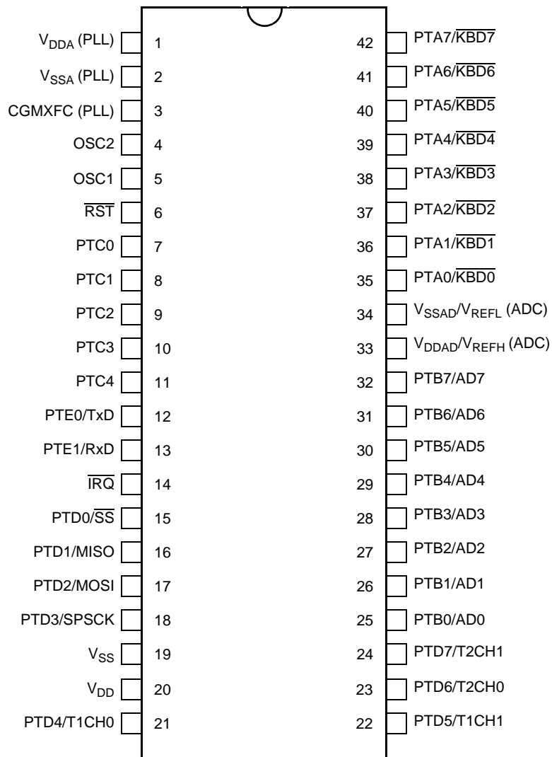
Figure 1-2. 42-Pin SDIP Pin Assignments
