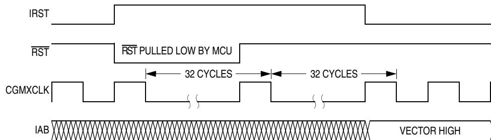
Figure 15-6. Internal Reset Timing
