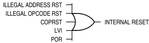
Figure 15-7. Sources of Internal Reset
