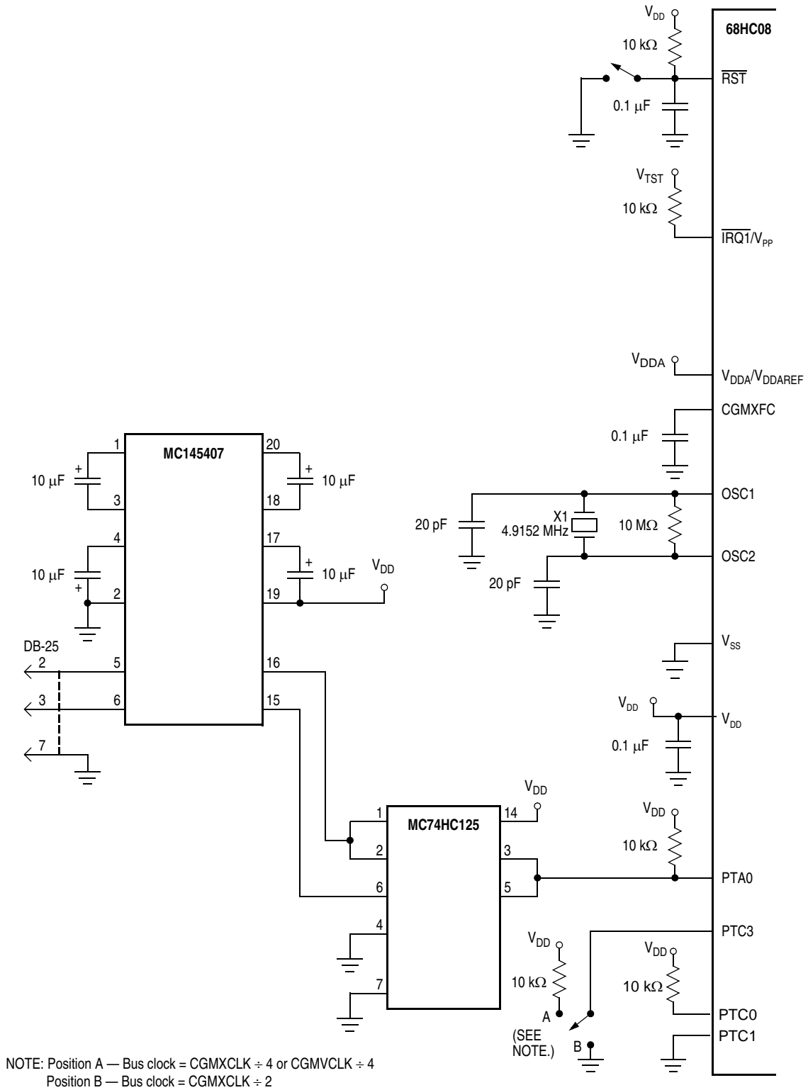
Figure 19-8. Monitor Mode Circuit
