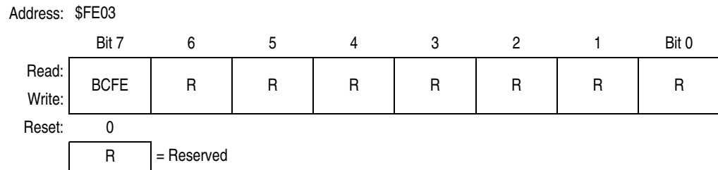
Figure 19-7. Break Flag Control Register (BFCR)
