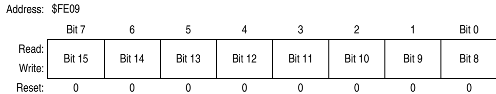
Figure 19-4. Break Address Register High (BRKH)
