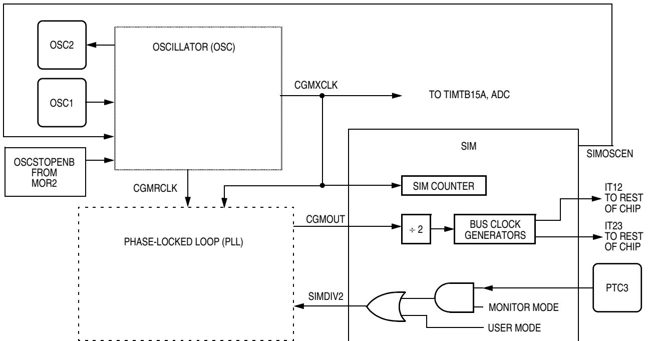
Figure 15-4. CGM Clock Signals
