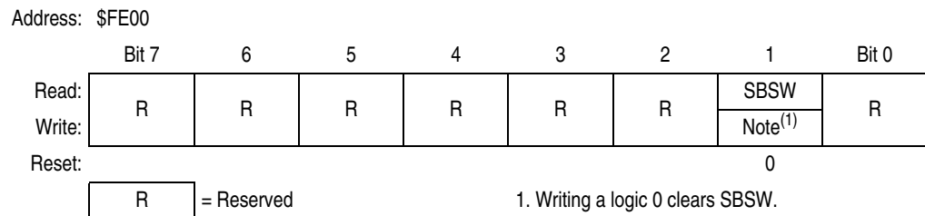
Figure 19-6. Break Status Register (BSR)
