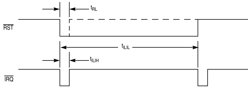
Figure 20-1. \overline{\text{RST}} and \overline{\text{IRQ}} Timing
