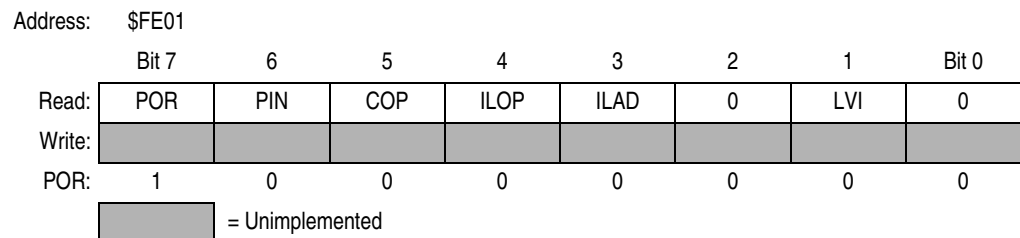
Figure 13-3. SIM Reset Status Register (SRSR)
