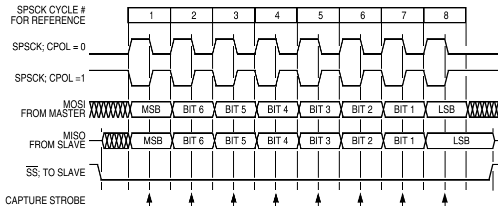
Figure 16-7. Transmission Format (CPHA = 1)
