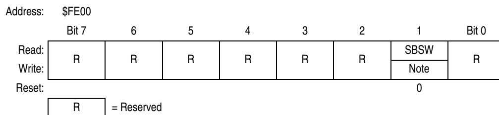
Figure 15-21. SIM Break Status Register (SBSR)
