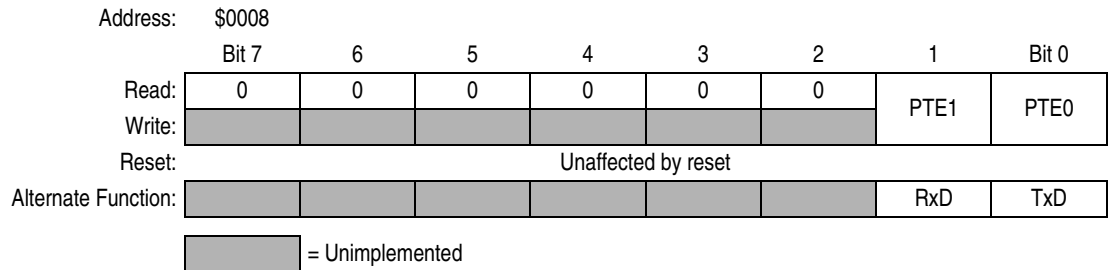
Figure 12-17. Port E Data Register (PTE)
