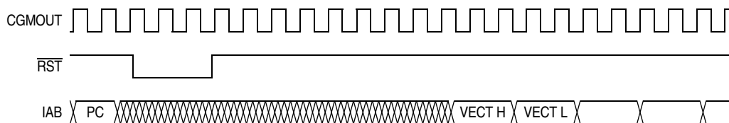
Figure 15-5. External Reset Timing
