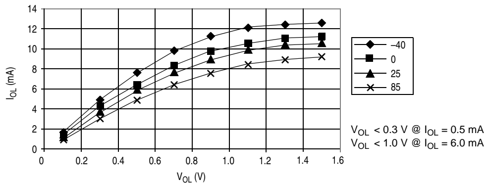
Figure 20-13. Typical Low-Side Driver Characteristics — Ports PTB7–PTB0, PTC6–PTC5, PTD7–PTD0, and PTE1–PTE0 ( V_{DD} = 2.7 Vdc)
