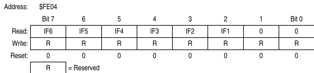
Figure 13-7. Interrupt Status Register 1 (INT1)
