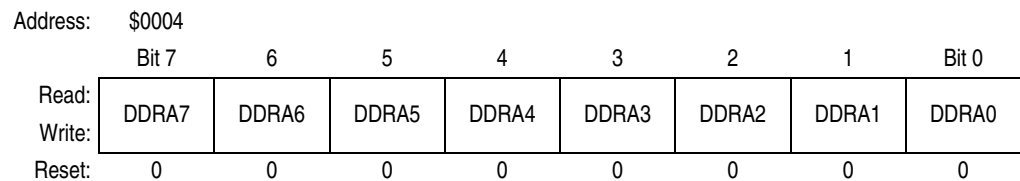
Figure 12-3. Data Direction Register A (DDRA)
