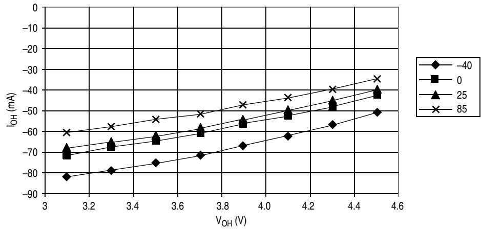
Figure 20-6. Typical High-Side Driver Characteristics — Ports PTB7–PTB0, PTC6–PTC5, PTD7–PTD0, and PTE1–PTE0 (V DD = 5.5 Vdc)
