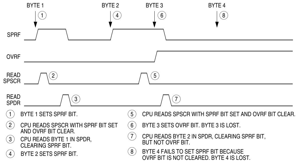
Figure 16-10. Missed Read of Overflow Condition
