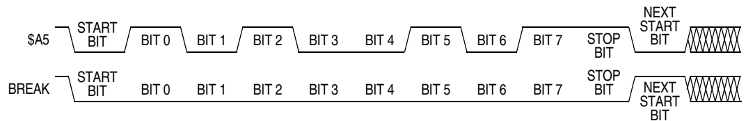
Figure 19-10. Sample Monitor Waveforms
