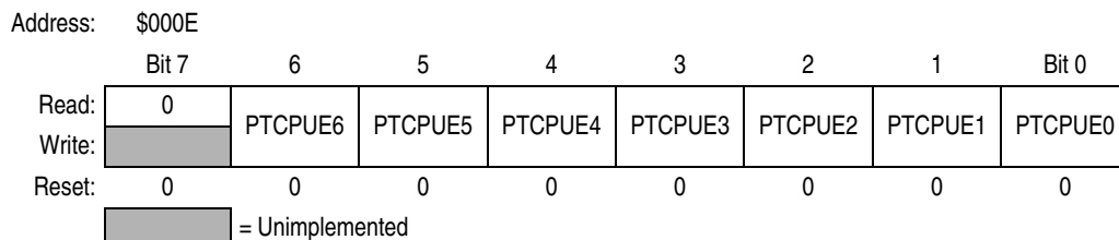
Figure 12-12. Port C Input Pullup Enable Register (PTCPUE)
