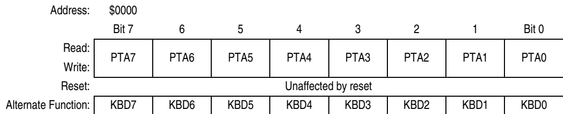
Figure 12-2. Port A Data Register (PTA)
