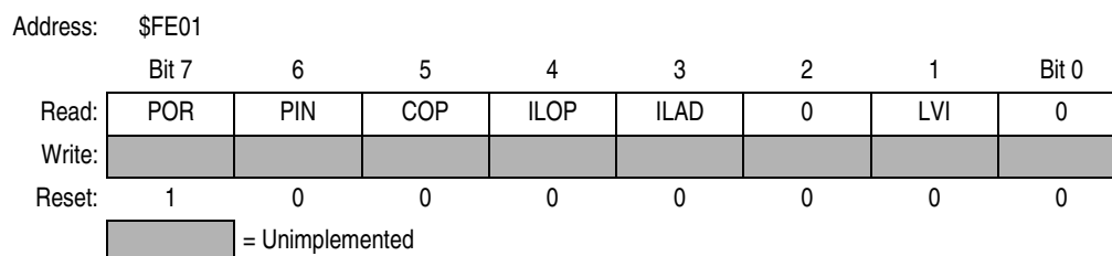
Figure 15-22. SIM Reset Status Register (SRSR)
