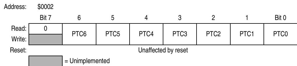
Figure 12-9. Port C Data Register (PTC)
