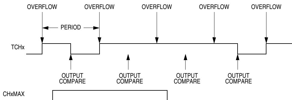
Figure 18-12. CHxMAX Latency
