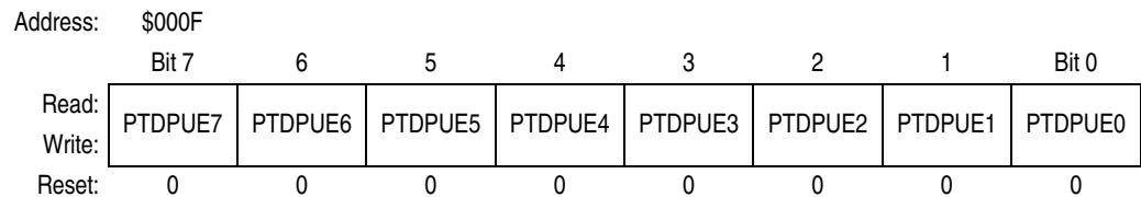
Figure 12-16. Port D Input Pullup Enable Register (PTDPUE)
