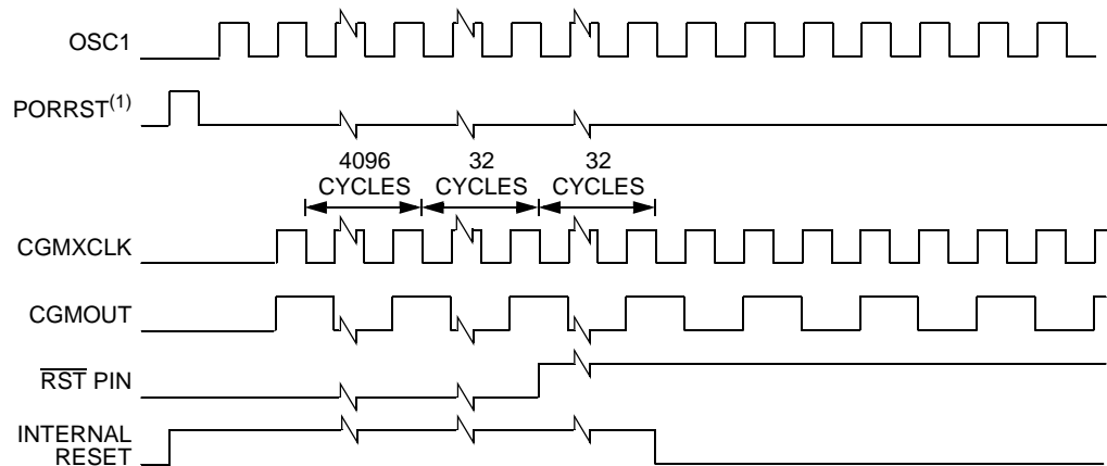
Figure 13-2. Power-On Reset Recovery
