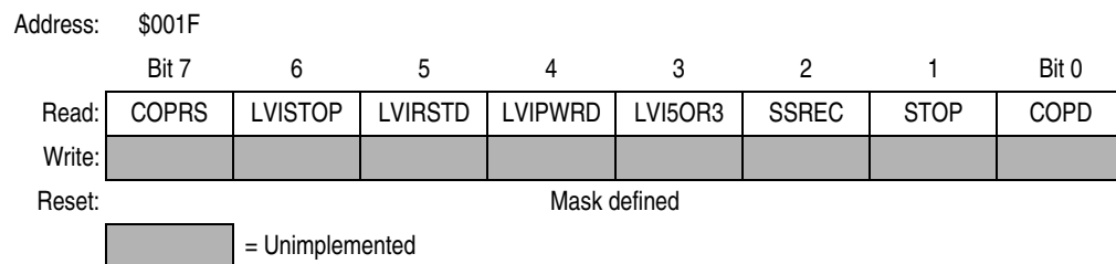
Figure 11-2. Mask Option Register 1 (MOR1)
