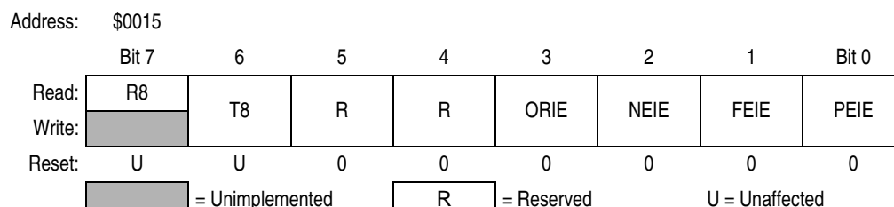
Figure 14-12. SCI Control Register 3 (SCC3)
