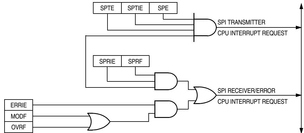
Figure 16-12. SPI Interrupt Request Generation
