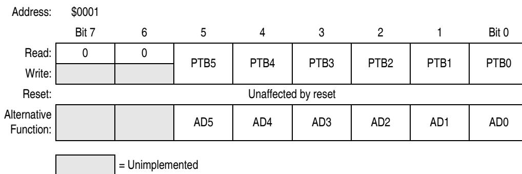
Figure 12-6. Port B Data Register (PTB)
