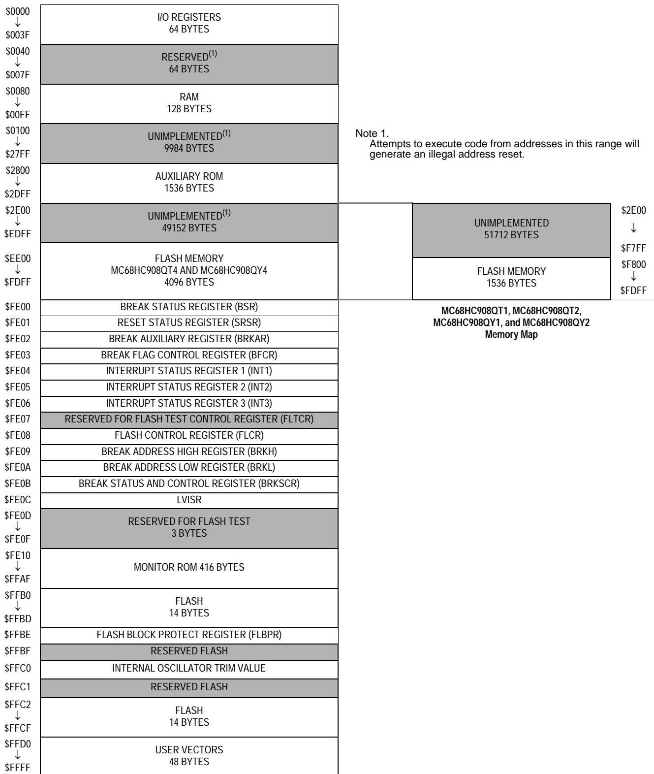
Figure 3. Memory Map
