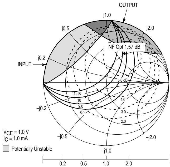
Figure 20. Constant Gain and Noise Figure Contours (f = 1.0 GHz)
