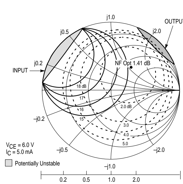
Figure 23. Constant Gain and Noise Figure Contours (f = 1.0 GHz)
