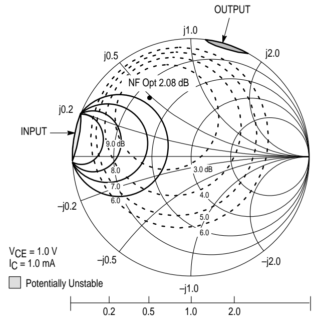
Figure 21. Constant Gain and Noise Figure Contours (f = 2.0 GHz)
