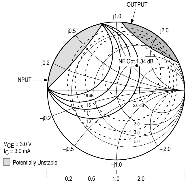
Figure 22. Constant Gain and Noise Figure Contours (f = 1.0 GHz)
