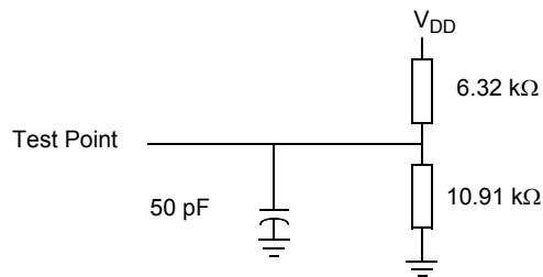
Figure 8. Control Timing Test Load for OUT and \overline{RST} Pins
