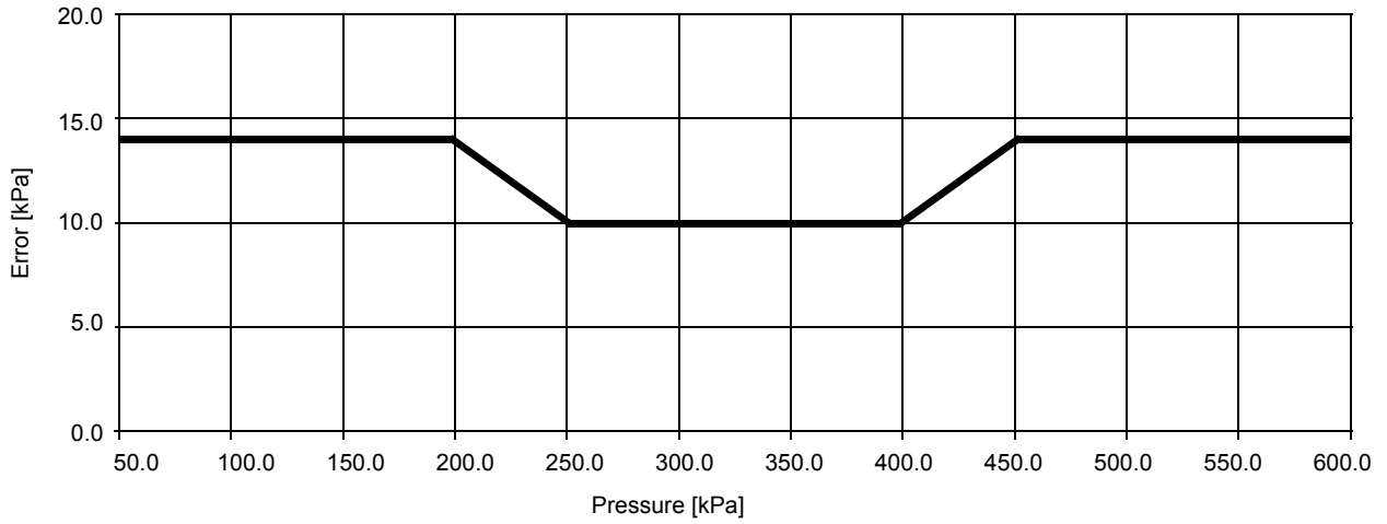
Figure 9. Pressure Error vs Pressure at T = 25^{\circ}\text{C} , 2.5\text{ V} \leq V_{\text{DD}} \leq 3.0\text{ V}
