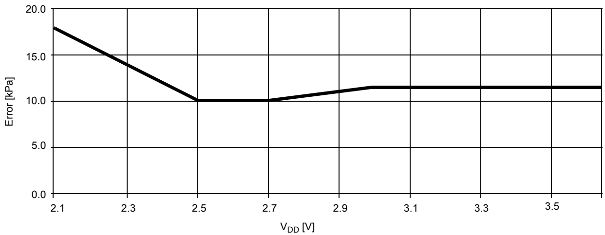
Figure 10. Pressure Error vs V_{\text{DD}} at T = 25^{\circ}\text{C} , 200\text{ kPa} \leq V_{\text{DD}} \leq 400\text{ kPa}
