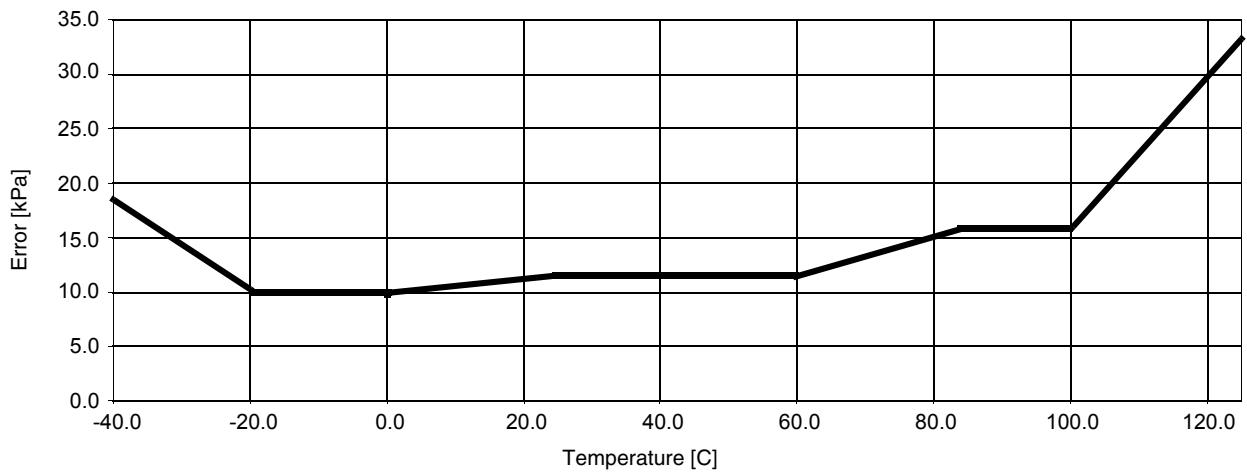
Figure 11. Pressure Error vs Temperature at V_{\text{DD}} = 3.0\text{ V} , 200\text{ kPa} \leq V_{\text{DD}} \leq 400\text{ kPa}
