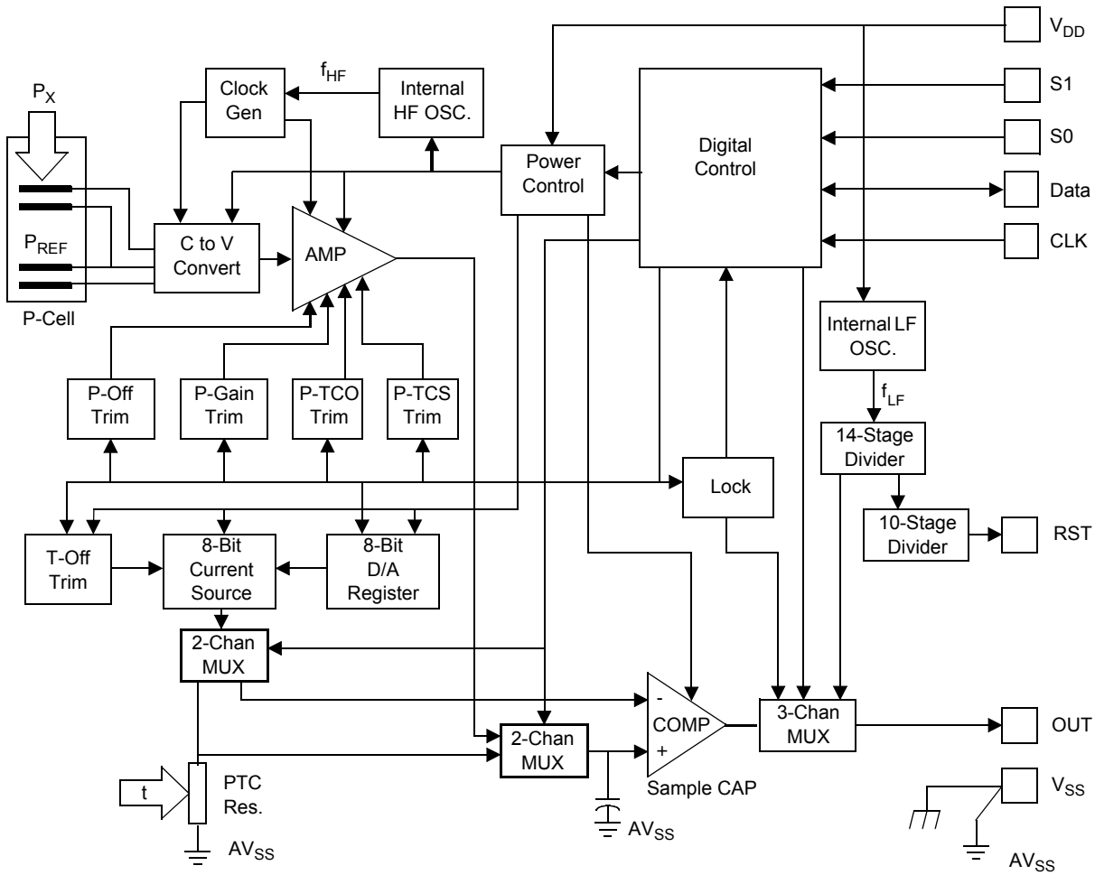
Figure 1. SPXY8011A Block Diagram
