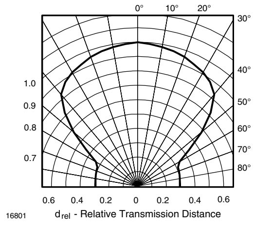
Fig. 12 - Directivity
